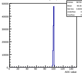
Pedestals mcm163-6A13-refv5-g0-s0-p1 ch 94 test1
