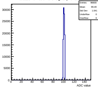
Pedestals mcm163-6A13-refv5-g0-s0-p1 ch 38 test1
