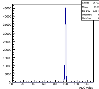
Pedestals mcm163-6A13-refv5-g0-s0-p1 ch 91 test1
