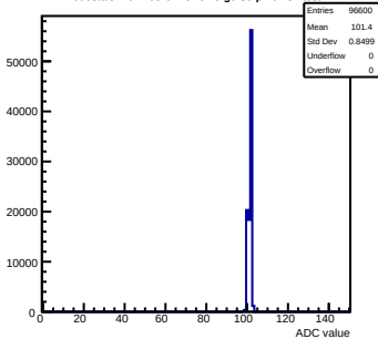
Pedestals mcm163-6A13-refv5-g0-s0-p1 ch 37 test1
