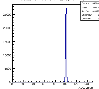
Pedestals mcm163-6A13-refv5-g0-s0-p1 ch 77 test1
