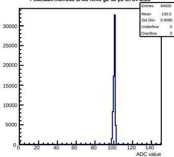
Pedestals mcm163-6A13-refv5-g0-s0-p1 ch 64 test1
