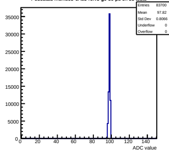
Pedestals mcm163-6A13-refV5-g0-s0-p1 ch 53 test1
