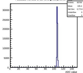
Pedestals mcm163-6A13-refV5-g0-s0-p1 ch 54 test1
