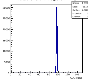
Pedestals mcm163-6A13-refv5-g0-s0-p1 ch 74 test1
