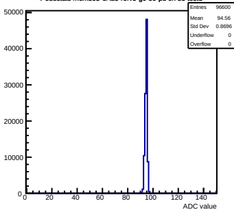
Pedestals mcm163-6A13-refv5-g0-s0-p1 ch 33 test1
