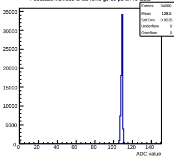
Pedestals mcm163-6A13-refv5-g0-s0-p1 ch 76 test1
