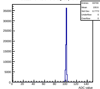
Pedestals mcm163-6A13-refV5-g0-s0-p1 ch 61 test1
