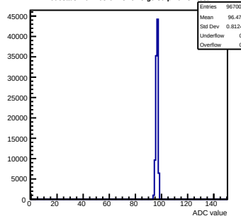
Pedestals mcm163-6A13-refv5-g0-s0-p1 ch 87 test1
