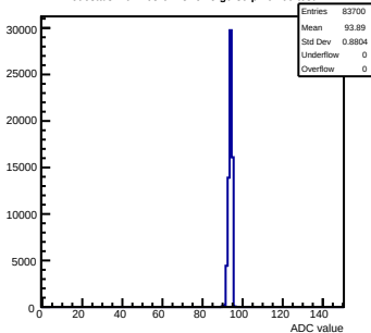
Pedestals mcm163-6A13-refV5-g0-s0-p1 ch 60 test1
