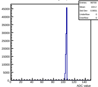
Pedestals mcm163-6A13-refv5-g0-s0-p1 ch 88 test1
