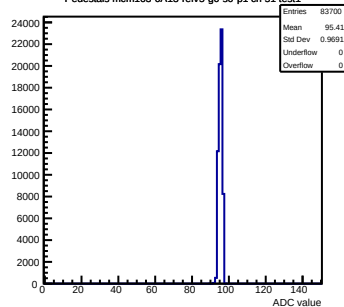
Pedestals mcm163-6A13-refV5-g0-s0-p1 ch 51 test1
