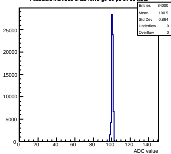
Pedestals mcm163-6A13-refv5-g0-s0-p1 ch 68 test1
