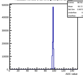
Pedestals mcm163-6A13-refv5-g0-s0-p1 ch 82 test1
