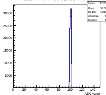
Pedestals mcm163-6A13-refv5-g0-s0-p1 ch 83 test1
