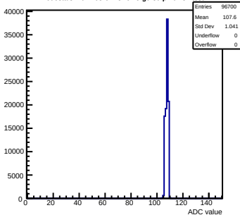
Pedestals mcm163-6A13-refv5-g0-s0-p1 ch 84 test1
