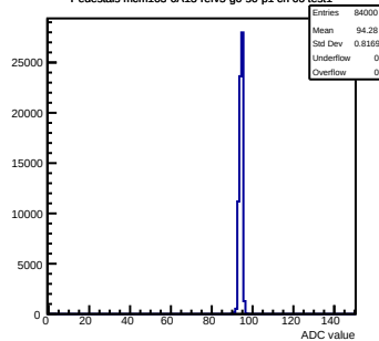
Pedestals mcm163-6A13-refv5-g0-s0-p1 ch 66 test1
