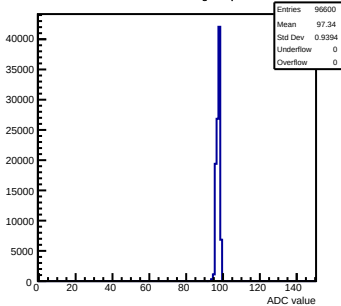
Pedestals mcm163-6A13-refv5-g0-s0-p1 ch 44 test1
