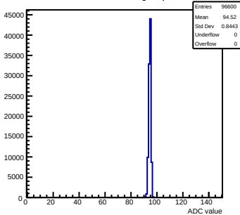
Pedestals mcm163-6A13-refv5-g0-s0-p1 ch 45 test1
