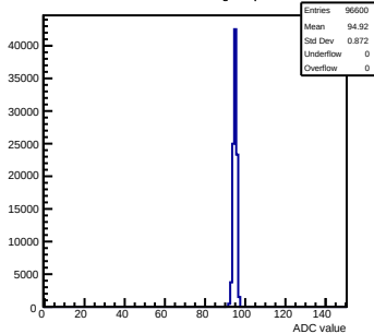
Pedestals mcm163-6A13-refv5-g0-s0-p1 ch 46 test1
