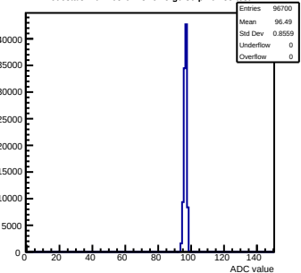
Pedestals mcm163-6A13-refv5-g0-s0-p1 ch 85 test1
