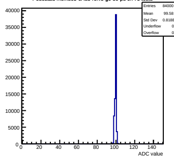
Pedestals mcm163-6A13-refv5-g0-s0-p1 ch 78 test1
