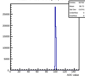
Pedestals mcm163-6A13-refV5-g0-s0-p1 ch 58 test1
