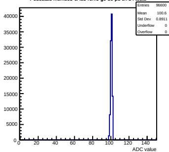
Pedestals mcm163-6A13-refv5-g0-s0-p1 ch 34 test1
