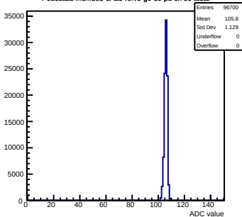
Pedestals mcm163-6A13-refv5-g0-s0-p1 ch 80 test1
