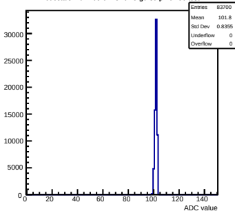
Pedestals mcm163-6A13-refV5-g0-s0-p1 ch 56 test1
