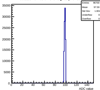
Pedestals mcm163-6A13-refv5-g0-s0-p1 ch 86 test1
