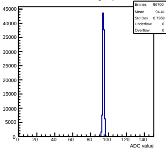
Pedestals mcm163-6A13-refv5-g0-s0-p1 ch 92 test1
