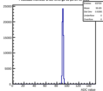
Pedestals mcm163-6A13-refV5-g0-s0-p1 ch 49 test1
