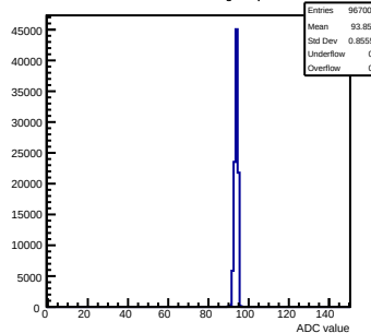
Pedestals mcm163-6A13-refv5-g0-s0-p1 ch 95 test1
