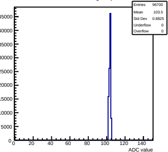
Pedestals mcm163-6A13-refv5-g0-s0-p1 ch 89 test1
