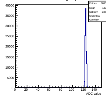
Pedestals mcm163-6A13-relv6-g0-s0-p1 ch 11 test1
