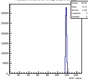
Pedestals mcm163-6A13-refv6-g0-s0-p1 ch 95 test1
