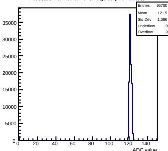
Pedestals mcm163-6A13-refv6-g0-s0-p1 ch 90 test1
