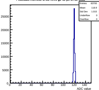
Pedestals mcm163-6A13-refv6-g0-s0-p1 ch 52 test1
