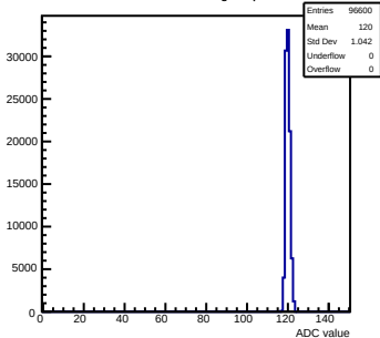
Pedestals mcm163-6A13-refv6-g0-s0-p1 ch 104 test1
