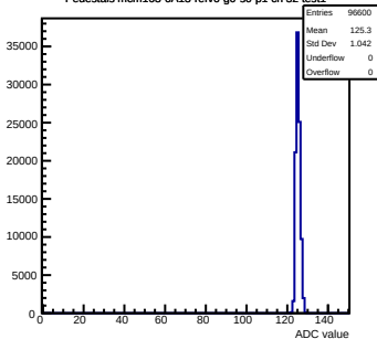
Pedestals mcm163-6A13-refv6-g0-s0-p1 ch 32 test1
