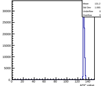
Pedestals mcm163-6A13-refv6-g0-s0-p1 ch 118 test1
