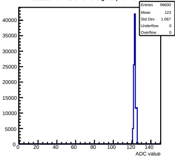
Pedestals mcm163-6A13-refv6-g0-s0-p1 ch 101 test1
