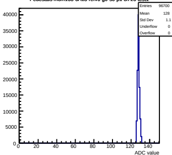
Pedestals mcm163-6A13-refv6-g0-s0-p1 ch 20 test1
