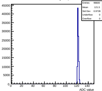
Pedestals mcm163-6A13-refv6-g0-s0-p1 ch 108 test1
