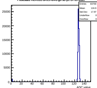
Pedestals mcm163-6A13-refv6-g0-s0-p1 ch 63 test1
