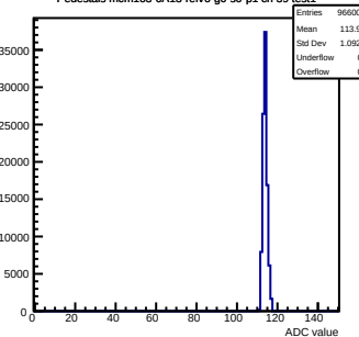
Pedestals mcm163-6A13-refv6-g0-s0-p1 ch 39 test1
