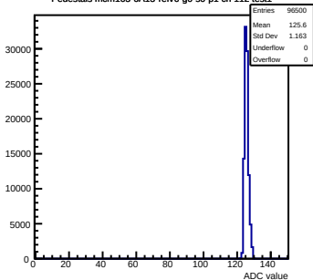
Pedestals mcm163-6A13-refv6-g0-s0-p1 ch 112 test1
