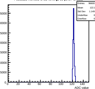
Pedestals mcm163-6A13-refv6-g0-s0-p1 ch 42 test1
