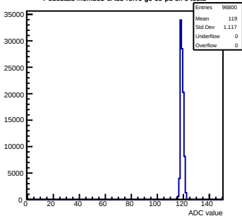
Pedestals mcm163-6A13-relv6-g0-s0-p1 ch 0 test1
