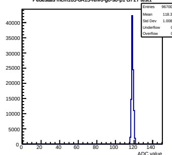
Pedestals mcm163-6A13-refv6-g0-s0-p1 ch 27 test1
