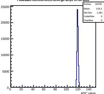
Pedestals mcm163-6A13-refv6-g0-s0-p1 ch 60 test1
