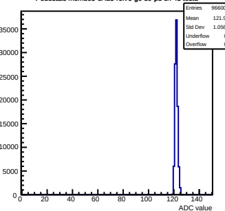
Pedestals mcm163-6A13-refv6-g0-s0-p1 ch 43 test1
