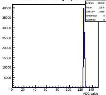
Pedestals mcm163-6A13-refv6-g0-s0-p1 ch 102 test1
