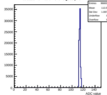
Pedestals mcm163-6A13-relv6-g0-s0-p1 ch 14 test1
