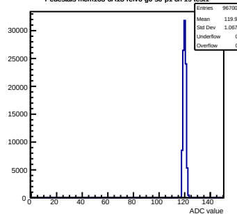
Pedestals mcm163-6A13-refv6-g0-s0-p1 ch 19 test1
