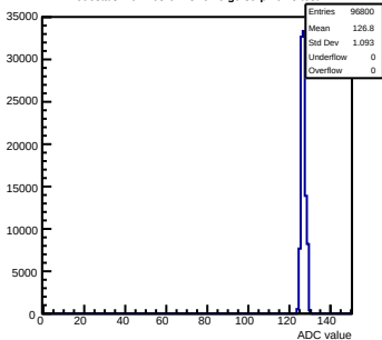
Pedestals mcm163-6A13-relv6-g0-s0-p1 ch 8 test1
