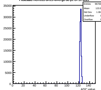
Pedestals mcm163-6A13-refv6-g0-s0-p1 ch 31 test1
