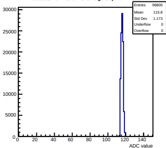
Pedestals mcm163-6A13-relv6-g0-s0-p1 ch 12 test1
