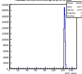
Pedestals mcm163-6A13-refv6-g0-s0-p1 ch 59 test1
