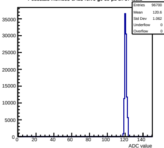
Pedestals mcm163-6A13-refv6-g0-s0-p1 ch 87 test1
