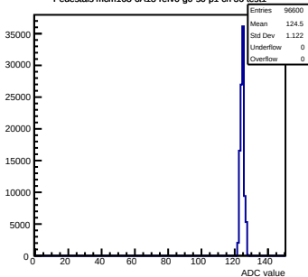
Pedestals mcm163-6A13-refv6-g0-s0-p1 ch 36 test1
