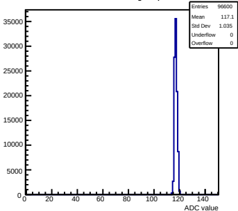
Pedestals mcm163-6A13-refv6-g0-s0-p1 ch 105 test1
