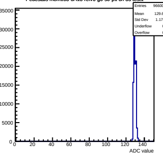
Pedestals mcm163-6A13-refv6-g0-s0-p1 ch 35 test1
