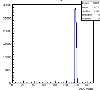
Pedestals mcm163-6A13-relv6-g0-s0-p1 ch 13 test1
