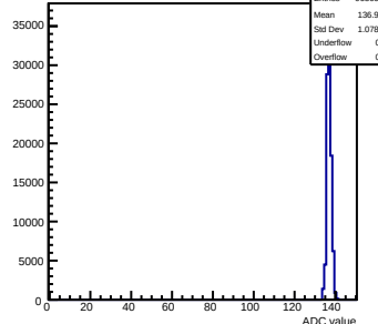
Pedestals mcm163-6A13-refv6-g0-s0-p1 ch 127 test1
