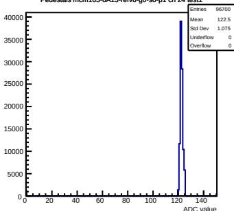
Pedestals mcm163-6A13-refv6-g0-s0-p1 ch 24 test1
