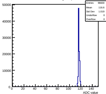
Pedestals mcm163-6A13-refv6-g0-s0-p1 ch 110 test1
