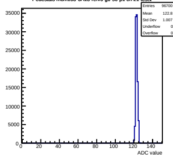
Pedestals mcm163-6A13-refv6-g0-s0-p1 ch 21 test1
