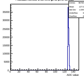
Pedestals mcm163-6A13-refv6-g0-s0-p1 ch 18 test1
