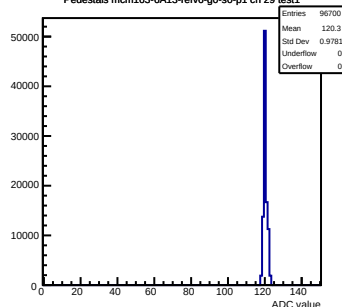
Pedestals mcm163-6A13-refv6-g0-s0-p1 ch 29 test1
