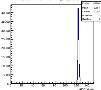
Pedestals mcm163-6A13-refv6-g0-s0-p1 ch 91 test1
