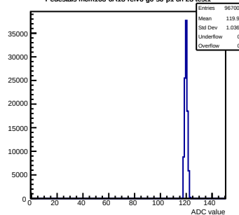
Pedestals mcm163-6A13-refv6-g0-s0-p1 ch 23 test1
