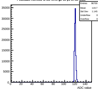
Pedestals mcm163-6A13-refv6-g0-s0-p1 ch 82 test1
