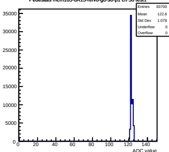
Pedestals mcm163-6A13-refv6-g0-s0-p1 ch 58 test1
