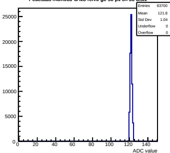
Pedestals mcm163-6A13-refv6-g0-s0-p1 ch 53 test1
