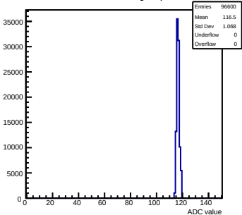
Pedestals mcm163-6A13-refv6-g0-s0-p1 ch 111 test1
