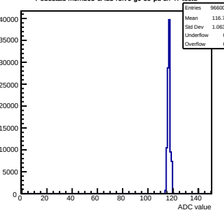
Pedestals mcm163-6A13-refv6-g0-s0-p1 ch 47 test1
