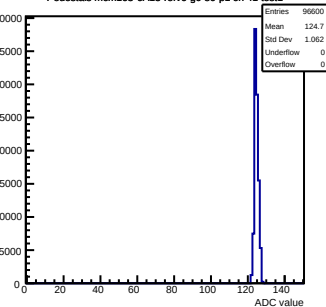
Pedestals mcm163-6A13-refv6-g0-s0-p1 ch 41 test1
