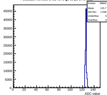
Pedestals mcm163-6A13-relv6-g0-s0-p1 ch 1 test1
