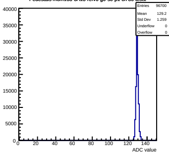
Pedestals mcm163-6A13-refv6-g0-s0-p1 ch 80 test1
