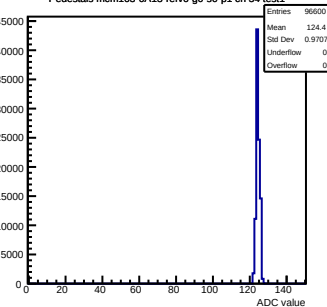
Pedestals mcm163-6A13-refv6-g0-s0-p1 ch 34 test1
