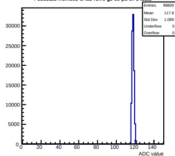
Pedestals mcm163-6A13-relv6-g0-s0-p1 ch 5 test1
