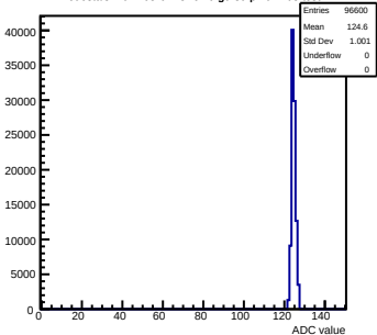
Pedestals mcm163-6A13-refv6-g0-s0-p1 ch 103 test1
