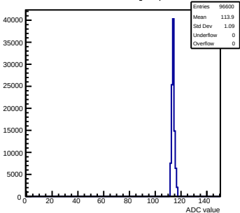
Pedestals mcm163-6A13-refv6-g0-s0-p1 ch 107 test1
