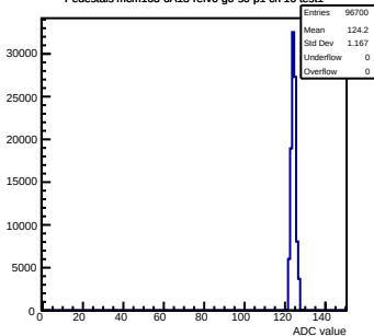
Pedestals mcm163-6A13-refv6-g0-s0-p1 ch 16 test1
