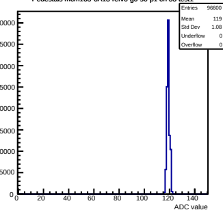
Pedestals mcm163-6A13-refv6-g0-s0-p1 ch 33 test1
