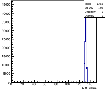
Pedestals mcm163-6A13-refv6-g0-s0-p1 ch 116 test1
