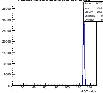
Pedestals mcm163-6A13-refV0-g0-s0-p1 ch 18 test1
