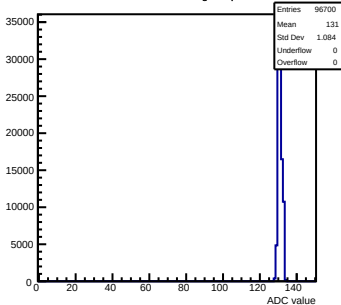
Pedestals mcm163-6A13-refV0-g0-s0-p1 ch 88 test1
