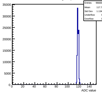
Pedestals mcm163-6A13-refV0-g0-s0-p1 ch 47 test1
