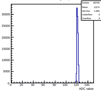
Pedestals mcm163-6A13-refV0-g0-s0-p1 ch 92 test1
