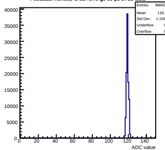
Pedestals mcm163-6A13-refV0-g0-s0-p1 ch 33 test1
