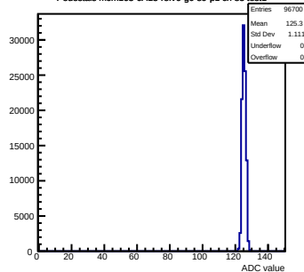
Pedestals mcm163-6A13-refV0-g0-s0-p1 ch 83 test1
