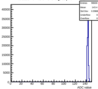
Pedestals mcm163-6A13-rev0-g0-s0-p1 ch 121 test1
