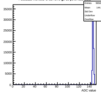
Pedestals mcm163-6A13-rev0-g0-s0-p1 ch 119 test1
