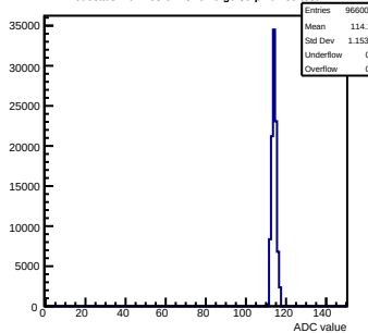
Pedestals mcm163-6A13-refV0-g0-s0-p1 ch 39 test1
