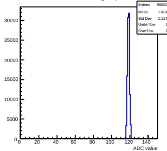
Pedestals mcm163-6A13-refV0-g0-s0-p1 ch 45 test1
