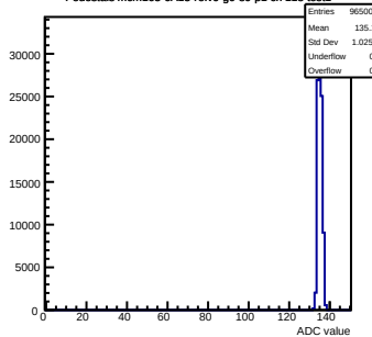
Pedestals mcm163-6A13-rev0-g0-s0-p1 ch 118 test1
