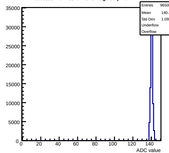
Pedestals mcm163-6A13-rev0-g0-s0-p1 ch 127 test1
