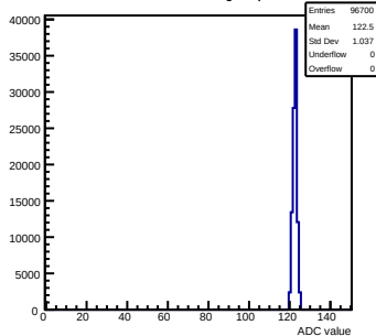
Pedestals mcm163-6A13-refV0-g0-s0-p1 ch 94 test1
