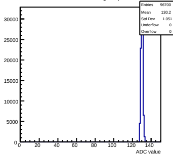
Pedestals mcm163-6A13-refV0-g0-s0-p1 ch 93 test1
