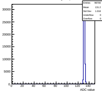
Pedestals mcm163-6A13-refV0-g0-s0-p1 ch 89 test1
