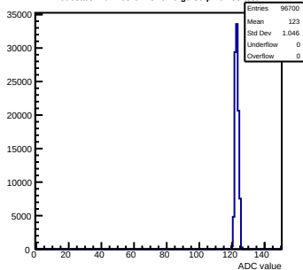
Pedestals mcm163-6A13-refV0-g0-s0-p1 ch 85 test1
