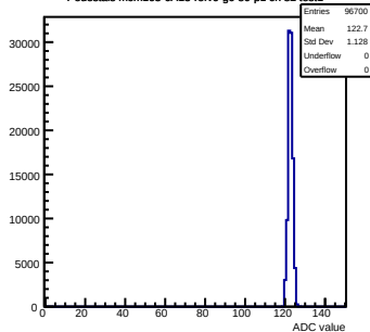
Pedestals mcm163-6A13-refV0-g0-s0-p1 ch 82 test1
