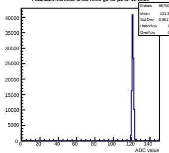
Pedestals mcm163-6A13-refV0-g0-s0-p1 ch 19 test1
