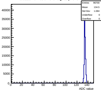
Pedestals mcm163-6A13-refV0-g0-s0-p1 ch 84 test1
