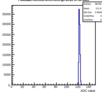
Pedestals mcm163-6A13-refV0-g0-s0-p1 ch 30 test1
