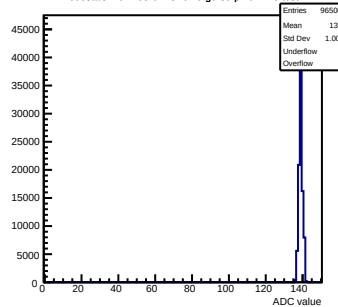
Pedestals mcm163-6A13-rev0-g0-s0-p1 ch 123 test1
