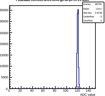
Pedestals mcm163-6A13-refV0-g0-s0-p1 ch 29 test1
