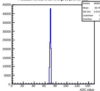
Pedestals mcm163-6A13-refV2-g0-s0-p1 ch 10 test1
