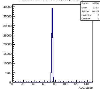
Pedestals mcm163-6A13-refV2-g0-s0-p1 ch 8 test1
