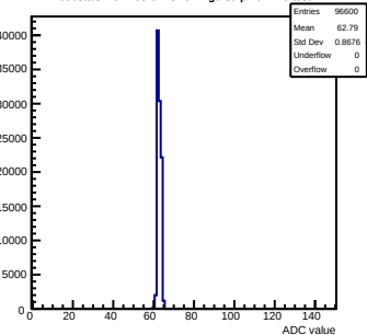
Pedestals mcm163-6A13-refv2-g0-s0-p1 ch 110 test1
