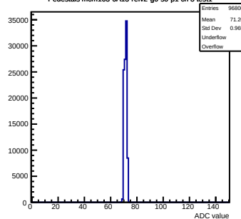
Pedestals mcm163-6A13-refV2-g0-s0-p1 ch 3 test1
