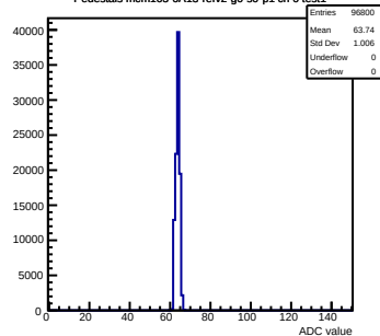
Pedestals mcm163-6A13-refV2-g0-s0-p1 ch 0 test1
