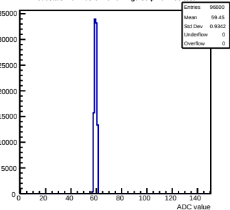
Pedestals mcm163-6A13-refv2-g0-s0-p1 ch 109 test1
