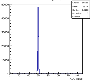
Pedestals mcm163-6A13-refv2-g0-s0-p1 ch 107 test1
