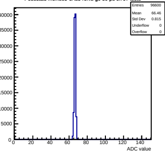
Pedestals mcm163-6A13-refv2-g0-s0-p1 ch 97 test1
