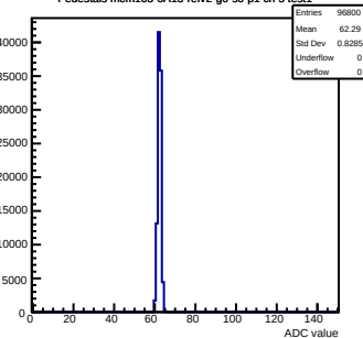
Pedestals mcm163-6A13-refV2-g0-s0-p1 ch 5 test1
