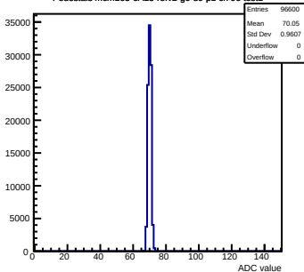
Pedestals mcm163-6A13-refv2-g0-s0-p1 ch 96 test1
