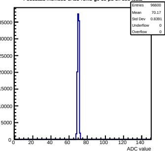
Pedestals mcm163-6A13-refv2-g0-s0-p1 ch 101 test1
