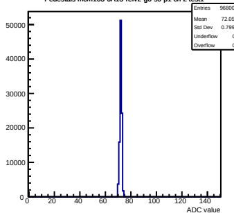
Pedestals mcm163-6A13-refV2-g0-s0-p1 ch 2 test1
