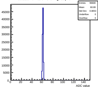
Pedestals mcm163-6A13-refv2-g0-s0-p1 ch 111 test1
