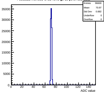
Pedestals mcm163-6A13-refv2-g0-s0-p1 ch 103 test1
