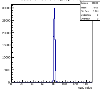
Pedestals mcm163-6A13-refV5-g0-s0-p1 ch 0 test1
