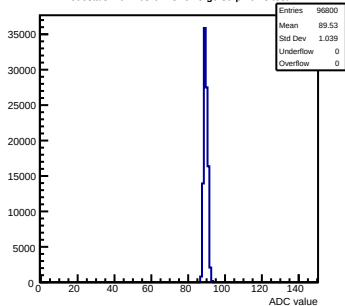
Pedestals mcm163-6A13-refV5-g0-s0-p1 ch 8 test1
