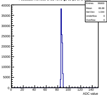
Pedestals mcm163-6A13-refV5-g0-s0-p1 ch 3 test1
