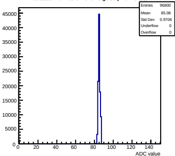
Pedestals mcm163-6A13-refV5-g0-s0-p1 ch 15 test1
