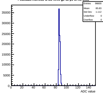
Pedestals mcm163-6A13-refv5-g0-s0-p1 ch 96 test1
