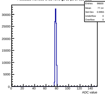
Pedestals mcm163-6A13-refv5-g0-s0-p1 ch 105 test1
