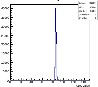
Pedestals mcm163-6A13-refV5-g0-s0-p1 ch 11 test1
