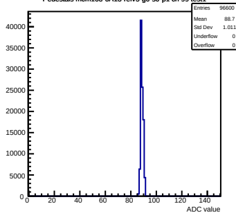
Pedestals mcm163-6A13-refv5-g0-s0-p1 ch 99 test1
