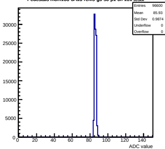
Pedestals mcm163-6A13-refv5-g0-s0-p1 ch 101 test1
