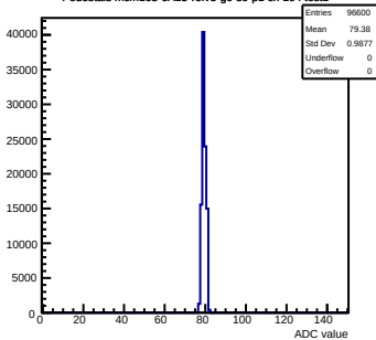
Pedestals mcm163-6A13-refv5-g0-s0-p1 ch 104 test1
