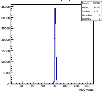
Pedestals mcm163-6A13-refV5-g0-s0-p1 ch 9 test1
