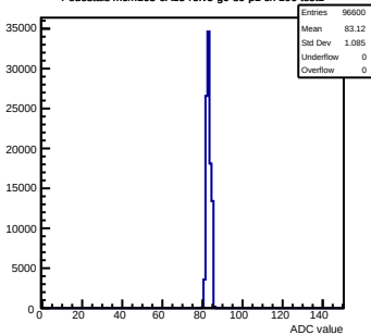
Pedestals mcm163-6A13-refv5-g0-s0-p1 ch 106 test1
