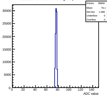
Pedestals mcm163-6A13-refV5-g0-s0-p1 ch 12 test1
