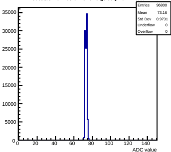
Pedestals mcm163-6A13-refV5-g0-s0-p1 ch 14 test1
