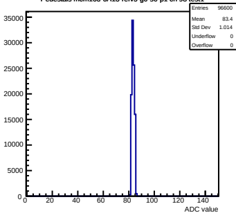
Pedestals mcm163-6A13-refv5-g0-s0-p1 ch 98 test1
