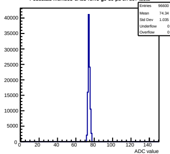
Pedestals mcm163-6A13-refv5-g0-s0-p1 ch 107 test1
