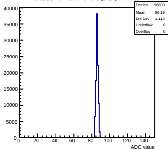
Pedestals mcm163-6A13-refV5-g0-s0-p1 ch 4 test1
