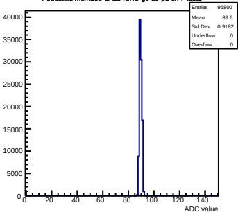
Pedestals mcm163-6A13-refV5-g0-s0-p1 ch 7 test1
