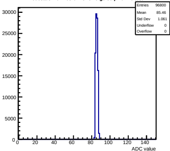
Pedestals mcm163-6A13-refV5-g0-s0-p1 ch 10 test1
