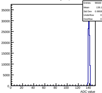
Pedestals mcm163-6A13-refV6-g0-s0-p1 ch 127 test1
