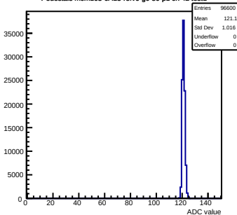
Pedestals mcm163-6A13-refv6-g0-s0-p1 ch 42 test1
