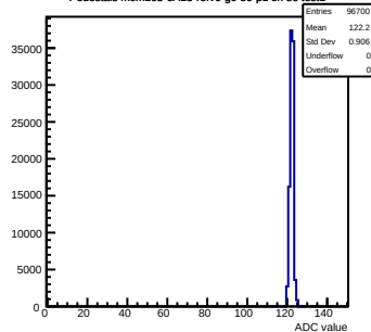
Pedestals mcm163-6A13-refv6-g0-s0-p1 ch 86 test1
