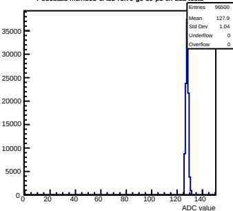
Pedestals mcm163-6A13-refV6-g0-s0-p1 ch 112 test1
