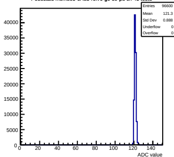
Pedestals mcm163-6A13-refv6-g0-s0-p1 ch 43 test1
