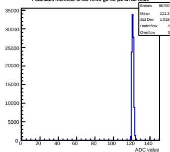
Pedestals mcm163-6A13-refv6-g0-s0-p1 ch 82 test1
