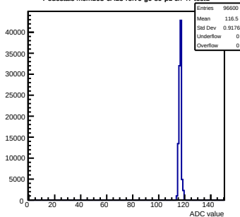
Pedestals mcm163-6A13-refv6-g0-s0-p1 ch 47 test1
