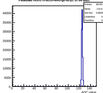
Pedestals mcm170-6010-refv0-g0-s0-p1 ch 89 test1
