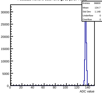
Pedestals mcm170-6010-refV0-g0-s0-p1 ch 0 test1
