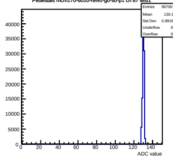
Pedestals mcm170-6010-refv0-g0-s0-p1 ch 87 test1
