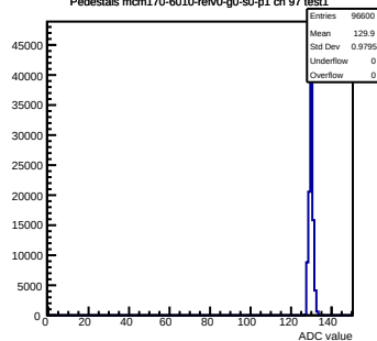
Pedestals mcm170-6010-refV0-g0-s0-p1 ch 97 test1
