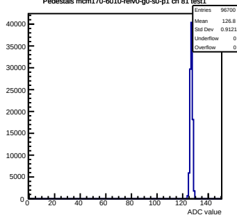
Pedestals mcm170-6010-refv0-g0-s0-p1 ch 81 test1
