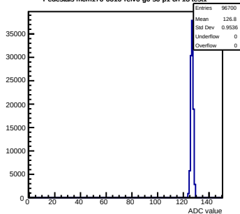
Pedestals mcm170-6010-rev0-g0-s0-p1 ch 18 test1
