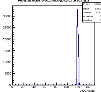
Pedestals mcm170-6010-refV0-g0-s0-p1 ch 103 test1
