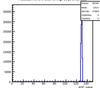
Pedestals mcm170-6010-rev0-g0-s0-p1 ch 25 test1
