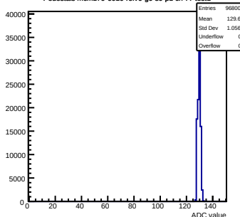
Pedestals mcm170-6010-refv0-g0-s0-p1 ch 77 test1
