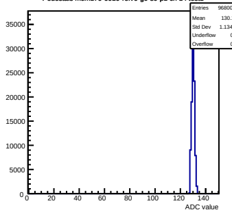
Pedestals mcm170-6010-refV0-g0-s0-p1 ch 14 test1
