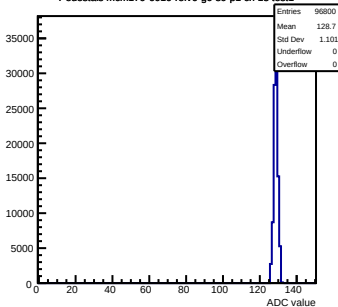
Pedestals mcm170-6010-refV0-g0-s0-p1 ch 13 test1
