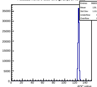
Pedestals mcm170-6010-refv0-g0-s0-p1 ch 73 test1
