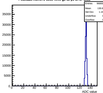
Pedestals mcm170-6010-refv0-g0-s0-p1 ch 67 test1
