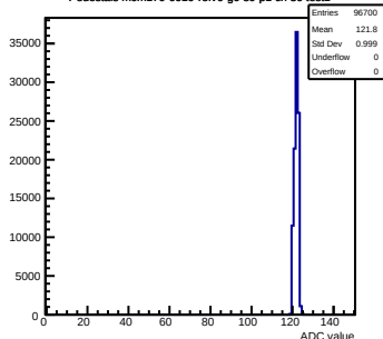
Pedestals mcm170-6010-rev0-g0-s0-p1 ch 30 test1
