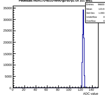
Pedestals mcm170-6010-refV0-g0-s0-p1 ch 101 test1
