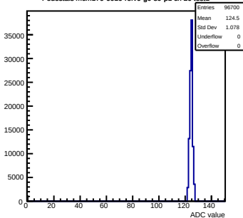
Pedestals mcm170-6010-rev0-g0-s0-p1 ch 20 test1
