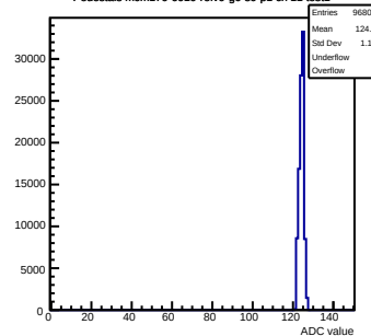
Pedestals mcm170-6010-refV0-g0-s0-p1 ch 11 test1
