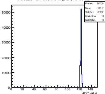
Pedestals mcm170-6010-rev0-g0-s0-p1 ch 24 test1
