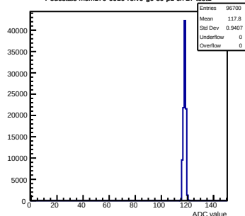
Pedestals mcm170-6010-rev0-g0-s0-p1 ch 27 test1
