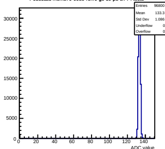
Pedestals mcm170-6010-refv0-g0-s0-p1 ch 74 test1
