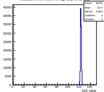
Pedestals mcm170-6010-rev0-g0-s0-p1 ch 23 test1
