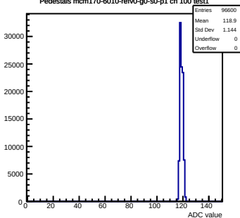
Pedestals mcm170-6010-refV0-g0-s0-p1 ch 100 test1
