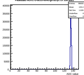
Pedestals mcm170-6010-refV0-g0-s0-p1 ch 106 test1
