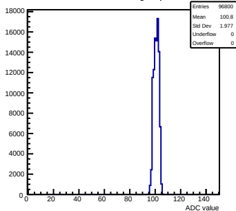
Pedestals mcm170-6010-refv1-g0-s0-p1 ch 14 test1
