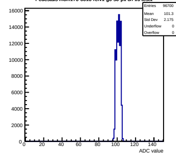
Pedestals mcm170-6010-rlv1-g0-s0-p1 ch 16 test1
