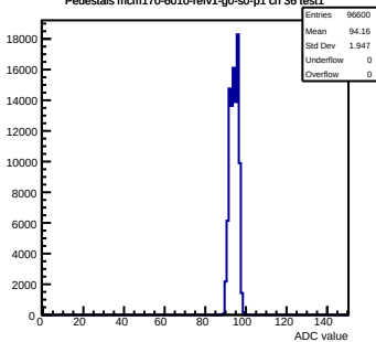
Pedestals mcm170-6010-rv1-g0-s0-p1 ch 36 test1
