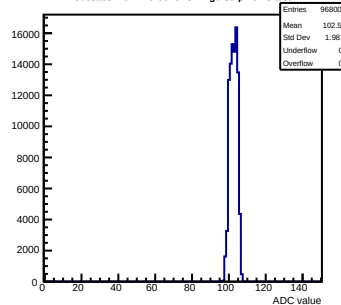
Pedestals mcm170-6010-refv1-g0-s0-p1 ch 3 test1
