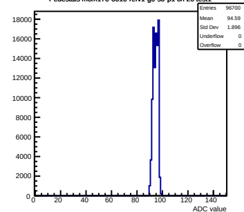
Pedestals mcm170-6010-rlv1-g0-s0-p1 ch 20 test1
