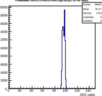
Pedestals mcm170-6010-rv1-g0-s0-p1 ch 42 test1
