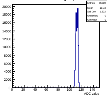
Pedestals mcm170-6010-refv1-g0-s0-p1 ch 2 test1
