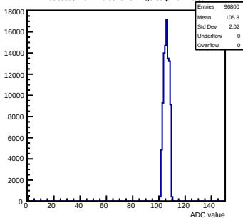
Pedestals mcm170-6010-refv1-g0-s0-p1 ch 4 test1
