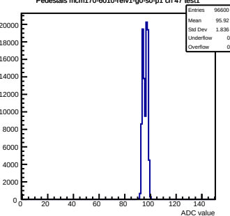
Pedestals mcm170-6010-rv1-g0-s0-p1 ch 47 test1
