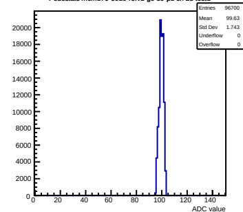
Pedestals mcm170-6010-rlv1-g0-s0-p1 ch 28 test1
