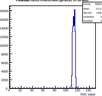
Pedestals mcm170-6010-rv1-g0-s0-p1 ch 39 test1
