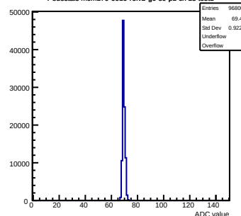
Pedestals mcm170-6010-ref2-g0-s0-p1 ch 15 test1
