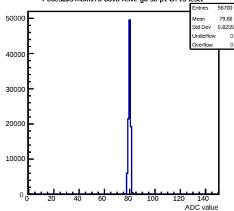
Pedestals mcm170-6010-refv2-g0-s0-p1 ch 19 test1
