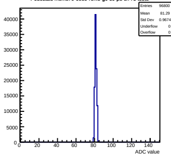
Pedestals mcm170-6010-refv2-g0-s0-p1 ch 75 test1
