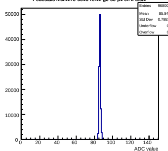
Pedestals mcm170-6010-ref2-g0-s0-p1 ch 2 test1
