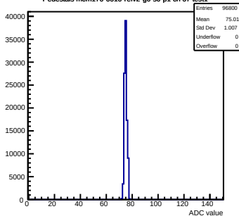
Pedestals mcm170-6010-refv2-g0-s0-p1 ch 67 test1
