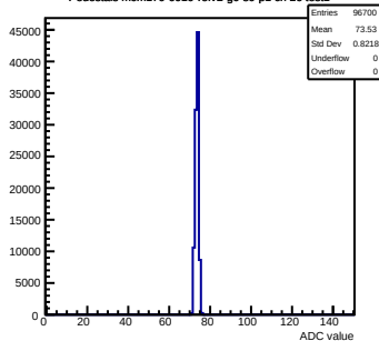
Pedestals mcm170-6010-refv2-g0-s0-p1 ch 26 test1
