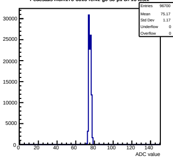
Pedestals mcm170-6010-refv2-g0-s0-p1 ch 16 test1
