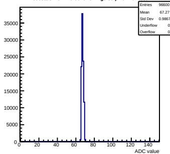
Pedestals mcm170-6010-refv2-g0-s0-p1 ch 101 test1
