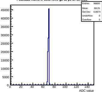
Pedestals mcm170-6010-refv2-g0-s0-p1 ch 65 test1
