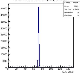
Pedestals mcm170-6010-refv2-g0-s0-p1 ch 73 test1
