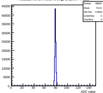
Pedestals mcm170-6010-refv2-g0-s0-p1 ch 74 test1
