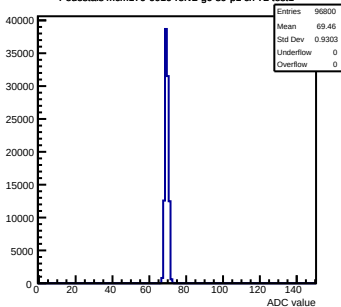
Pedestals mcm170-6010-refv2-g0-s0-p1 ch 72 test1
