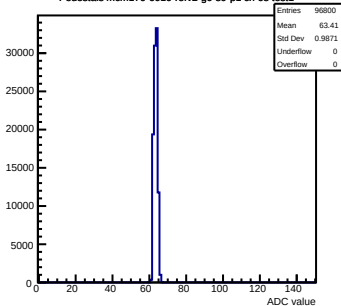
Pedestals mcm170-6010-refv2-g0-s0-p1 ch 68 test1
