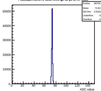
Pedestals mcm170-6010-refv2-g0-s0-p1 ch 17 test1
