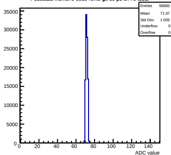
Pedestals mcm170-6010-refv2-g0-s0-p1 ch 79 test1
