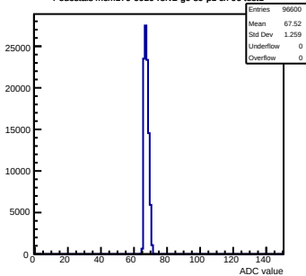
Pedestals mcm170-6010-refv2-g0-s0-p1 ch 96 test1
