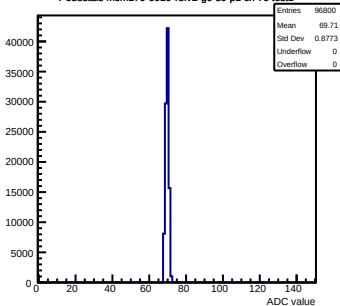
Pedestals mcm170-6010-refv2-g0-s0-p1 ch 70 test1
