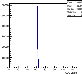
Pedestals mcm170-6010-refv2-g0-s0-p1 ch 109 test1
