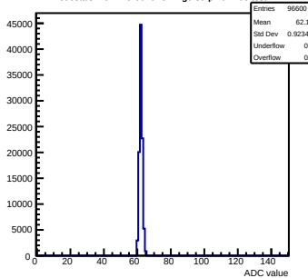
Pedestals mcm170-6010-refv2-g0-s0-p1 ch 103 test1
