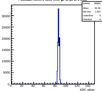
Pedestals mcm170-6010-ref2-g0-s0-p1 ch 0 test1
