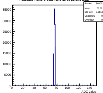
Pedestals mcm170-6010-ref2-g0-s0-p1 ch 1 test1
