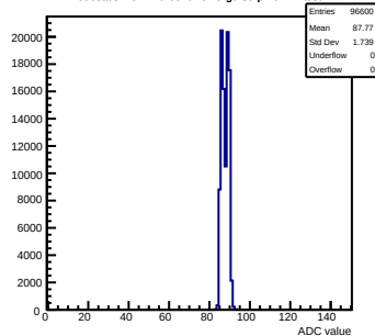
Pedestals mcm170-6010-rvf5-g0-s0-p1 ch 47 test1
