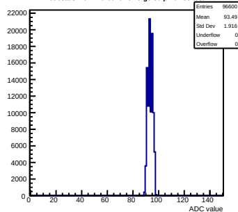
Pedestals mcm170-6010-rvf5-g0-s0-p1 ch 38 test1
