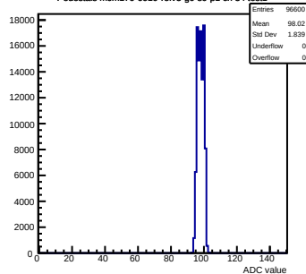
Pedestals mcm170-6010-rvf5-g0-s0-p1 ch 34 test1
