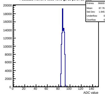
Pedestals mcm170-6010-rvf5-g0-s0-p1 ch 35 test1
