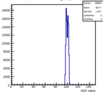
Pedestals mcm170-6010-rvf5-g0-s0-p1 ch 40 test1
