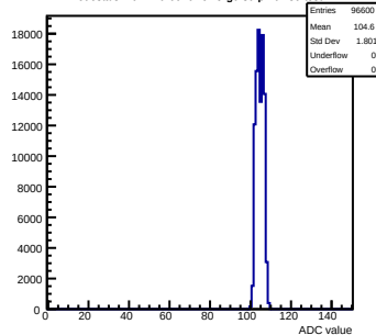
Pedestals mcm170-6010-rvf5-g0-s0-p1 ch 39 test1
