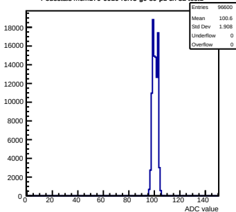
Pedestals mcm170-6010-rvf5-g0-s0-p1 ch 32 test1
