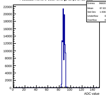
Pedestals mcm170-6010-rvf5-g0-s0-p1 ch 33 test1
