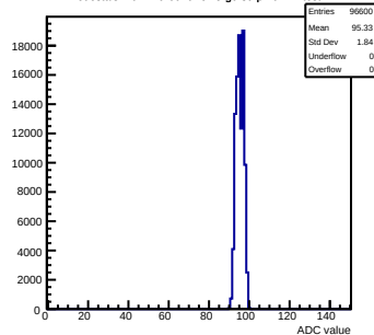
Pedestals mcm170-6010-rvf5-g0-s0-p1 ch 41 test1
