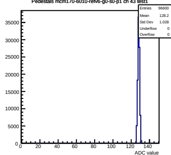
Pedestals mcm170-6010-rtv6-g0-s0-p1 ch 43 test1
