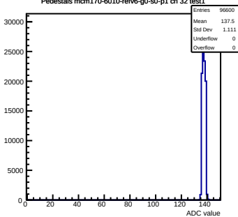
Pedestals mcm170-6010-rtv6-g0-s0-p1 ch 32 test1
