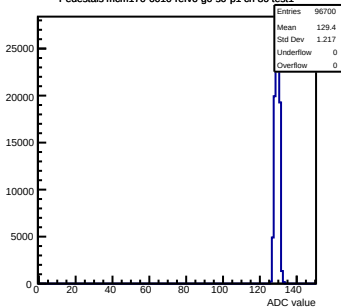
Pedestals mcm170-6010-relv6-g0-s0-p1 ch 80 test1
