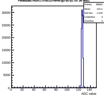
Pedestals mcm170-6010-rtv6-g0-s0-p1 ch 36 test1
