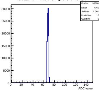
Pedestals mcm170-6010-refv2-g0-s0-p1 ch 107 test1
