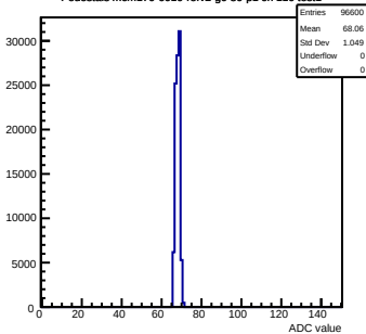
Pedestals mcm170-6010-refv2-g0-s0-p1 ch 110 test1
