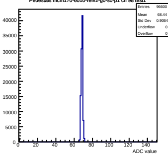
Pedestals mcm170-6010-refv2-g0-s0-p1 ch 98 test1
