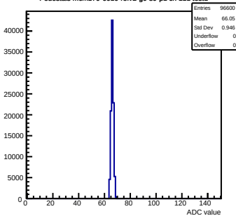
Pedestals mcm170-6010-refv2-g0-s0-p1 ch 111 test1
