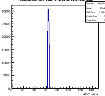
Pedestals mcm170-6010-refv2-g0-s0-p1 ch 103 test1
