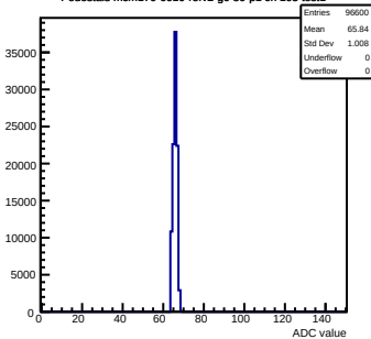
Pedestals mcm170-6010-refv2-g0-s0-p1 ch 105 test1
