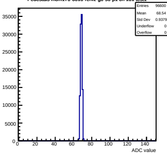
Pedestals mcm170-6010-refv2-g0-s0-p1 ch 101 test1
