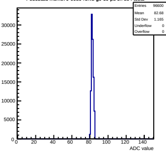
Pedestals mcm170-6010-refv2-g0-s0-p1 ch 104 test1
