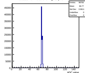
Pedestals mcm170-6010-refv2-g0-s0-p1 ch 24 test1
