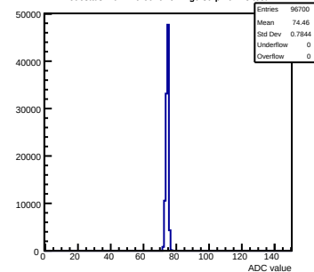
Pedestals mcm170-6010-refv2-g0-s0-p1 ch 28 test1
