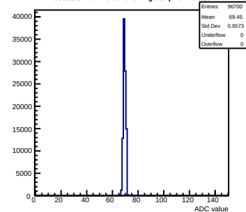
Pedestals mcm170-6010-refv2-g0-s0-p1 ch 20 test1
