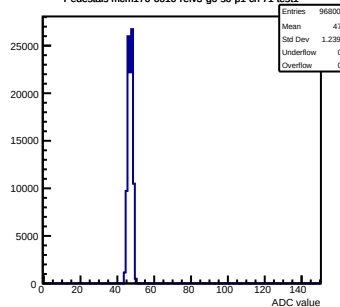
Pedestals mcm170-6010-refv3-g0-s0-p1 ch 71 test1
