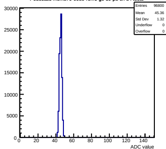
Pedestals mcm170-6010-refv3-g0-s0-p1 ch 14 test1
