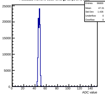
Pedestals mcm170-6010-refv3-g0-s0-p1 ch 3 test1
