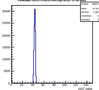
Pedestals mcm170-6010-refv3-g0-s0-p1 ch 66 test1
