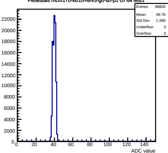
Pedestals mcm170-6010-refv3-g0-s0-p1 ch 64 test1
