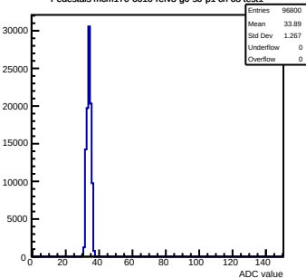
Pedestals mcm170-6010-refv3-g0-s0-p1 ch 68 test1
