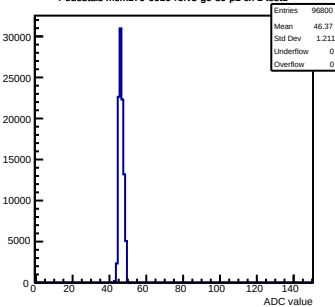
Pedestals mcm170-6010-refv3-g0-s0-p1 ch 1 test1
