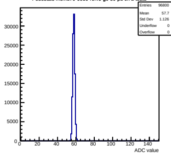
Pedestals mcm170-6010-refv3-g0-s0-p1 ch 2 test1
