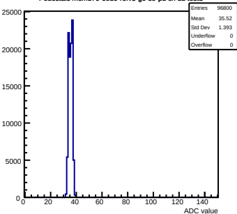
Pedestals mcm170-6010-refv3-g0-s0-p1 ch 12 test1
