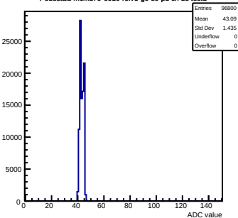
Pedestals mcm170-6010-refv3-g0-s0-p1 ch 13 test1
