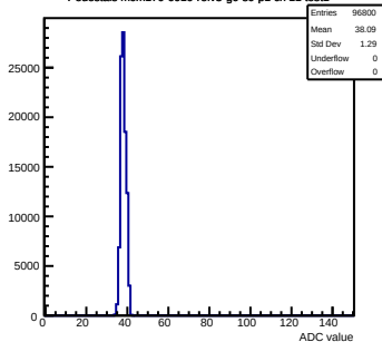
Pedestals mcm170-6010-refv3-g0-s0-p1 ch 11 test1
