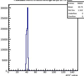
Pedestals mcm170-6010-refv3-g0-s0-p1 ch 72 test1
