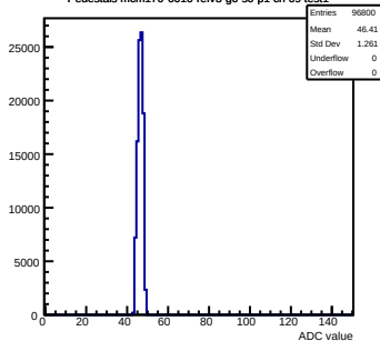
Pedestals mcm170-6010-refv3-g0-s0-p1 ch 69 test1
