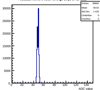
Pedestals mcm170-6010-refv3-g0-s0-p1 ch 10 test1
