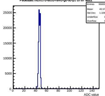
Pedestals mcm170-6010-refv3-g0-s0-p1 ch 67 test1
