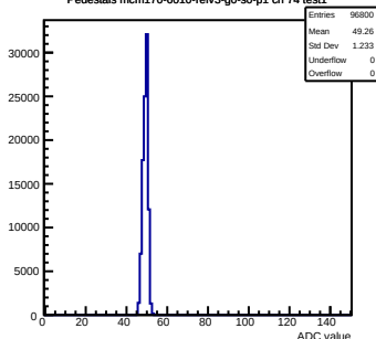
Pedestals mcm170-6010-refv3-g0-s0-p1 ch 74 test1
