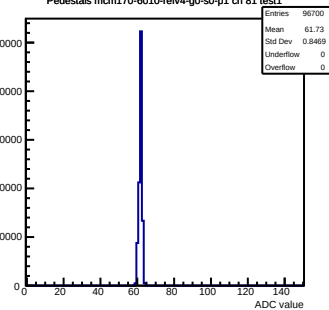
Pedestals mcm170-6010-rtv4-g0-s0-p1 ch 81 test1
