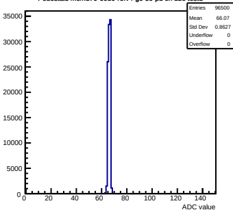
Pedestals mcm170-6010-refv4-g0-s0-p1 ch 126 test1
