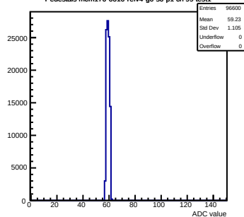
Pedestals mcm170-6010-refv4-g0-s0-p1 ch 99 test1
