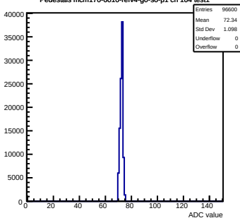
Pedestals mcm170-6010-refv4-g0-s0-p1 ch 104 test1
