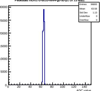
Pedestals mcm170-6010-refv4-g0-s0-p1 ch 13 test1
