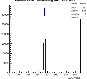
Pedestals mcm170-6010-rlv4-g0-s0-p1 ch 32 test1
