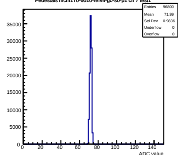
Pedestals mcm170-6010-refv4-g0-s0-p1 ch 7 test1
