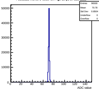
Pedestals mcm170-6010-refv4-g0-s0-p1 ch 123 test1
