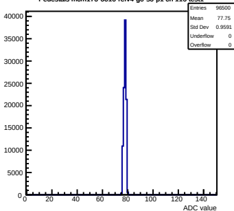
Pedestals mcm170-6010-refv4-g0-s0-p1 ch 116 test1
