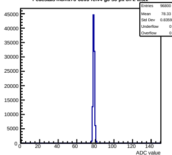
Pedestals mcm170-6010-refv4-g0-s0-p1 ch 2 test1
