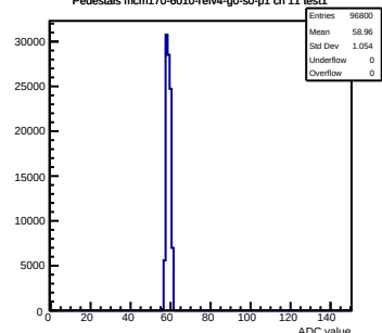
Pedestals mcm170-6010-refv4-g0-s0-p1 ch 11 test1
