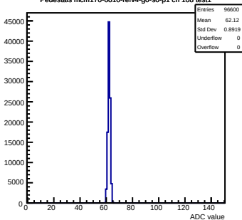
Pedestals mcm170-6010-refv4-g0-s0-p1 ch 108 test1
