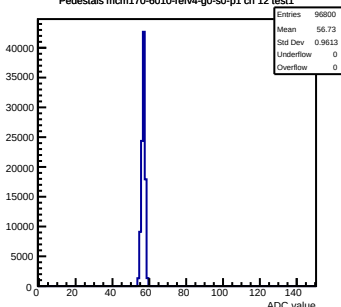
Pedestals mcm170-6010-refv4-g0-s0-p1 ch 12 test1
