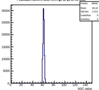
Pedestals mcm170-6010-refv4-g0-s0-p1 ch 96 test1
