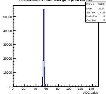
Pedestals mcm170-6010-refv4-g0-s0-p1 ch 109 test1
