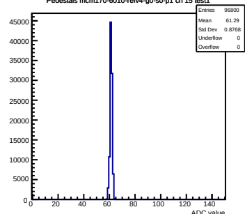
Pedestals mcm170-6010-refv4-g0-s0-p1 ch 15 test1
