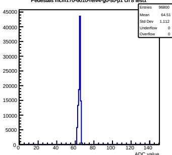
Pedestals mcm170-6010-refv4-g0-s0-p1 ch 8 test1
