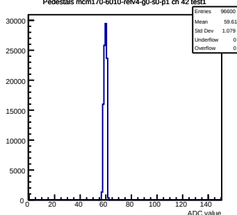
Pedestals mcm170-6010-rlv4-g0-s0-p1 ch 42 test1
