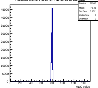
Pedestals mcm170-6010-refv4-g0-s0-p1 ch 113 test1
