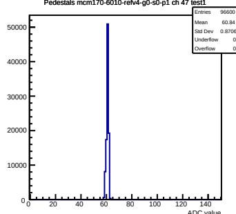
Pedestals mcm170-6010-rlv4-g0-s0-p1 ch 47 test1
