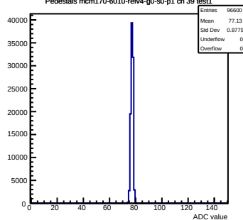
Pedestals mcm170-6010-rlv4-g0-s0-p1 ch 39 test1
