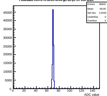
Pedestals mcm170-6010-refv4-g0-s0-p1 ch 106 test1
