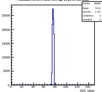
Pedestals mcm170-6010-refv4-g0-s0-p1 ch 112 test1
