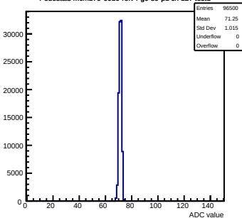
Pedestals mcm170-6010-refv4-g0-s0-p1 ch 127 test1
