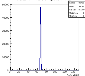
Pedestals mcm170-6010-rtv4-g0-s0-p1 ch 91 test1
