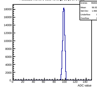
Pedestals mcm170-6010-rtv5-g0-s0-p1 ch 3 test1
