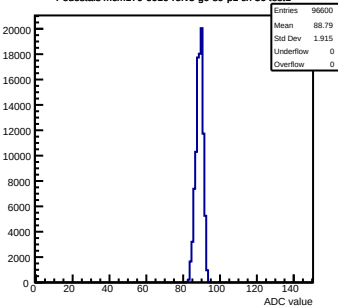
Pedestals mcm170-6010-refV5-g0-s0-p1 ch 36 test1
