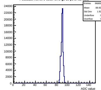
Pedestals mcm170-6010-rtv5-g0-s0-p1 ch 11 test1
