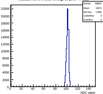
Pedestals mcm170-6010-refV5-g0-s0-p1 ch 44 test1
