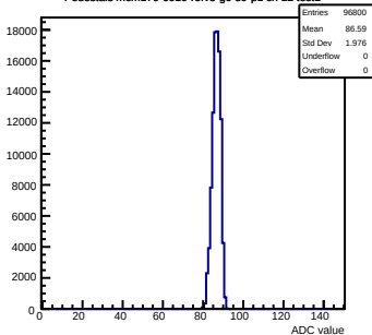
Pedestals mcm170-6010-rtv5-g0-s0-p1 ch 12 test1
