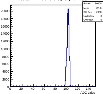
Pedestals mcm170-6010-refV5-g0-s0-p1 ch 40 test1
