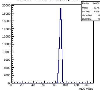
Pedestals mcm170-6010-refV5-g0-s0-p1 ch 42 test1
