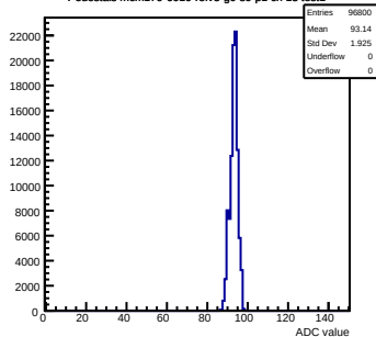
Pedestals mcm170-6010-rtv5-g0-s0-p1 ch 13 test1
