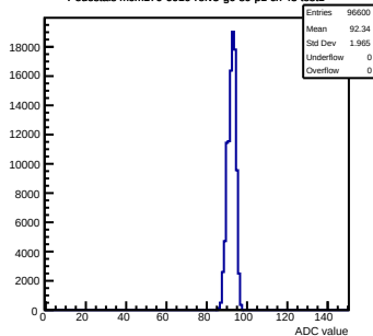
Pedestals mcm170-6010-refV5-g0-s0-p1 ch 43 test1
