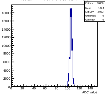
Pedestals mcm170-6010-rtv5-g0-s0-p1 ch 0 test1
