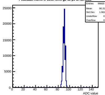
Pedestals mcm170-6010-refV5-g0-s0-p1 ch 33 test1
