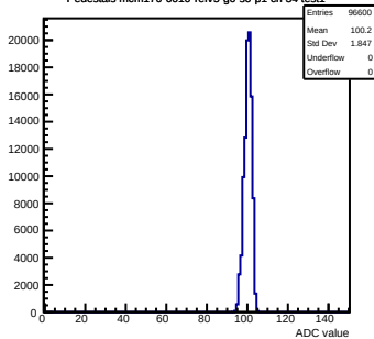
Pedestals mcm170-6010-refV5-g0-s0-p1 ch 34 test1
