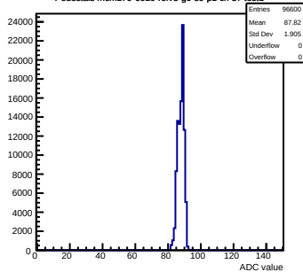
Pedestals mcm170-6010-refV5-g0-s0-p1 ch 37 test1
