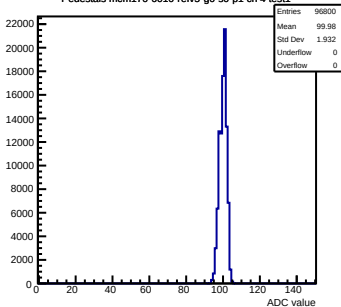
Pedestals mcm170-6010-rtv5-g0-s0-p1 ch 4 test1
