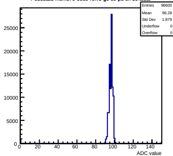
Pedestals mcm170-6010-refV5-g0-s0-p1 ch 38 test1
