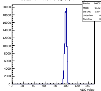
Pedestals mcm170-6010-refV5-g0-s0-p1 ch 41 test1
