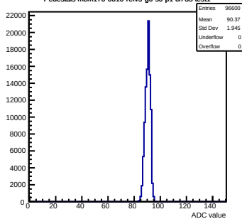
Pedestals mcm170-6010-refV5-g0-s0-p1 ch 35 test1
