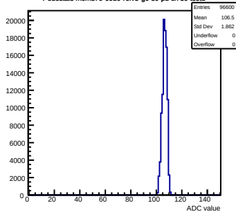
Pedestals mcm170-6010-refV5-g0-s0-p1 ch 39 test1
