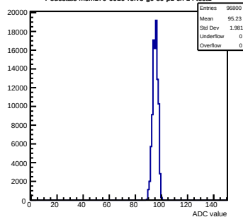
Pedestals mcm170-6010-rtv5-g0-s0-p1 ch 14 test1
