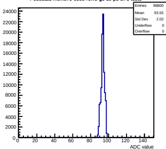
Pedestals mcm170-6010-rtv5-g0-s0-p1 ch 8 test1
