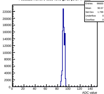
Pedestals mcm170-6010-refV5-g0-s0-p1 ch 47 test1
