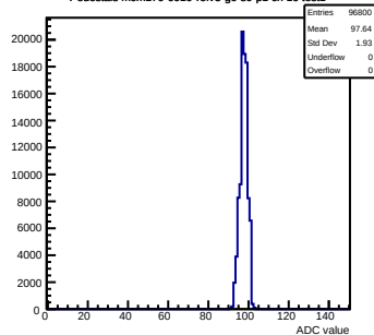
Pedestals mcm170-6010-rtv5-g0-s0-p1 ch 10 test1
