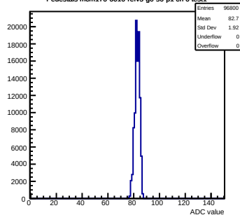
Pedestals mcm170-6010-rtv5-g0-s0-p1 ch 6 test1
