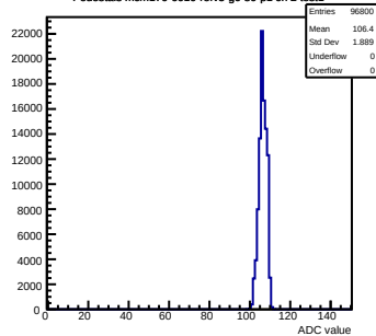
Pedestals mcm170-6010-rtv5-g0-s0-p1 ch 2 test1
