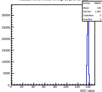
Pedestals mcm170-6010-rtv6-g0-s0-p1 ch 32 test1
