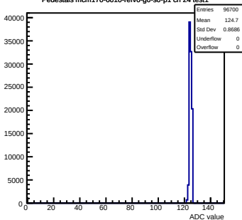
Pedestals mcm170-6010-rtv6-g0-s0-p1 ch 24 test1
