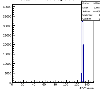
Pedestals mcm170-6010-relv6-g0-s0-p1 ch 79 test1
