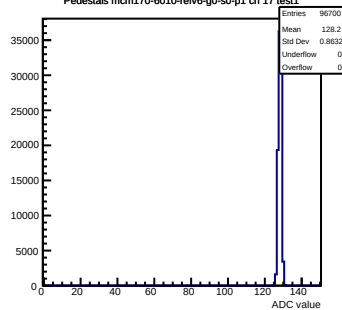
Pedestals mcm170-6010-rtv6-g0-s0-p1 ch 17 test1
