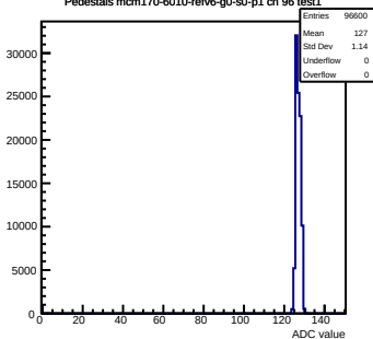
Pedestals mcm170-6010-refv6-g0-s0-p1 ch 96 test1
