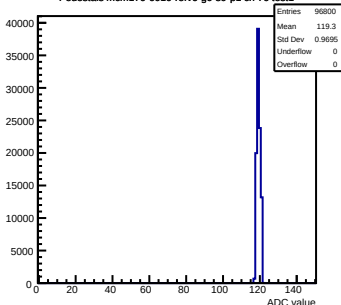
Pedestals mcm170-6010-relv6-g0-s0-p1 ch 76 test1
