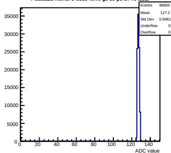
Pedestals mcm170-6010-relv6-g0-s0-p1 ch 70 test1
