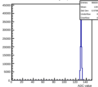
Pedestals mcm170-6010-rtv6-g0-s0-p1 ch 46 test1
