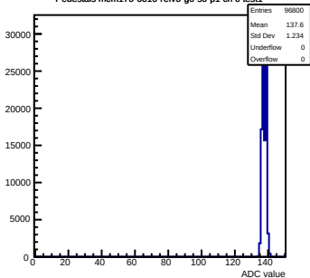
Pedestals mcm170-6010-rtv6-g0-s0-p1 ch 0 test1
