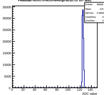
Pedestals mcm170-6010-refv6-g0-s0-p1 ch 107 test1
