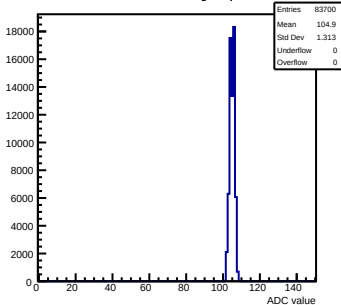
Pedestals mcm171-7611-rfv1-g0-s0-p1 ch 56 test1
