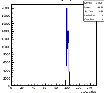
Pedestals mcm171-7611-rlv1-g0-s0-p1 ch 68 test1
