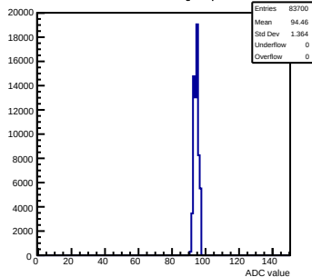
Pedestals mcm171-7611-rfv1-g0-s0-p1 ch 61 test1
