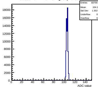
Pedestals mcm171-7611-rfv1-g0-s0-p1 ch 50 test1
