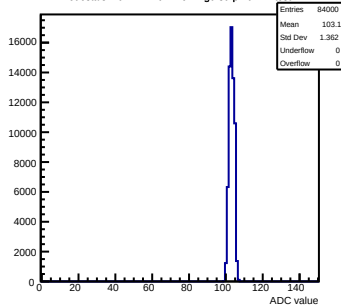
Pedestals mcm171-7611-rlv1-g0-s0-p1 ch 71 test1
