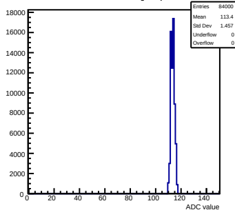
Pedestals mcm171-7611-rlv1-g0-s0-p1 ch 75 test1
