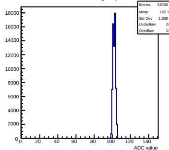
Pedestals mcm171-7611-rfv1-g0-s0-p1 ch 63 test1
