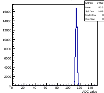
Pedestals mcm171-7611-rlv1-g0-s0-p1 ch 77 test1
