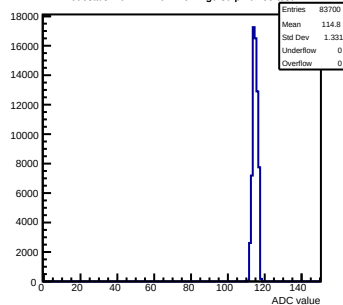
Pedestals mcm171-7611-rfv1-g0-s0-p1 ch 55 test1
