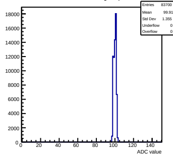
Pedestals mcm171-7611-rfv1-g0-s0-p1 ch 59 test1
