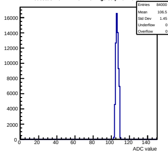
Pedestals mcm171-7611-rlv1-g0-s0-p1 ch 70 test1
