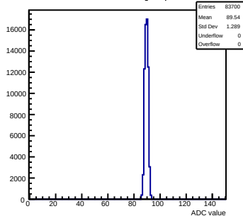
Pedestals mcm171-7611-rfv1-g0-s0-p1 ch 57 test1
