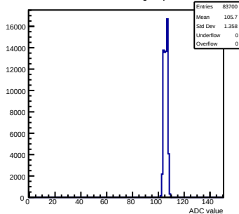
Pedestals mcm171-7611-rfv1-g0-s0-p1 ch 58 test1
