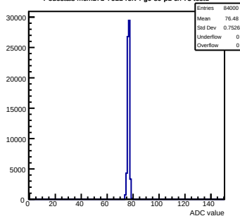
Pedestals mcm171-7611-rlv4-g0-s0-p1 ch 73 test1
