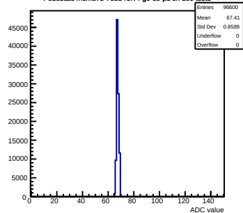
Pedestals mcm171-7611-refv4-g0-s0-p1 ch 100 test1
