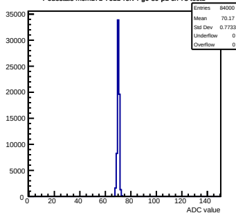
Pedestals mcm171-7611-rlv4-g0-s0-p1 ch 78 test1
