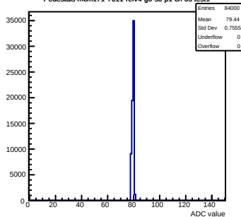
Pedestals mcm171-7611-rlv4-g0-s0-p1 ch 65 test1
