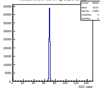
Pedestals mcm171-7611-refv4-g0-s0-p1 ch 98 test1
