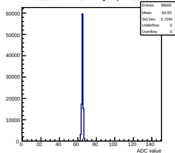
Pedestals mcm171-7611-refv4-g0-s0-p1 ch 108 test1
