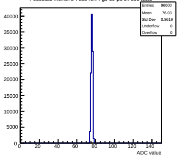
Pedestals mcm171-7611-refv4-g0-s0-p1 ch 103 test1
