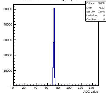
Pedestals mcm171-7611-refv4-g0-s0-p1 ch 110 test1
