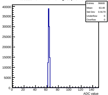
Pedestals mcm171-7611-refv4-g0-s0-p1 ch 107 test1
