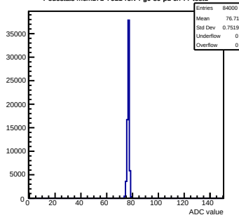
Pedestals mcm171-7611-rlv4-g0-s0-p1 ch 77 test1
