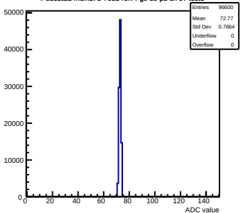
Pedestals mcm171-7611-refv4-g0-s0-p1 ch 97 test1
