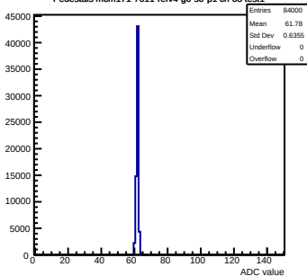
Pedestals mcm171-7611-rlv4-g0-s0-p1 ch 68 test1
