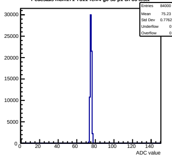
Pedestals mcm171-7611-rlv4-g0-s0-p1 ch 66 test1
