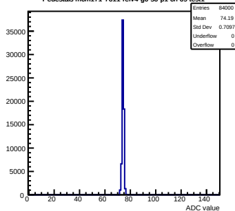
Pedestals mcm171-7611-rlv4-g0-s0-p1 ch 69 test1
