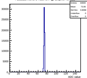
Pedestals mcm171-7611-rlv4-g0-s0-p1 ch 72 test1
