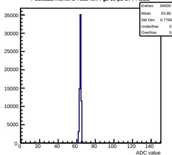
Pedestals mcm171-7611-rlv4-g0-s0-p1 ch 74 test1
