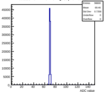
Pedestals mcm171-7611-refv4-g0-s0-p1 ch 109 test1
