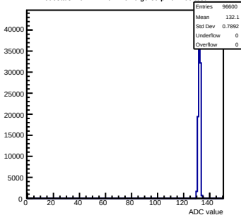
Pedestals mcm171-7611- rfv6-g0-s0-p1 ch 100 test1
