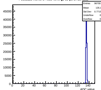
Pedestals mcm171-7611-relv6-g0-s0-p1 ch 31 test1
