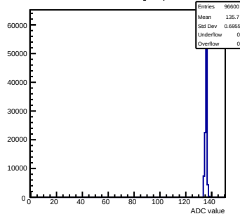
Pedestals mcm171-7611- rfv6-g0-s0-p1 ch 110 test1
