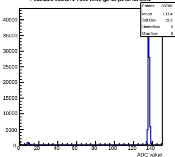
Pedestals mcm171-7611-rlv6-g0-s0-p1 ch 48 test1
