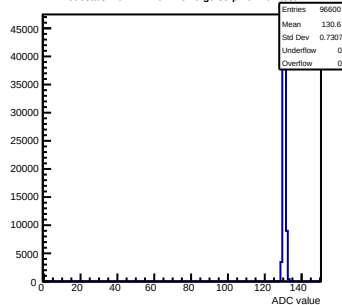
Pedestals mcm171-7611- rfv6-g0-s0-p1 ch 102 test1
