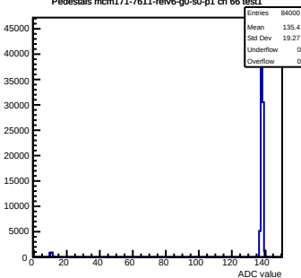
Pedestals mcm171-7611-relv6-g0-s0-p1 ch 66 test1
