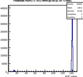
Pedestals mcm171-7611-relv6-g0-s0-p1 ch 73 test1
