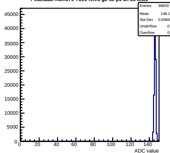
Pedestals mcm171-7611-rlv6-g0-s0-p1 ch 33 test1
