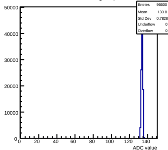
Pedestals mcm171-7611- rfv6-g0-s0-p1 ch 109 test1
