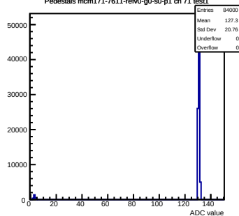
Pedestals mcm171-7611-rev0-g0-s0-p1 ch 71 test1
