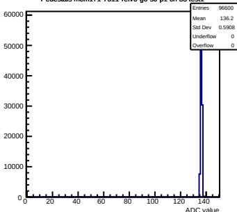
Pedestals mcm171-7611-rev0-g0-s0-p1 ch 38 test1
