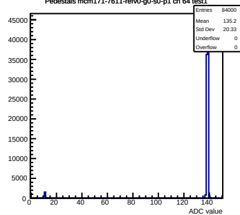
Pedestals mcm171-7611-rev0-g0-s0-p1 ch 64 test1
