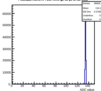
Pedestals mcm171-7611-rev0-g0-s0-p1 ch 35 test1
