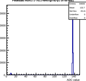
Pedestals mcm171-7611-rev0-g0-s0-p1 ch 69 test1
