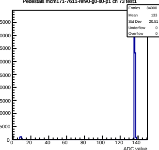
Pedestals mcm171-7611-rev0-g0-s0-p1 ch 73 test1
