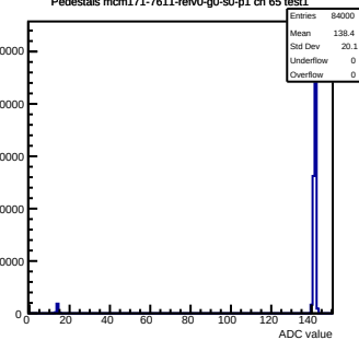
Pedestals mcm171-7611-rev0-g0-s0-p1 ch 65 test1
