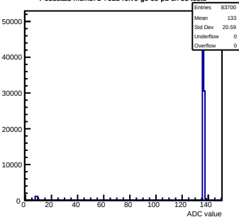
Pedestals mcm171-7611-rev0-g0-s0-p1 ch 53 test1
