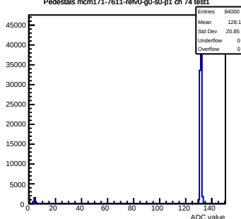
Pedestals mcm171-7611-rev0-g0-s0-p1 ch 74 test1
