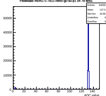
Pedestals mcm171-7611-rev0-g0-s0-p1 ch 79 test1
