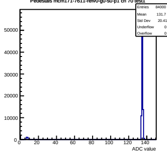
Pedestals mcm171-7611-rev0-g0-s0-p1 ch 70 test1
