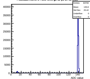
Pedestals mcm171-7611-rev0-g0-s0-p1 ch 48 test1
