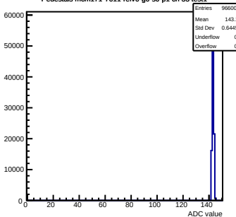
Pedestals mcm171-7611-rev0-g0-s0-p1 ch 33 test1
