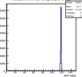
Pedestals mcm171-7611-rlv1-g0-s0-p1 ch 49 test1
