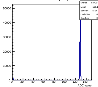
Pedestals mcm171-7611-rlv1-g0-s0-p1 ch 55 test1
