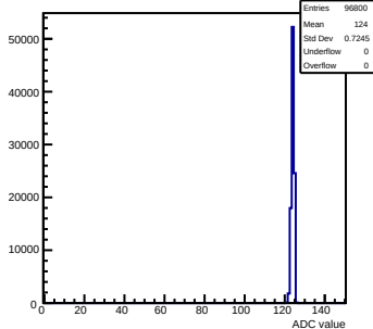
Pedestals mcm171-7611-refv1-g0-s0-p1 ch 13 test1
