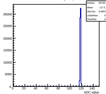
Pedestals mcm171-7611-rlv1-g0-s0-p1 ch 59 test1
