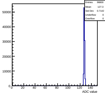
Pedestals mcm171-7611-refv1-g0-s0-p1 ch 9 test1
