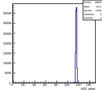
Pedestals mcm171-7611-refv1-g0-s0-p1 ch 11 test1
