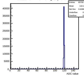
Pedestals mcm171-7611-rlv1-g0-s0-p1 ch 54 test1
