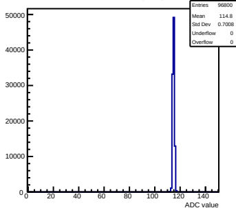
Pedestals mcm171-7611-refv1-g0-s0-p1 ch 1 test1
