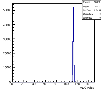
Pedestals mcm171-7611-refv1-g0-s0-p1 ch 15 test1
