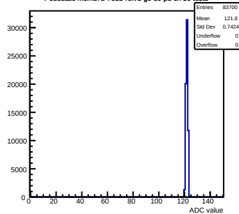
Pedestals mcm171-7611-rlv1-g0-s0-p1 ch 50 test1
