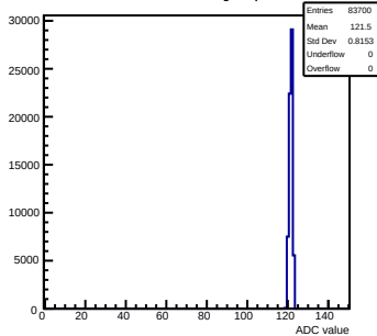
Pedestals mcm171-7611-rlv1-g0-s0-p1 ch 60 test1
