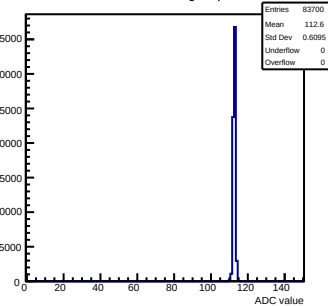
Pedestals mcm171-7611-rlv1-g0-s0-p1 ch 57 test1
