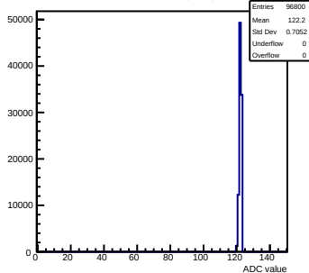
Pedestals mcm171-7611-refv1-g0-s0-p1 ch 6 test1
