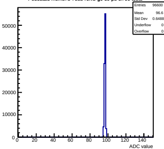
Pedestals mcm171-7611-refv2-g0-s0-p1 ch 99 test1
