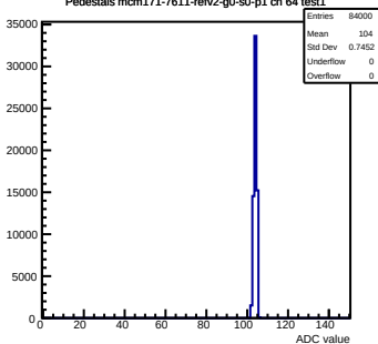
Pedestals mcm171-7611-refv2-g0-s0-p1 ch 64 test1
