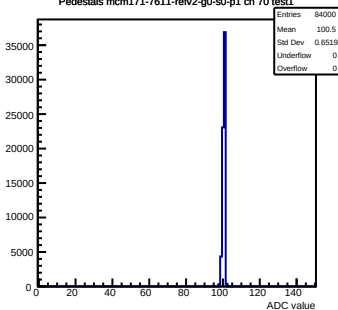
Pedestals mcm171-7611-refv2-g0-s0-p1 ch 70 test1
