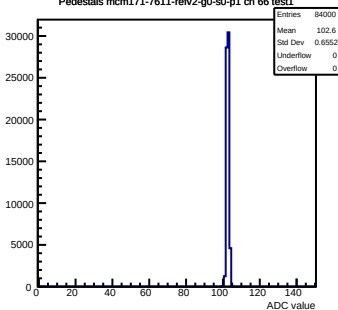
Pedestals mcm171-7611-refv2-g0-s0-p1 ch 66 test1
