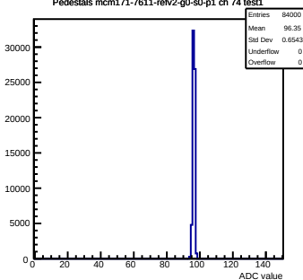
Pedestals mcm171-7611-refv2-g0-s0-p1 ch 74 test1
