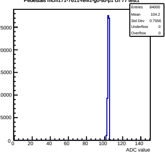
Pedestals mcm171-7611-refv2-g0-s0-p1 ch 77 test1
