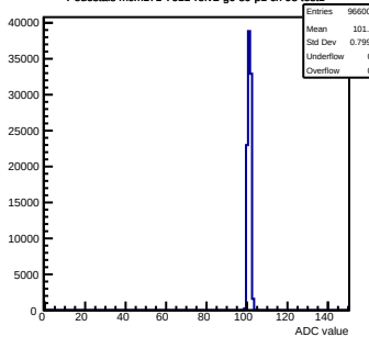
Pedestals mcm171-7611-refv2-g0-s0-p1 ch 98 test1
