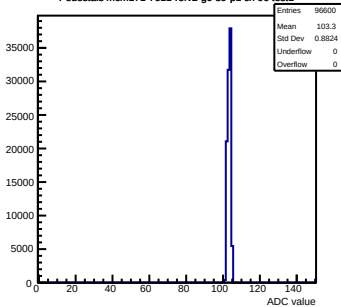
Pedestals mcm171-7611-refv2-g0-s0-p1 ch 96 test1
