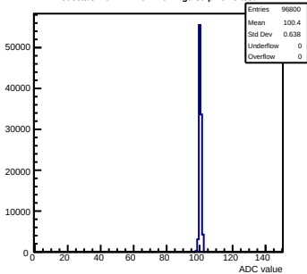
Pedestals mcm171-7611-refv2-g0-s0-p1 ch 8 test1
