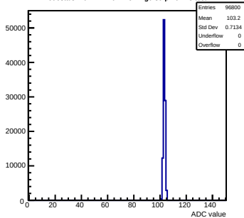
Pedestals mcm171-7611-refv2-g0-s0-p1 ch 13 test1
