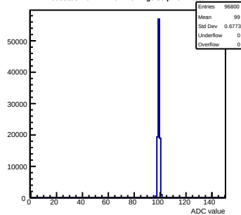
Pedestals mcm171-7611-refv2-g0-s0-p1 ch 7 test1
