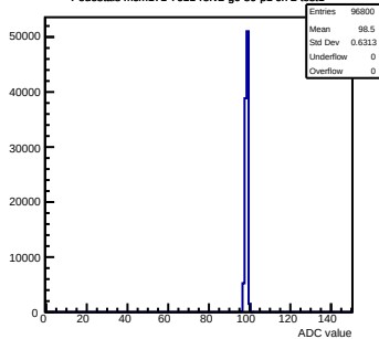
Pedestals mcm171-7611-refv2-g0-s0-p1 ch 2 test1
