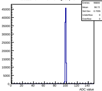
Pedestals mcm171-7611-refv2-g0-s0-p1 ch 4 test1
