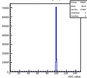
Pedestals mcm171-7611-refv2-g0-s0-p1 ch 5 test1
