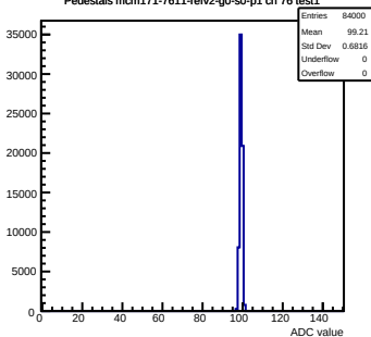
Pedestals mcm171-7611-refv2-g0-s0-p1 ch 76 test1
