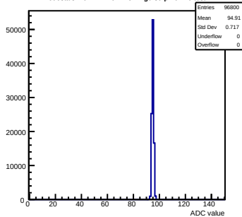
Pedestals mcm171-7611-refv2-g0-s0-p1 ch 10 test1
