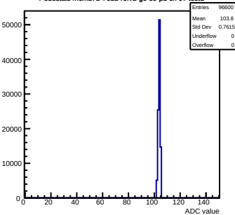
Pedestals mcm171-7611-refv2-g0-s0-p1 ch 97 test1
