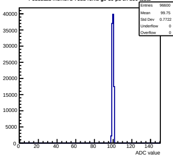
Pedestals mcm171-7611-refv2-g0-s0-p1 ch 100 test1
