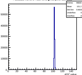
Pedestals mcm171-7611-refv2-g0-s0-p1 ch 109 test1
