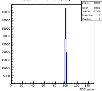
Pedestals mcm171-7611-refv2-g0-s0-p1 ch 0 test1
