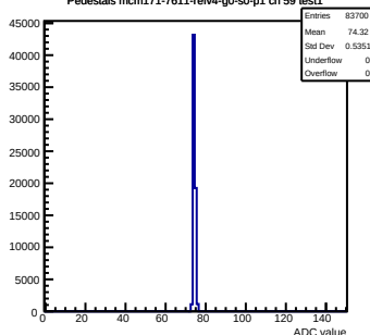
Pedestals mcm171-7611-rv4-g0-s0-p1 ch 59 test1
