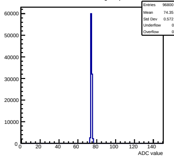
Pedestals mcm171-7611-rfv4-g0-s0-p1 ch 14 test1
