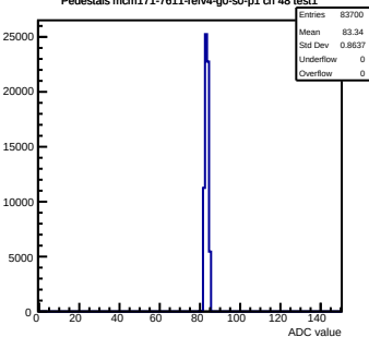
Pedestals mcm171-7611-rv4-g0-s0-p1 ch 48 test1
