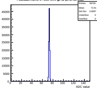
Pedestals mcm171-7611-rv4-g0-s0-p1 ch 80 test1
