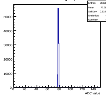
Pedestals mcm171-7611-rfv4-g0-s0-p1 ch 7 test1
