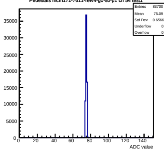
Pedestals mcm171-7611-rv4-g0-s0-p1 ch 54 test1
