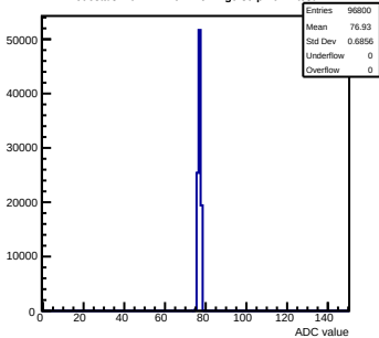
Pedestals mcm171-7611-rfv4-g0-s0-p1 ch 4 test1
