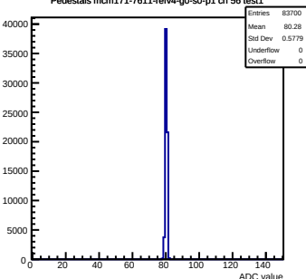
Pedestals mcm171-7611-rv4-g0-s0-p1 ch 56 test1
