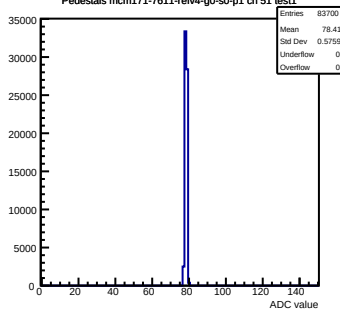
Pedestals mcm171-7611-rv4-g0-s0-p1 ch 51 test1
