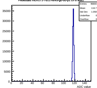
Pedestals mcm171-7611-refV5-g0-s0-p1 ch 6 test1
