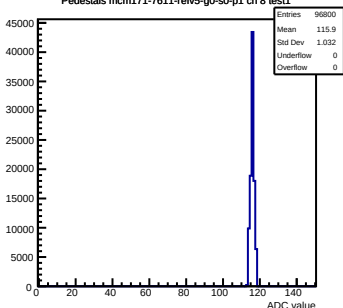
Pedestals mcm171-7611-refV5-g0-s0-p1 ch 8 test1
