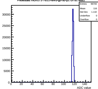
Pedestals mcm171-7611-refV5-g0-s0-p1 ch 81 test1
