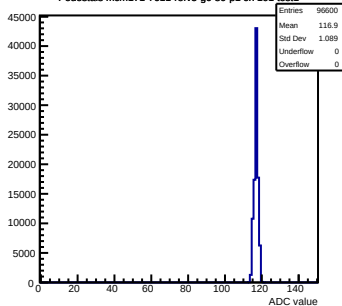
Pedestals mcm171-7611-refV5-g0-s0-p1 ch 101 test1
