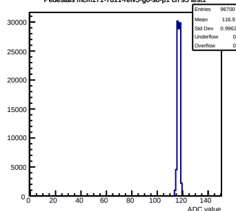
Pedestals mcm171-7611-refV5-g0-s0-p1 ch 95 test1
