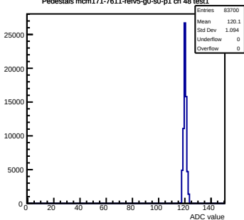
Pedestals mcm171-7611- rev5-g0-s0-p1 ch 48 test1
