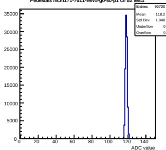
Pedestals mcm171-7611-refV5-g0-s0-p1 ch 82 test1
