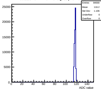
Pedestals mcm171-7611-refV5-g0-s0-p1 ch 70 test1
