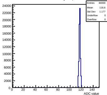
Pedestals mcm171-7611-refV5-g0-s0-p1 ch 78 test1
