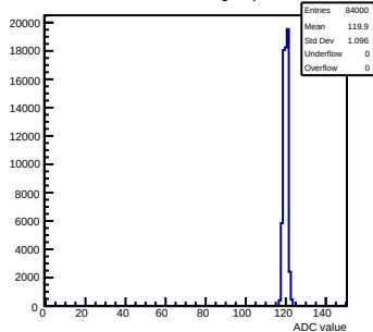
Pedestals mcm171-7611-refV5-g0-s0-p1 ch 77 test1
