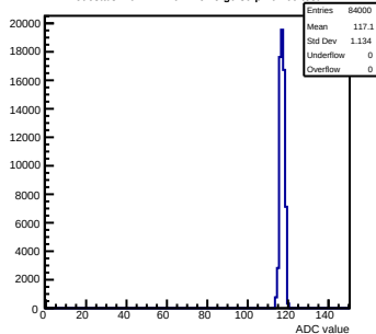
Pedestals mcm171-7611-refV5-g0-s0-p1 ch 69 test1
