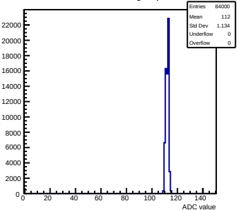
Pedestals mcm171-7611-refV5-g0-s0-p1 ch 79 test1
