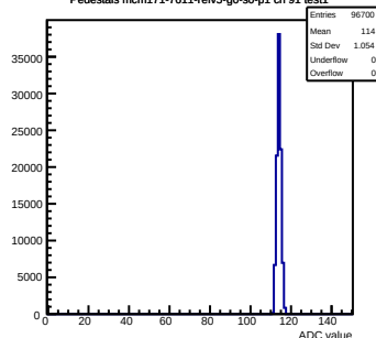
Pedestals mcm171-7611-refV5-g0-s0-p1 ch 91 test1
