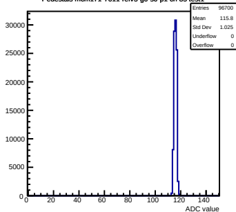
Pedestals mcm171-7611-refV5-g0-s0-p1 ch 85 test1
