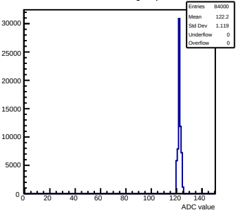
Pedestals mcm171-7611-refV5-g0-s0-p1 ch 75 test1
