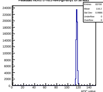
Pedestals mcm171-7611- rev5-g0-s0-p1 ch 58 test1
