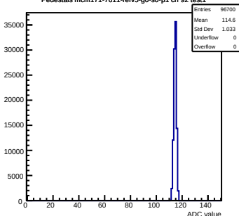
Pedestals mcm171-7611-refV5-g0-s0-p1 ch 92 test1
