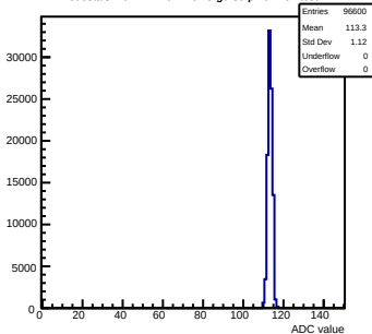
Pedestals mcm171-7611-refV5-g0-s0-p1 ch 104 test1
