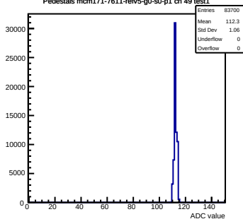
Pedestals mcm171-7611- rev5-g0-s0-p1 ch 49 test1
