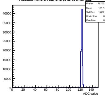
Pedestals mcm171-7611-refV5-g0-s0-p1 ch 86 test1
