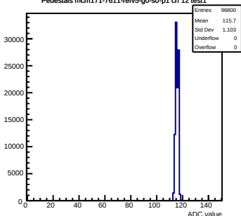
Pedestals mcm171-7611-refV5-g0-s0-p1 ch 12 test1
