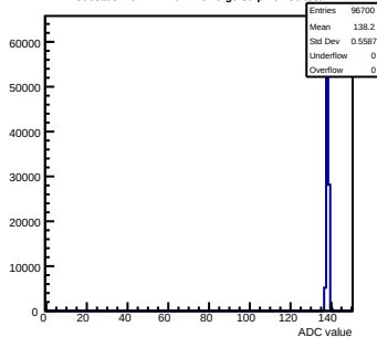
Pedestals mcm171-7611-rev0-g0-s0-p1 ch 86 test1
