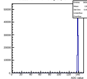
Pedestals mcm171-7611-refV0-g0-s0-p1 ch 119 test1
