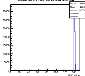
Pedestals mcm171-7611- \text{rev0-g0-s0-p1} ch 42 test1
