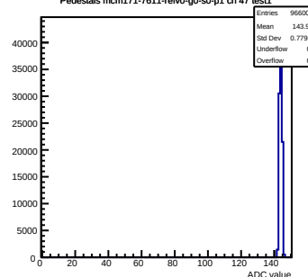
Pedestals mcm171-7611- \text{rev0-g0-s0-p1} ch 47 test1
