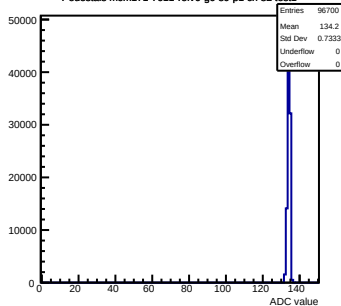
Pedestals mcm171-7611-rev0-g0-s0-p1 ch 82 test1
