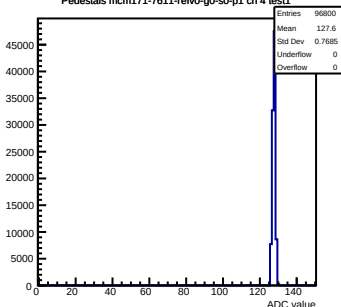
Pedestals mcm171-7611-refV0-g0-s0-p1 ch 4 test1
