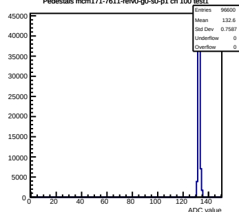
Pedestals mcm171-7611-refV0-g0-s0-p1 ch 100 test1
