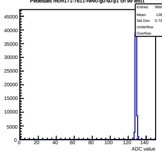
Pedestals mcm171-7611-refV0-g0-s0-p1 ch 99 test1
