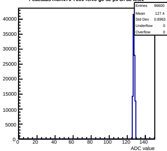
Pedestals mcm171-7611- \text{rev0-g0-s0-p1} ch 32 test1
