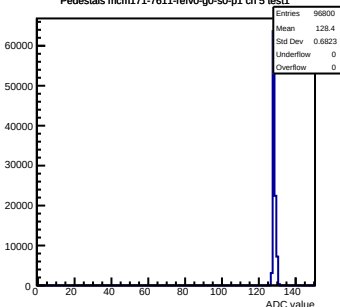
Pedestals mcm171-7611-refV0-g0-s0-p1 ch 5 test1
