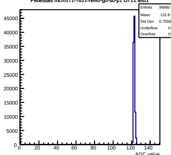
Pedestals mcm171-7611-refV0-g0-s0-p1 ch 11 test1
