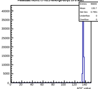
Pedestals mcm171-7611-refV0-g0-s0-p1 ch 6 test1
