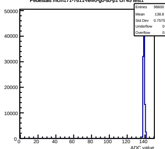
Pedestals mcm171-7611- \text{rev0-g0-s0-p1} ch 45 test1
