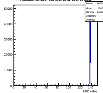
Pedestals mcm171-7611- \text{rev0-g0-s0-p1} ch 35 test1
