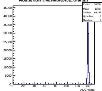
Pedestals mcm171-7611-refV0-g0-s0-p1 ch 96 test1
