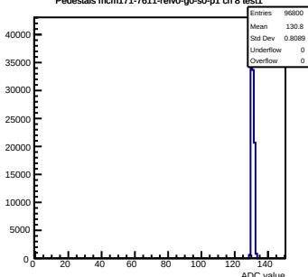
Pedestals mcm171-7611-refV0-g0-s0-p1 ch 8 test1
