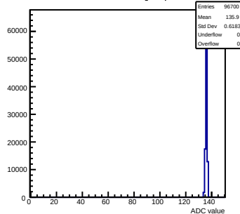
Pedestals mcm171-7611-rev0-g0-s0-p1 ch 95 test1
