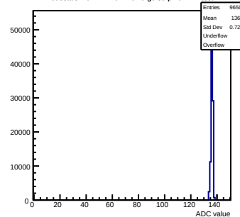
Pedestals mcm171-7611-refV0-g0-s0-p1 ch 127 test1
