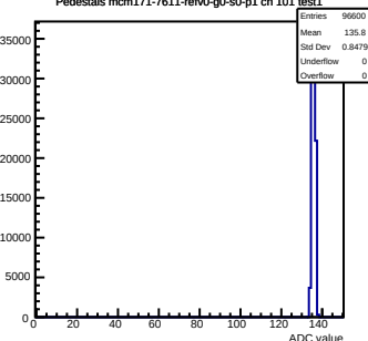
Pedestals mcm171-7611-refV0-g0-s0-p1 ch 101 test1
