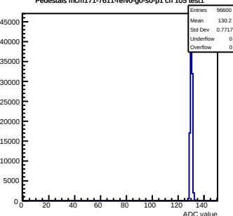
Pedestals mcm171-7611-refV0-g0-s0-p1 ch 105 test1
