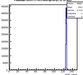
Pedestals mcm171-7611-refV0-g0-s0-p1 ch 10 test1
