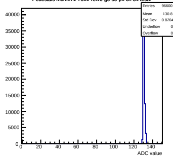
Pedestals mcm171-7611- \text{rev0-g0-s0-p1} ch 34 test1
