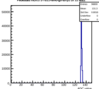
Pedestals mcm171-7611-refV0-g0-s0-p1 ch 12 test1
