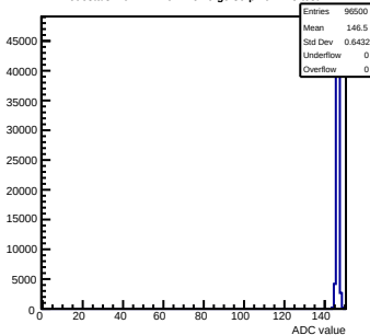
Pedestals mcm171-7611-refV0-g0-s0-p1 ch 125 test1
