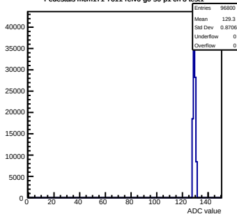
Pedestals mcm171-7611-refV0-g0-s0-p1 ch 3 test1
