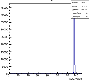
Pedestals mcm171-7611-refV0-g0-s0-p1 ch 116 test1
