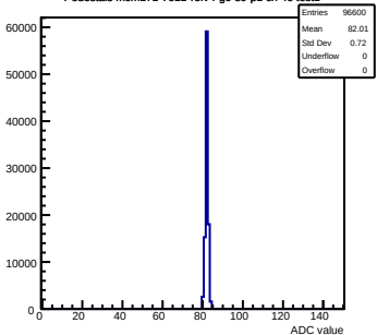
Pedestals mcm171-7611-rlv4-g0-s0-p1 ch 46 test1
