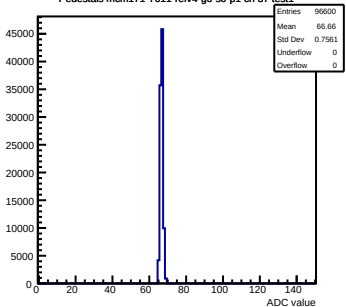
Pedestals mcm171-7611-rlv4-g0-s0-p1 ch 37 test1
