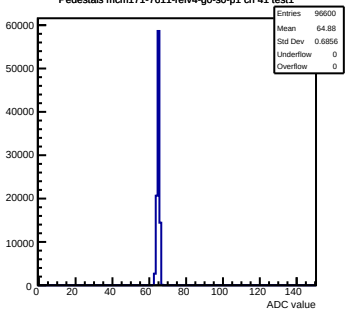
Pedestals mcm171-7611-rlv4-g0-s0-p1 ch 41 test1
