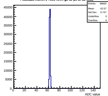
Pedestals mcm171-7611-rlv4-g0-s0-p1 ch 32 test1
