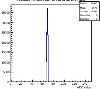
Pedestals mcm171-7611-rlv4-g0-s0-p1 ch 34 test1
