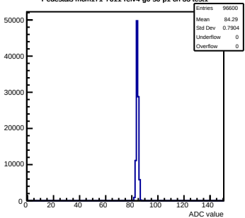
Pedestals mcm171-7611-rlv4-g0-s0-p1 ch 33 test1
