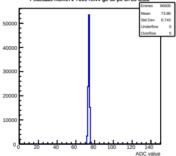
Pedestals mcm171-7611-rlv4-g0-s0-p1 ch 39 test1
