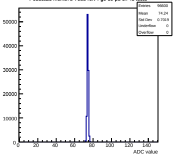
Pedestals mcm171-7611-rlv4-g0-s0-p1 ch 45 test1
