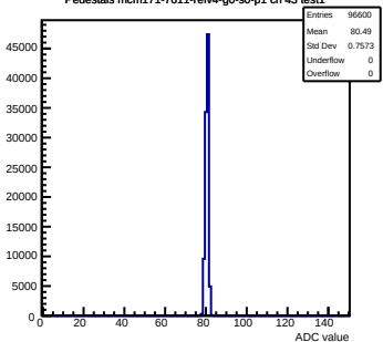
Pedestals mcm171-7611-rlv4-g0-s0-p1 ch 43 test1
