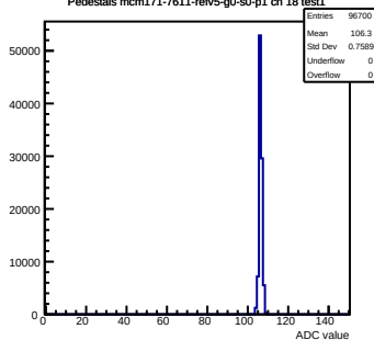
Pedestals mcm171-7611-rfv5-g0-s0-p1 ch 18 test1
