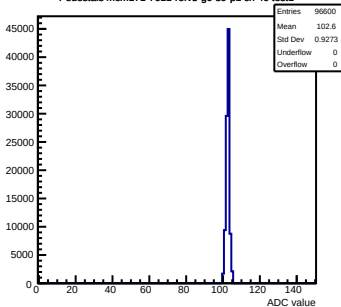
Pedestals mcm171-7611- \text{rev5-g0-s0-p1} ch 40 test1
