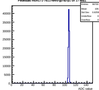
Pedestals mcm171-7611-rfv5-g0-s0-p1 ch 17 test1
