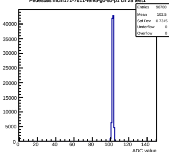
Pedestals mcm171-7611-rfv5-g0-s0-p1 ch 28 test1
