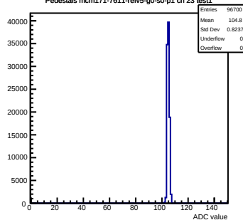
Pedestals mcm171-7611-rfv5-g0-s0-p1 ch 23 test1
