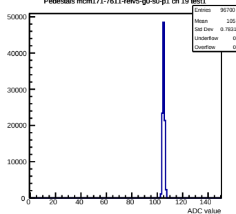
Pedestals mcm171-7611-rfv5-g0-s0-p1 ch 19 test1
