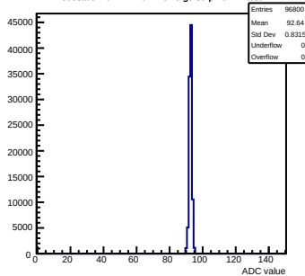
Pedestals mcm171-7611-refV5-g0-s0-p1 ch 14 test1
