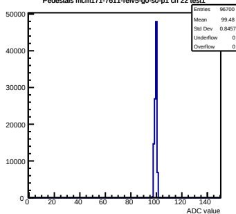
Pedestals mcm171-7611-rfv5-g0-s0-p1 ch 22 test1
