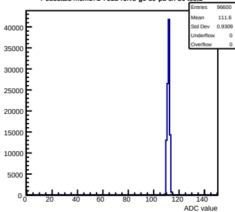
Pedestals mcm171-7611- \text{rev5-g0-s0-p1} ch 36 test1
