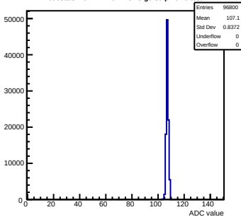
Pedestals mcm171-7611-refV5-g0-s0-p1 ch 9 test1
