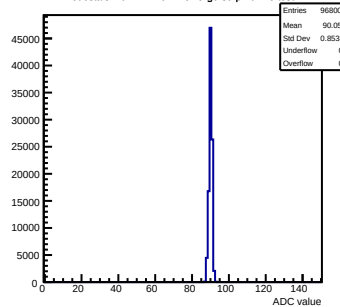
Pedestals mcm171-7611-refV5-g0-s0-p1 ch 15 test1
