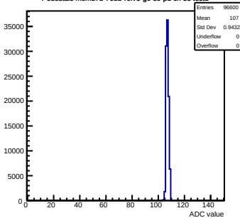
Pedestals mcm171-7611- \text{rev5-g0-s0-p1} ch 38 test1
