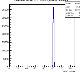
Pedestals mcm171-7611-rfv5-g0-s0-p1 ch 26 test1
