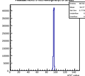
Pedestals mcm171-7611-rfv5-g0-s0-p1 ch 30 test1
