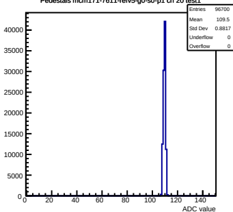
Pedestals mcm171-7611-rfv5-g0-s0-p1 ch 20 test1
