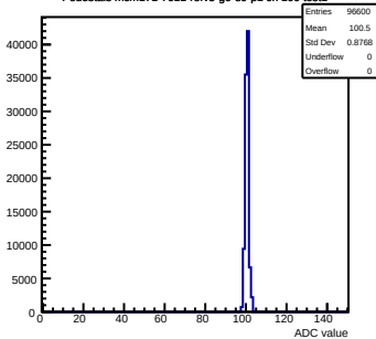
Pedestals mcm171-7611-refV5-g0-s0-p1 ch 100 test1
