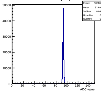
Pedestals mcm171-7611-refV5-g0-s0-p1 ch 10 test1
