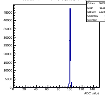
Pedestals mcm171-7611-refV5-g0-s0-p1 ch 7 test1
