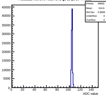
Pedestals mcm171-7611- \text{rev5-g0-s0-p1} ch 44 test1
