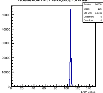
Pedestals mcm171-7611-rfv5-g0-s0-p1 ch 24 test1
