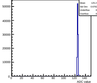
Pedestals mcm171-7611-refv6-g0-s0-p1 ch 126 test1
