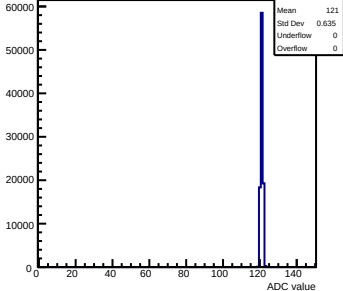
Pedestals mcm171-7611-refv6-g0-s0-p1 ch 124 test1
