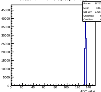
Pedestals mcm171-7611-relv6-g0-s0-p1 ch 26 test1
