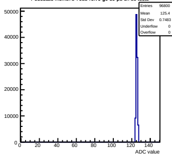
Pedestals mcm171-7611-rlv6-g0-s0-p1 ch 10 test1
