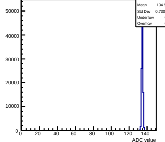
Pedestals mcm171-7611-refv6-g0-s0-p1 ch 127 test1
