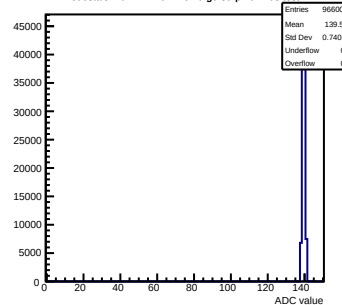
Pedestals mcm171-7611-rlv6-g0-s0-p1 ch 103 test1
