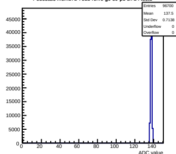
Pedestals mcm171-7611-relv6-g0-s0-p1 ch 24 test1
