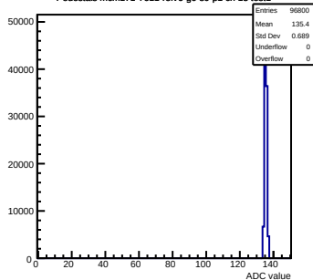
Pedestals mcm171-7611-rlv6-g0-s0-p1 ch 13 test1
