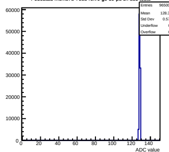
Pedestals mcm171-7611-refv6-g0-s0-p1 ch 115 test1
