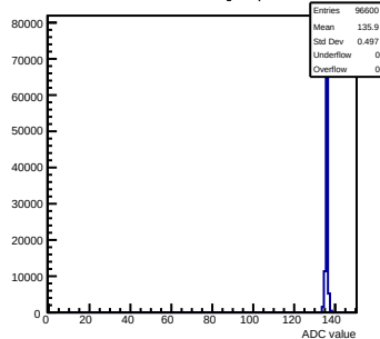
Pedestals mcm171-7611-rlv6-g0-s0-p1 ch 110 test1
