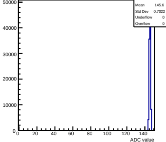
Pedestals mcm171-7611-refv6-g0-s0-p1 ch 125 test1
