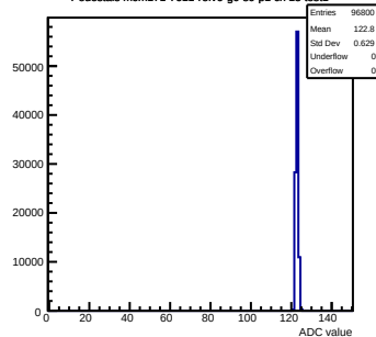
Pedestals mcm171-7611-rlv6-g0-s0-p1 ch 15 test1
