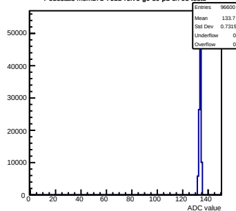
Pedestals mcm171-7611-rlv6-g0-s0-p1 ch 98 test1
