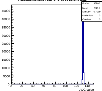
Pedestals mcm171-7611-rlv6-g0-s0-p1 ch 0 test1
