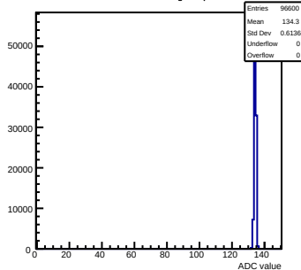
Pedestals mcm171-7611-rlv6-g0-s0-p1 ch 109 test1
