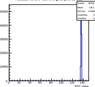
Pedestals mcm171-7611-relv6-g0-s0-p1 ch 25 test1
