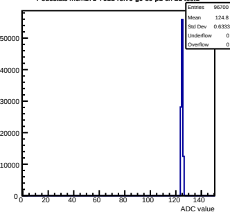
Pedestals mcm171-7611-relv6-g0-s0-p1 ch 21 test1
