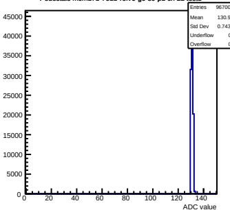
Pedestals mcm171-7611-relv6-g0-s0-p1 ch 22 test1
