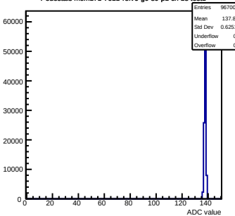
Pedestals mcm171-7611-relv6-g0-s0-p1 ch 18 test1
