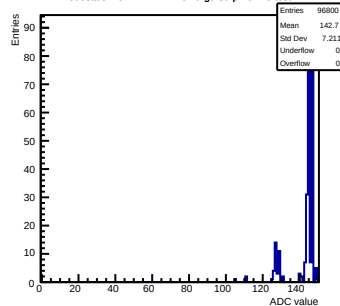
Pedestals mcm172-7417-rev0-g0-s0-p1 ch 79 test1
