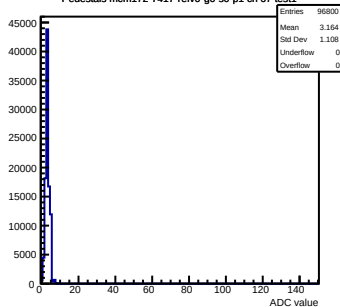
Pedestals mcm172-7417-rev0-g0-s0-p1 ch 67 test1
