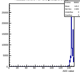
Pedestals mcm172-7417-refV0-g0-s0-p1 ch 2 test1
