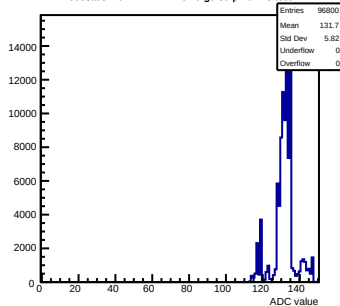
Pedestals mcm172-7417-rev0-g0-s0-p1 ch 78 test1
