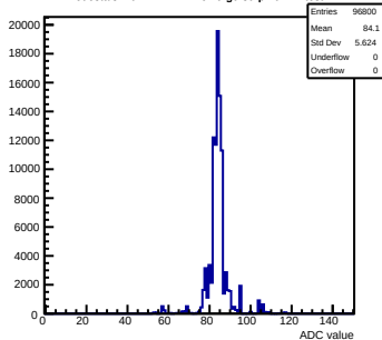
Pedestals mcm172-7417-rev0-g0-s0-p1 ch 72 test1
