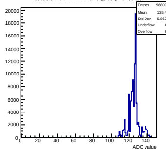
Pedestals mcm172-7417-rev0-g0-s0-p1 ch 69 test1
