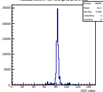
Pedestals mcm172-7417-refV0-g0-s0-p1 ch 6 test1
