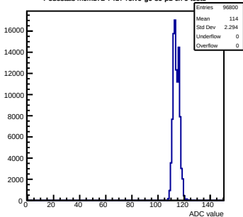
Pedestals mcm172-7417-refV0-g0-s0-p1 ch 0 test1
