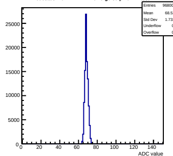
Pedestals mcm172-7417-rev0-g0-s0-p1 ch 77 test1
