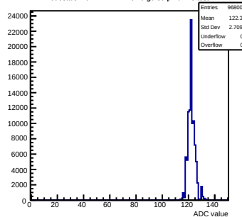
Pedestals mcm172-7417-rev0-g0-s0-p1 ch 73 test1
