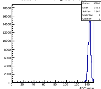
Pedestals mcm172-7417-refv1-g0-s0-p1 ch 13 test1
