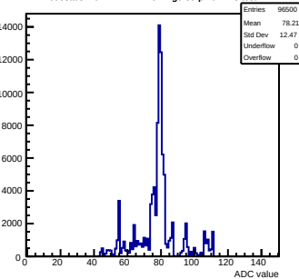
Pedestals mcm172-7417-refv1-g0-s0-p1 ch 125 test1
