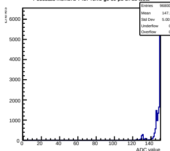
Pedestals mcm172-7417-refv1-g0-s0-p1 ch 11 test1
