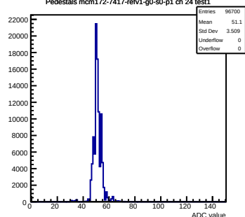
Pedestals mcm172-7417-rfv1-g0-s0-p1 ch 24 test1
