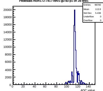
Pedestals mcm172-7417-rfv1-g0-s0-p1 ch 28 test1
