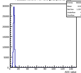
Pedestals mcm172-7417-relv1-g0-s0-p1 ch 59 test1
