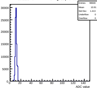
Pedestals mcm172-7417-relv1-g0-s0-p1 ch 60 test1
