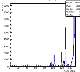
Pedestals mcm172-7417-relv1-g0-s0-p1 ch 61 test1
