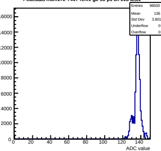
Pedestals mcm172-7417-refv1-g0-s0-p1 ch 113 test1
