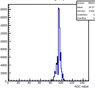
Pedestals mcm172-7417-refv1-g0-s0-p1 ch 121 test1
