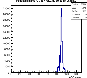
Pedestals mcm172-7417-rfv1-g0-s0-p1 ch 26 test1
