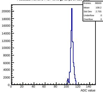
Pedestals mcm172-7417-refv1-g0-s0-p1 ch 116 test1
