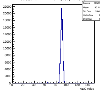
Pedestals mcm172-7417-relv1-g0-s0-p1 ch 55 test1
