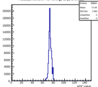
Pedestals mcm172-7417-refv1-g0-s0-p1 ch 9 test1
