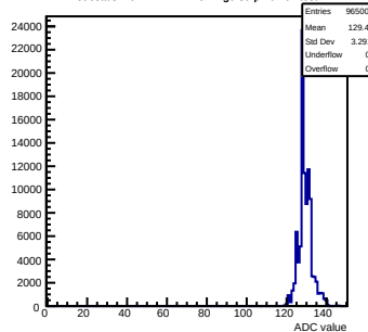
Pedestals mcm172-7417-relv1-g0-s0-p1 ch 62 test1
