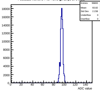
Pedestals mcm172-7417-refv1-g0-s0-p1 ch 0 test1
