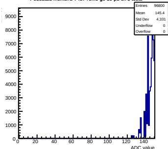
Pedestals mcm172-7417-refv1-g0-s0-p1 ch 8 test1
