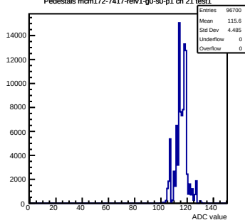
Pedestals mcm172-7417-rfv1-g0-s0-p1 ch 21 test1
