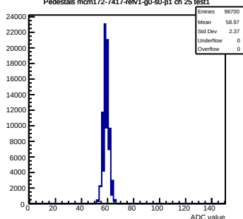
Pedestals mcm172-7417-rfv1-g0-s0-p1 ch 25 test1
