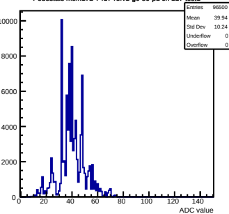
Pedestals mcm172-7417-refv1-g0-s0-p1 ch 117 test1
