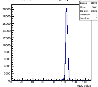
Pedestals mcm172-7417-refv1-g0-s0-p1 ch 5 test1
