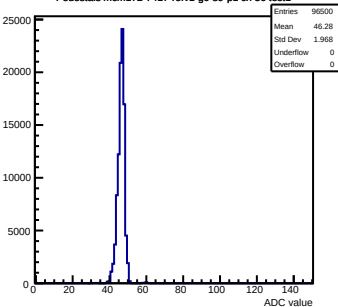
Pedestals mcm172-7417-relv1-g0-s0-p1 ch 56 test1
