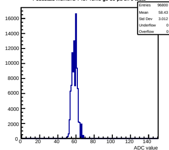
Pedestals mcm172-7417-refv1-g0-s0-p1 ch 6 test1
