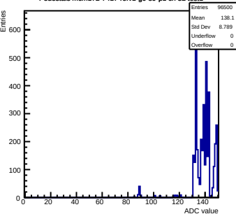
Pedestals mcm172-7417-relv1-g0-s0-p1 ch 52 test1
