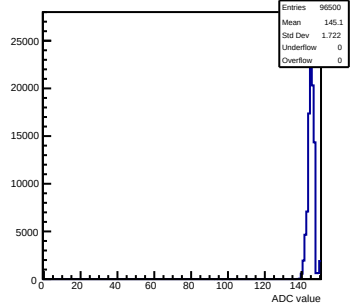
Pedestals mcm172-7417- \text{rev5-g0-s0-p1} ch 61 \text{test1}
