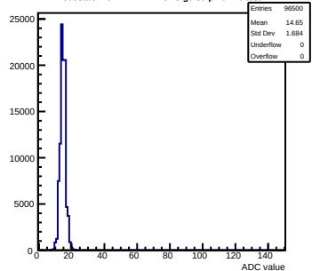
Pedestals mcm172-7417- \text{rev5-g0-s0-p1} ch 49 \text{test1}
