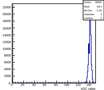
Pedestals mcm172-7417- \text{rev5-g0-s0-p1} ch 54 \text{test1}
