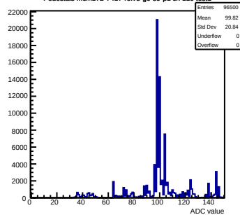
Pedestals mcm172-7417-refv5-g0-s0-p1 ch 119 test1
