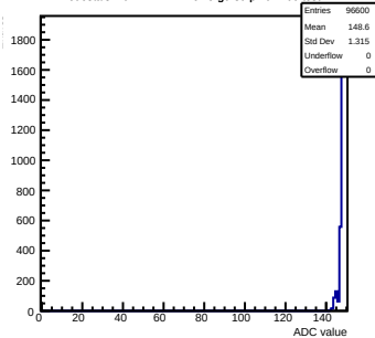
Pedestals mcm172-7417-refv5-g0-s0-p1 ch 100 test1
