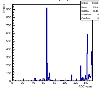
Pedestals mcm172-7417-refv5-g0-s0-p1 ch 127 test1
