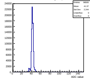
Pedestals mcm172-7417- \text{rev5-g0-s0-p1} ch 56 \text{test1}
