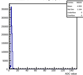
Pedestals mcm172-7417-refv5-g0-s0-p1 ch 120 test1
