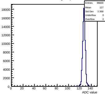
Pedestals mcm172-7417-refv5-g0-s0-p1 ch 108 test1
