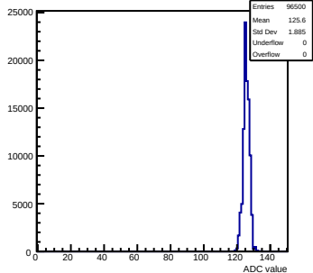
Pedestals mcm172-7417- \text{rev5-g0-s0-p1} ch 62 \text{test1}
