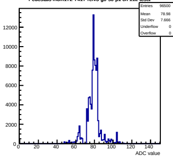
Pedestals mcm172-7417-refv5-g0-s0-p1 ch 112 test1
