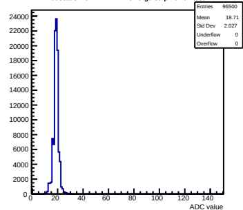
Pedestals mcm172-7417- \text{rev5-g0-s0-p1} ch 51 \text{test1}
