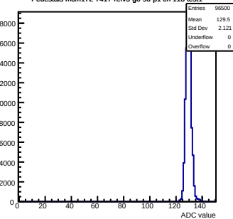
Pedestals mcm172-7417-refv5-g0-s0-p1 ch 113 test1
