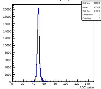
Pedestals mcm172-7417-refv5-g0-s0-p1 ch 126 test1
