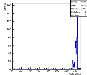
Pedestals mcm172-7417- \text{rev5-g0-s0-p1} ch 52 \text{test1}
