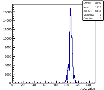
Pedestals mcm172-7417- \text{rev5-g0-s0-p1} ch 57 \text{test1}
