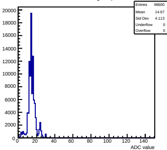
Pedestals mcm172-7417-refv5-g0-s0-p1 ch 104 test1
