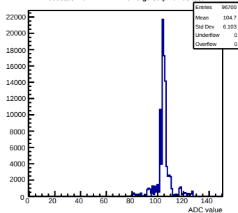
Pedestals mcm172-7417-relv6-g0-s0-p1 ch 93 test1
