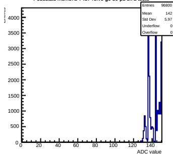
Pedestals mcm172-7417-rlv6-g0-s0-p1 ch 2 test1
