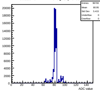
Pedestals mcm172-7417-relv6-g0-s0-p1 ch 90 test1
