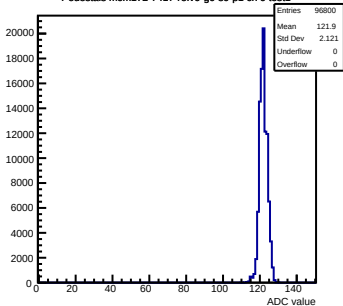
Pedestals mcm172-7417-rlv6-g0-s0-p1 ch 0 test1
