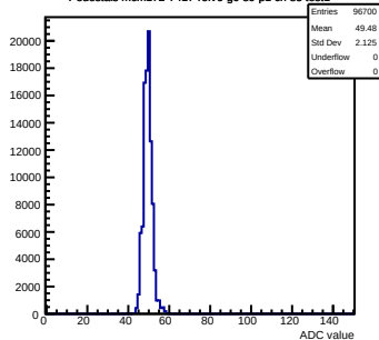
Pedestals mcm172-7417-relv6-g0-s0-p1 ch 85 test1
