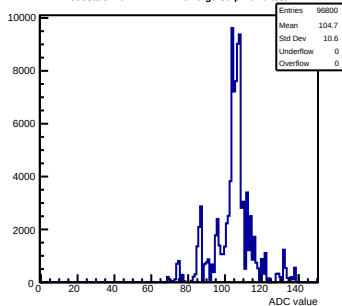
Pedestals mcm172-7417-rlv6-g0-s0-p1 ch 9 test1
