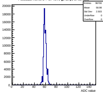
Pedestals mcm172-7417-relv6-g0-s0-p1 ch 86 test1
