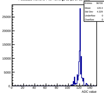
Pedestals mcm172-7417-relv6-g0-s0-p1 ch 82 test1
