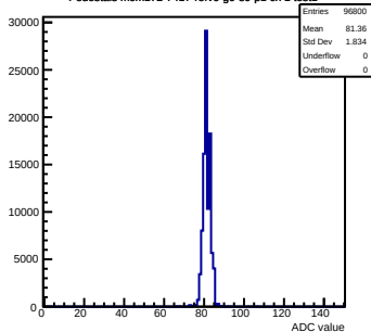
Pedestals mcm172-7417-rlv6-g0-s0-p1 ch 1 test1
