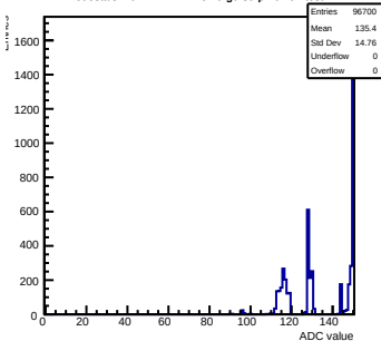
Pedestals mcm172-7417-relv6-g0-s0-p1 ch 94 test1
