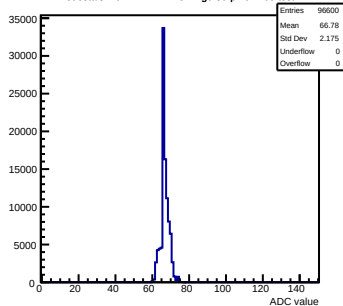
Pedestals mcm172-7417-refv1-g0-s0-p1 ch 105 test1
