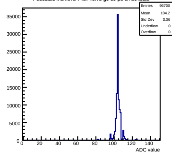
Pedestals mcm172-7417-rlv1-g0-s0-p1 ch 26 test1
