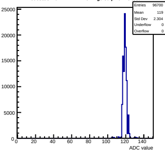
Pedestals mcm172-7417-rlv1-g0-s0-p1 ch 28 test1
