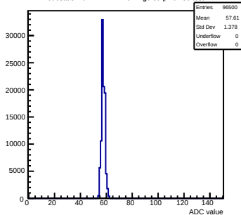
Pedestals mcm172-7417-refv2-g0-s0-p1 ch 56 test1
