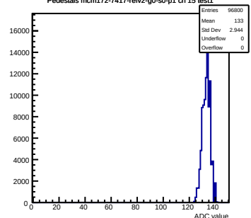
Pedestals mcm172-7417-refv2-g0-s0-p1 ch 15 test1
