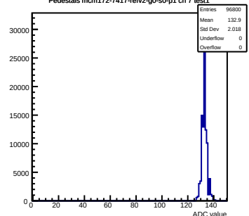
Pedestals mcm172-7417-refv2-g0-s0-p1 ch 7 test1
