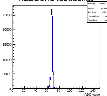
Pedestals mcm172-7417-refv2-g0-s0-p1 ch 34 test1
