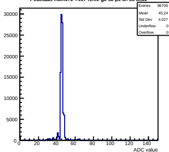
Pedestals mcm172-7417-refv2-g0-s0-p1 ch 86 test1
