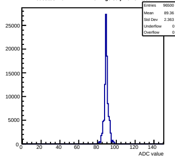
Pedestals mcm172-7417-refv2-g0-s0-p1 ch 57 test1
