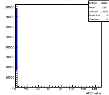
Pedestals mcm172-7417-refv2-g0-s0-p1 ch 76 test1
