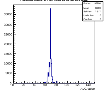
Pedestals mcm172-7417-refv2-g0-s0-p1 ch 3 test1
