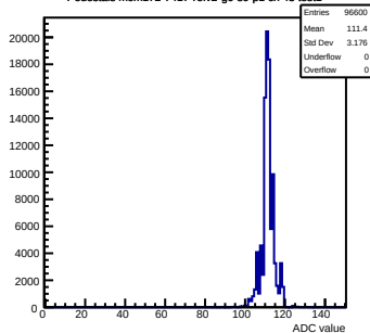
Pedestals mcm172-7417-refv2-g0-s0-p1 ch 43 test1
