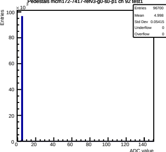
Pedestals mcm172-7417-rev3-g0-s0-p1 ch 92 test1
