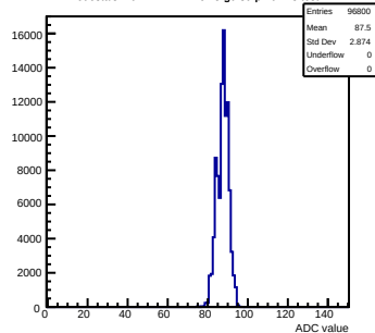
Pedestals mcm172-7417-refv3-g0-s0-p1 ch 13 test1
