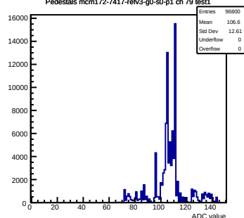
Pedestals mcm172-7417-refv3-g0-s0-p1 ch 79 test1
