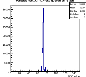
Pedestals mcm172-7417-refv3-g0-s0-p1 ch 78 test1
