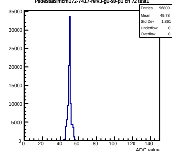
Pedestals mcm172-7417-refv3-g0-s0-p1 ch 72 test1
