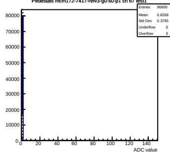
Pedestals mcm172-7417-refv3-g0-s0-p1 ch 67 test1
