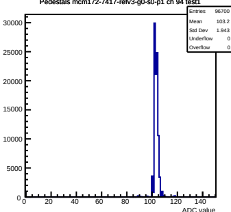
Pedestals mcm172-7417-rev3-g0-s0-p1 ch 94 test1
