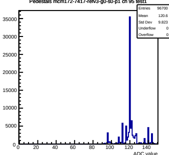
Pedestals mcm172-7417-rev3-g0-s0-p1 ch 95 test1
