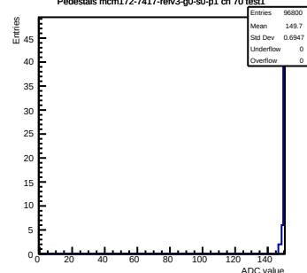
Pedestals mcm172-7417-refv3-g0-s0-p1 ch 70 test1
