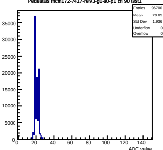
Pedestals mcm172-7417-rev3-g0-s0-p1 ch 90 test1
