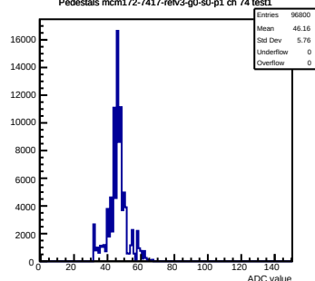
Pedestals mcm172-7417-refv3-g0-s0-p1 ch 74 test1
