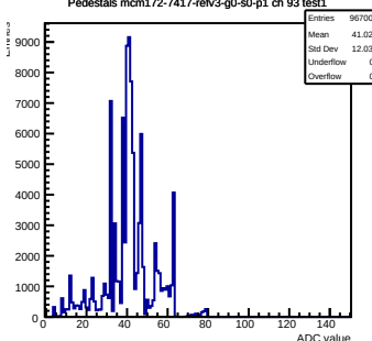
Pedestals mcm172-7417-rev3-g0-s0-p1 ch 93 test1
