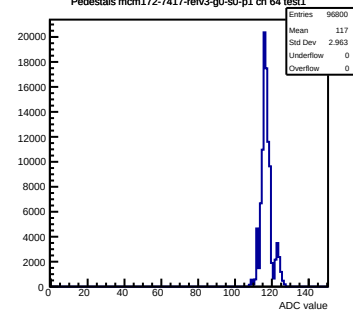
Pedestals mcm172-7417-refv3-g0-s0-p1 ch 64 test1
