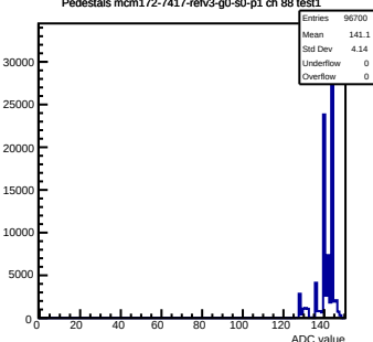
Pedestals mcm172-7417-rev3-g0-s0-p1 ch 88 test1
