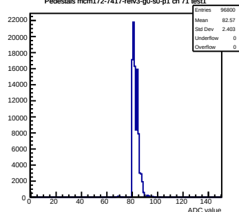
Pedestals mcm172-7417-refv3-g0-s0-p1 ch 71 test1
