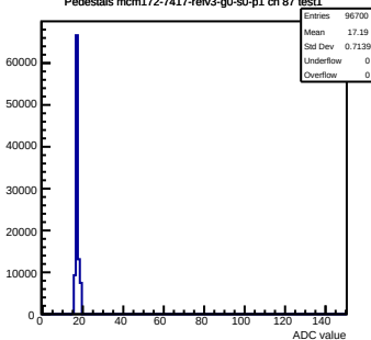
Pedestals mcm172-7417-rev3-g0-s0-p1 ch 87 test1
