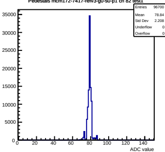
Pedestals mcm172-7417-rev3-g0-s0-p1 ch 82 test1
