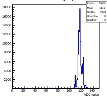
Pedestals mcm172-7417-refv3-g0-s0-p1 ch 10 test1
