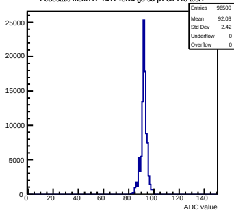
Pedestals mcm172-7417-refv4-g0-s0-p1 ch 113 test1
