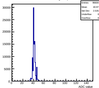
Pedestals mcm172-7417-refv4-g0-s0-p1 ch 110 test1
