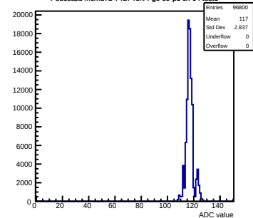
Pedestals mcm172-7417-rlv4-g0-s0-p1 ch 64 test1
