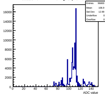
Pedestals mcm172-7417-rlv4-g0-s0-p1 ch 79 test1
