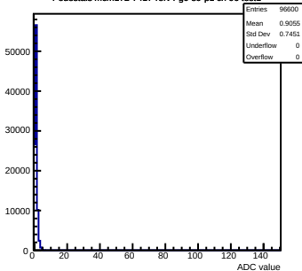
Pedestals mcm172-7417-refv4-g0-s0-p1 ch 96 test1
