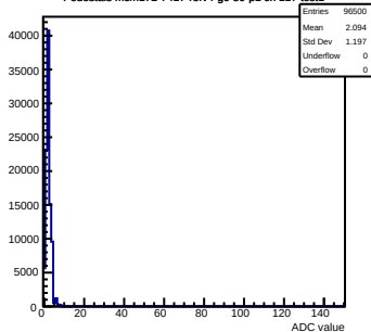
Pedestals mcm172-7417-refv4-g0-s0-p1 ch 117 test1
