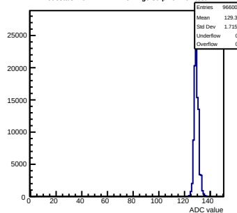
Pedestals mcm172-7417-refv4-g0-s0-p1 ch 107 test1
