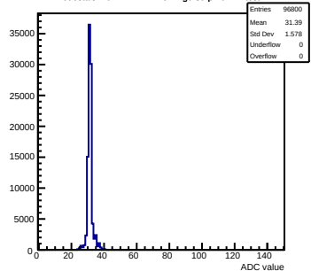
Pedestals mcm172-7417-rlv4-g0-s0-p1 ch 77 test1
