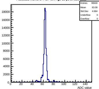
Pedestals mcm172-7417-refv4-g0-s0-p1 ch 116 test1
