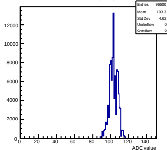
Pedestals mcm172-7417-refv4-g0-s0-p1 ch 109 test1
