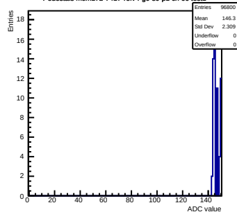
Pedestals mcm172-7417-rlv4-g0-s0-p1 ch 66 test1
