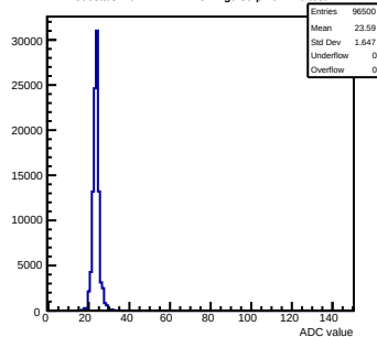
Pedestals mcm172-7417-refv4-g0-s0-p1 ch 126 test1
