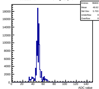
Pedestals mcm172-7417-rlv4-g0-s0-p1 ch 74 test1
