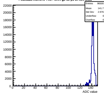
Pedestals mcm172-7417-refv4-g0-s0-p1 ch 114 test1
