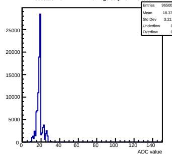
Pedestals mcm172-7417-refv4-g0-s0-p1 ch 123 test1
