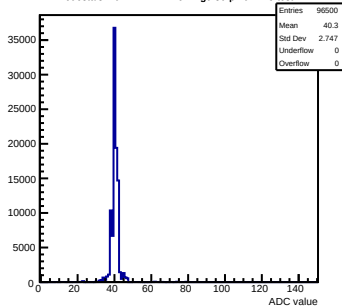
Pedestals mcm172-7417-refv4-g0-s0-p1 ch 125 test1
