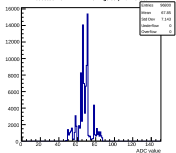
Pedestals mcm172-7417-rlv4-g0-s0-p1 ch 73 test1
