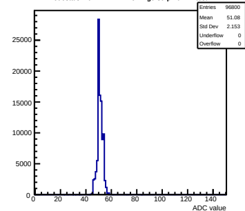
Pedestals mcm172-7417-rlv4-g0-s0-p1 ch 72 test1
