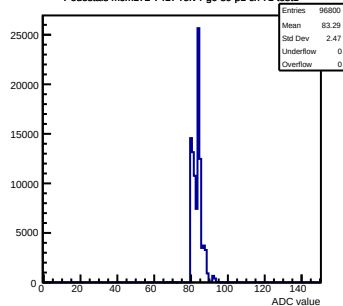
Pedestals mcm172-7417-rlv4-g0-s0-p1 ch 71 test1
