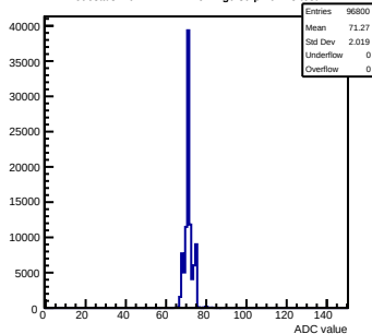
Pedestals mcm172-7417-rlv4-g0-s0-p1 ch 78 test1
