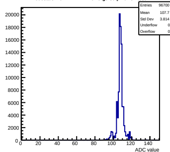
Pedestals mcm172-7417- \text{rev5-g0-s0-p1} ch 31 \text{test1}
