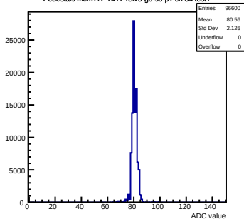
Pedestals mcm172-7417-rev5-g0-s0-p1 ch 34 test1
