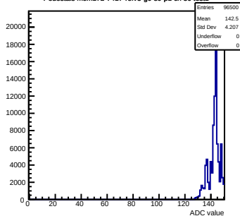
Pedestals mcm172-7417-relv5-g0-s0-p1 ch 50 test1
