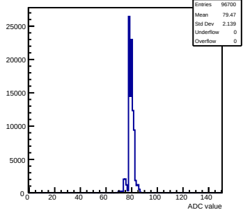
Pedestals mcm172-7417-refv5-g0-s0-p1 ch 93 test1
