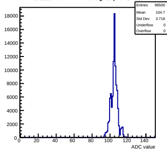
Pedestals mcm172-7417-relv5-g0-s0-p1 ch 57 test1
