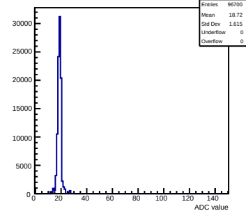
Pedestals mcm172-7417-refv5-g0-s0-p1 ch 92 test1
