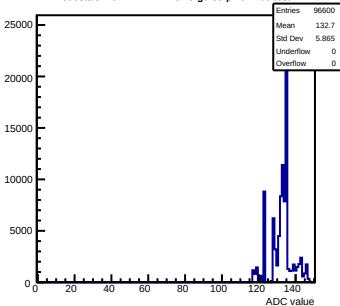
Pedestals mcm172-7417-refV5-g0-s0-p1 ch 106 test1
