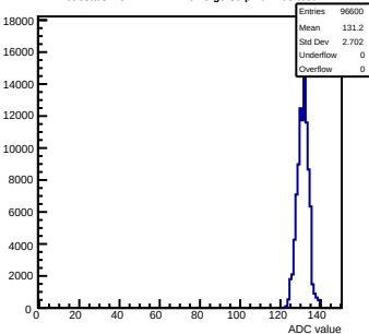
Pedestals mcm172-7417-refV5-g0-s0-p1 ch 108 test1
