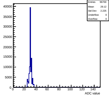
Pedestals mcm172-7417-refv5-g0-s0-p1 ch 87 test1
