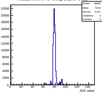
Pedestals mcm172-7417-rev5-g0-s0-p1 ch 40 test1
