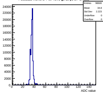
Pedestals mcm172-7417-relv5-g0-s0-p1 ch 49 test1
