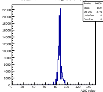
Pedestals mcm172-7417-rev5-g0-s0-p1 ch 45 test1
