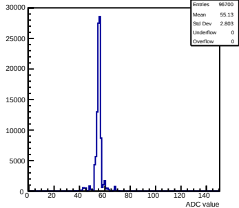
Pedestals mcm172-7417-refv5-g0-s0-p1 ch 86 test1
