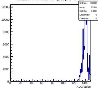
Pedestals mcm172-7417-refV5-g0-s0-p1 ch 101 test1
