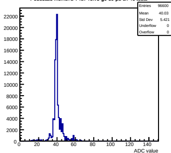
Pedestals mcm172-7417-rev5-g0-s0-p1 ch 46 test1
