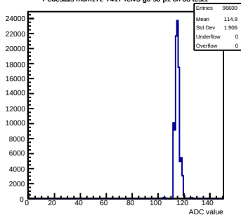
Pedestals mcm172-7417-rev5-g0-s0-p1 ch 33 test1
