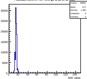
Pedestals mcm172-7417-rev5-g0-s0-p1 ch 32 test1
