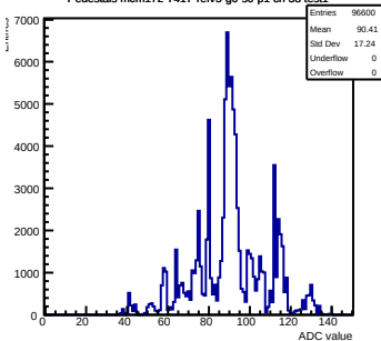
Pedestals mcm172-7417-rev5-g0-s0-p1 ch 38 test1
