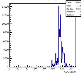
Pedestals mcm172-7417-relv5-g0-s0-p1 ch 62 test1
