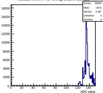
Pedestals mcm172-7417-refV5-g0-s0-p1 ch 103 test1
