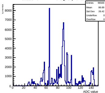
Pedestals mcm172-7417-relv5-g0-s0-p1 ch 55 test1
