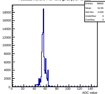
Pedestals mcm172-7417-rev5-g0-s0-p1 ch 41 test1
