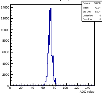
Pedestals mcm172-7417-relv5-g0-s0-p1 ch 56 test1
