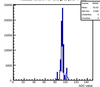
Pedestals mcm172-7417-rev5-g0-s0-p1 ch 47 test1
