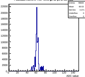
Pedestals mcm172-7417-rev5-g0-s0-p1 ch 36 test1
