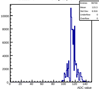
Pedestals mcm172-7417- \text{rev5-g0-s0-p1} ch 28 \text{test1}
