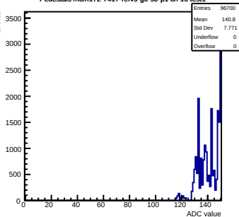
Pedestals mcm172-7417- \text{rev5-g0-s0-p1} ch 16 \text{test1}
