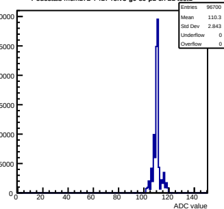
Pedestals mcm172-7417- \text{rev5-g0-s0-p1} ch 21 \text{test1}
