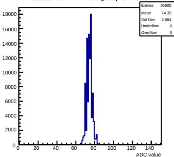
Pedestals mcm172-7417-refV5-g0-s0-p1 ch 110 test1
