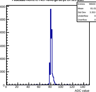
Pedestals mcm172-7417- \text{rfv6-g0-s0-p1} ch 125 test1
