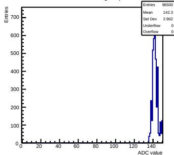
Pedestals mcm172-7417-rlv6-g0-s0-p1 ch 58 test1
