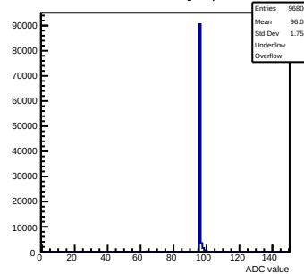
Pedestals mcm172-7417-rlv6-g0-s0-p1 ch 74 test1
