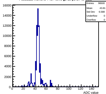
Pedestals mcm172-7417-rlv6-g0-s0-p1 ch 49 test1
