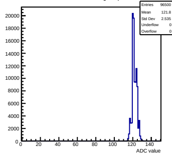
Pedestals mcm172-7417-rlv6-g0-s0-p1 ch 62 test1
