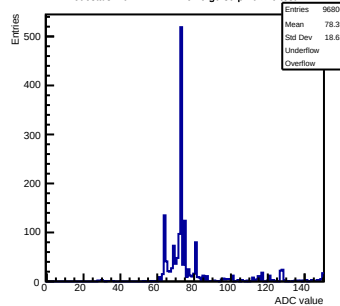
Pedestals mcm172-7417-rlv6-g0-s0-p1 ch 70 test1
