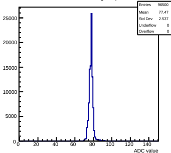
Pedestals mcm172-7417-rlv6-g0-s0-p1 ch 56 test1
