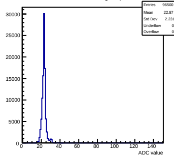
Pedestals mcm172-7417-rlv6-g0-s0-p1 ch 59 test1
