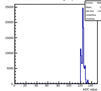
Pedestals mcm172-7417-rlv6-g0-s0-p1 ch 71 test1
