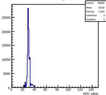
Pedestals mcm172-7417-rlv6-g0-s0-p1 ch 60 test1
