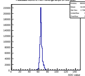
Pedestals mcm172-7417- \text{rfv6-g0-s0-p1} ch 126 test1
