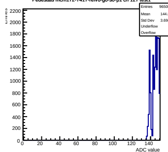
Pedestals mcm172-7417- \text{rfv6-g0-s0-p1} ch 127 test1
