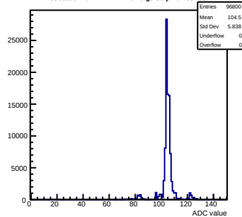
Pedestals mcm172-7417-rlv6-g0-s0-p1 ch 69 test1
