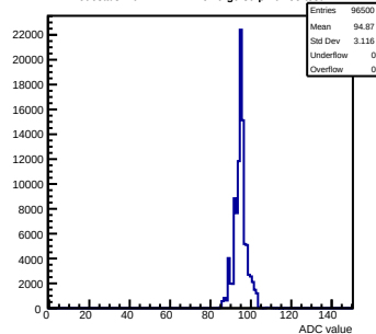
Pedestals mcm172-7417-rlv6-g0-s0-p1 ch 55 test1
