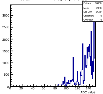
Pedestals mcm172-7417-rlv6-g0-s0-p1 ch 64 test1
