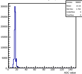
Pedestals mcm172-7417-rlv6-g0-s0-p1 ch 76 test1
