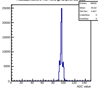
Pedestals mcm172-7417- \text{rfv6-g0-s0-p1} ch 112 test1
