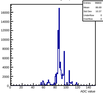
Pedestals mcm172-7417-rlv6-g0-s0-p1 ch 72 test1
