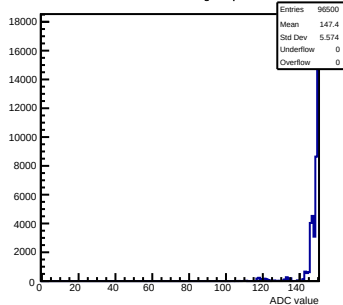
Pedestals mcm172-7417-rlv6-g0-s0-p1 ch 61 test1
