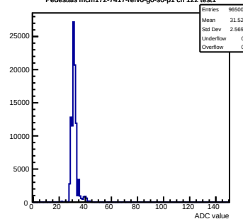
Pedestals mcm172-7417- \text{rfv6-g0-s0-p1} ch 122 test1
