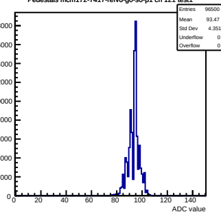
Pedestals mcm172-7417- \text{rfv6-g0-s0-p1} ch 121 test1
