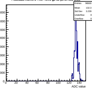
Pedestals mcm172-7417- \text{rfv6-g0-s0-p1} ch 113 test1
