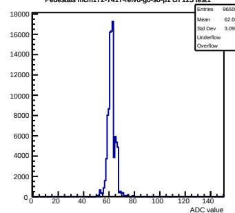
Pedestals mcm172-7417- \text{rfv6-g0-s0-p1} ch 123 test1
