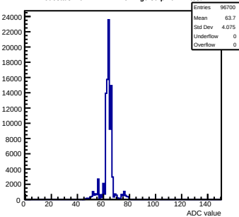
Pedestals mcm172-7417-refv2-g0-s0-p1 ch 24 test1
