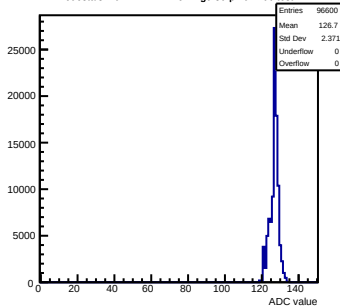
Pedestals mcm172-7417-refv2-g0-s0-p1 ch 106 test1
