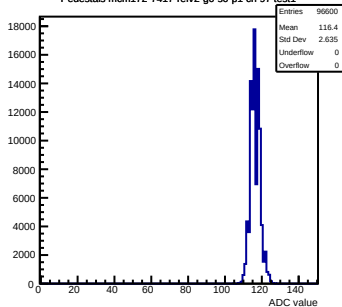
Pedestals mcm172-7417-refv2-g0-s0-p1 ch 97 test1
