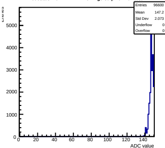
Pedestals mcm172-7417-refv2-g0-s0-p1 ch 107 test1
