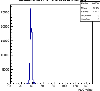
Pedestals mcm172-7417-refv2-g0-s0-p1 ch 96 test1
