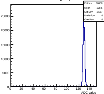
Pedestals mcm172-7417-refv2-g0-s0-p1 ch 108 test1
