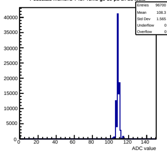
Pedestals mcm172-7417-refv2-g0-s0-p1 ch 21 test1
