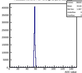
Pedestals mcm172-7417-refv2-g0-s0-p1 ch 102 test1
