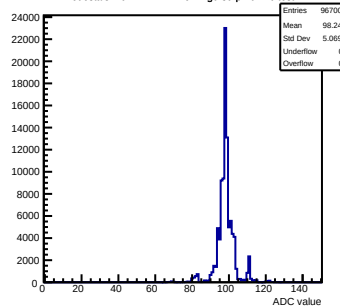
Pedestals mcm172-7417-refv2-g0-s0-p1 ch 26 test1
