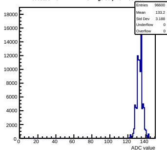
Pedestals mcm172-7417-refv2-g0-s0-p1 ch 109 test1
