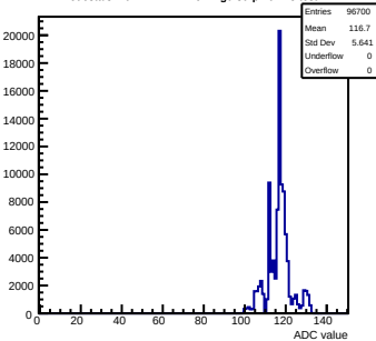
Pedestals mcm172-7417-refv2-g0-s0-p1 ch 28 test1
