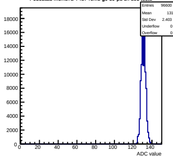
Pedestals mcm172-7417-refv2-g0-s0-p1 ch 103 test1
