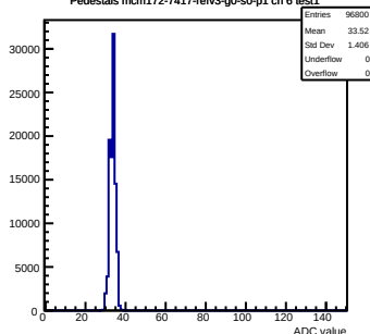
Pedestals mcm172-7417-refv3-g0-s0-p1 ch 6 test1
