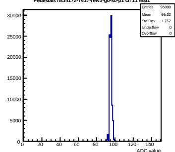
Pedestals mcm172-7417-refv3-g0-s0-p1 ch 11 test1
