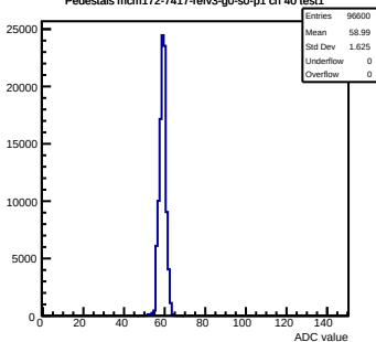
Pedestals mcm172-7417-refv3-g0-s0-p1 ch 40 test1
