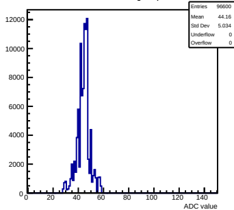
Pedestals mcm172-7417-refv3-g0-s0-p1 ch 105 test1
