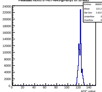
Pedestals mcm172-7417-refv3-g0-s0-p1 ch 10 test1
