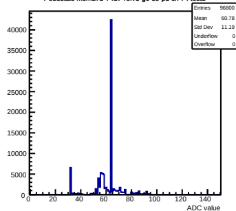
Pedestals mcm172-7417-rev3-g0-s0-p1 ch 74 test1
