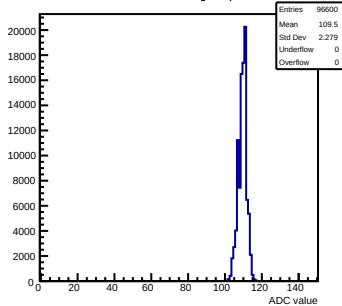
Pedestals mcm172-7417-refv3-g0-s0-p1 ch 109 test1
