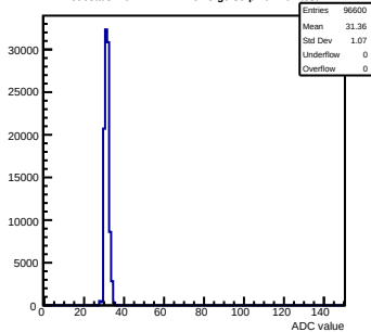
Pedestals mcm172-7417-refv3-g0-s0-p1 ch 102 test1
