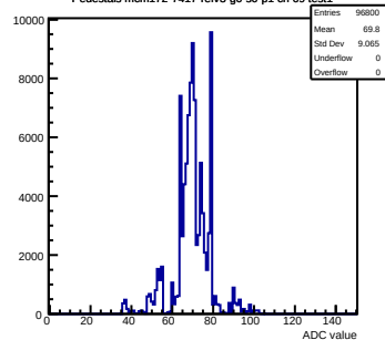
Pedestals mcm172-7417-rev3-g0-s0-p1 ch 69 test1
