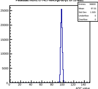
Pedestals mcm172-7417-refv3-g0-s0-p1 ch 13 test1
