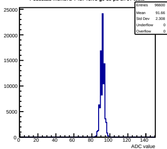
Pedestals mcm172-7417-refv3-g0-s0-p1 ch 97 test1
