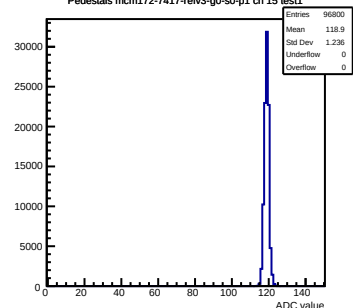
Pedestals mcm172-7417-refv3-g0-s0-p1 ch 15 test1
