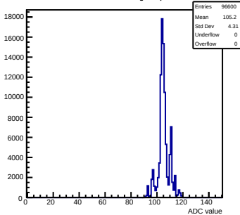
Pedestals mcm172-7417-refv3-g0-s0-p1 ch 108 test1
