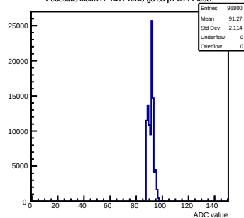
Pedestals mcm172-7417-rev3-g0-s0-p1 ch 71 test1
