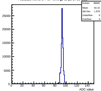
Pedestals mcm172-7417-refv3-g0-s0-p1 ch 98 test1
