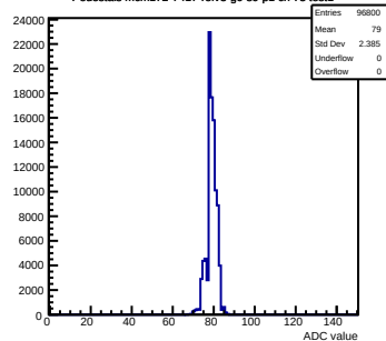
Pedestals mcm172-7417-rev3-g0-s0-p1 ch 73 test1
