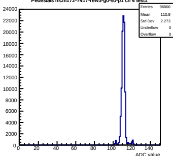
Pedestals mcm172-7417-refv3-g0-s0-p1 ch 4 test1
