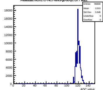
Pedestals mcm172-7417-refv3-g0-s0-p1 ch 7 test1
