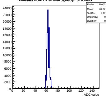
Pedestals mcm172-7417-refv3-g0-s0-p1 ch 45 test1
