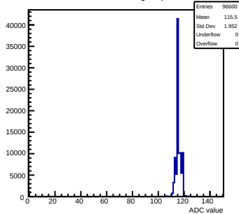
Pedestals mcm172-7417-refv3-g0-s0-p1 ch 111 test1
