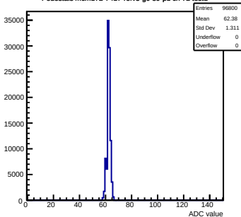
Pedestals mcm172-7417-rev3-g0-s0-p1 ch 72 test1
