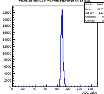
Pedestals mcm172-7417-refv3-g0-s0-p1 ch 33 test1
