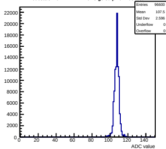
Pedestals mcm172-7417-refv3-g0-s0-p1 ch 103 test1
