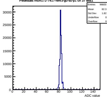
Pedestals mcm172-7417-refv3-g0-s0-p1 ch 37 test1
