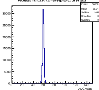
Pedestals mcm172-7417-refv3-g0-s0-p1 ch 34 test1
