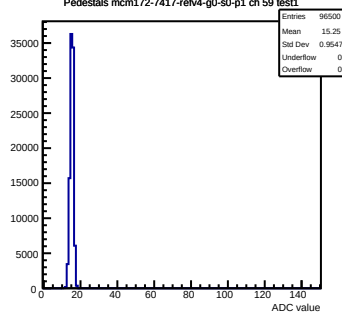
Pedestals mcm172-7417-refv4-g0-s0-p1 ch 59 test1
