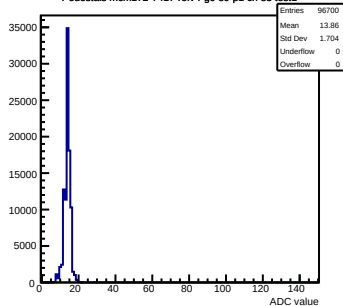
Pedestals mcm172-7417-refv4-g0-s0-p1 ch 85 test1
