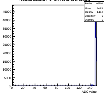
Pedestals mcm172-7417-refv4-g0-s0-p1 ch 81 test1
