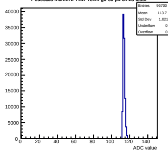
Pedestals mcm172-7417-recv4-g0-s0-p1 ch 23 test1
