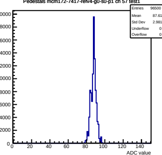
Pedestals mcm172-7417-refv4-g0-s0-p1 ch 57 test1
