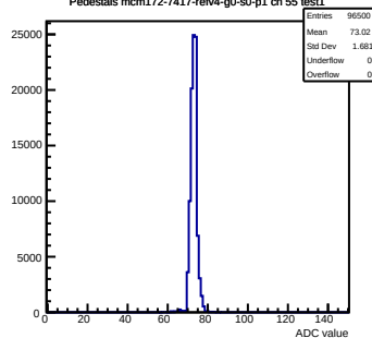
Pedestals mcm172-7417-refv4-g0-s0-p1 ch 55 test1
