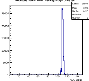
Pedestals mcm172-7417-refv4-g0-s0-p1 ch 48 test1
