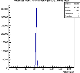
Pedestals mcm172-7417-refv4-g0-s0-p1 ch 56 test1
