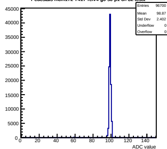
Pedestals mcm172-7417-refv4-g0-s0-p1 ch 82 test1
