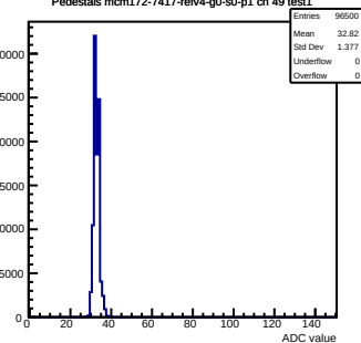
Pedestals mcm172-7417-refv4-g0-s0-p1 ch 49 test1
