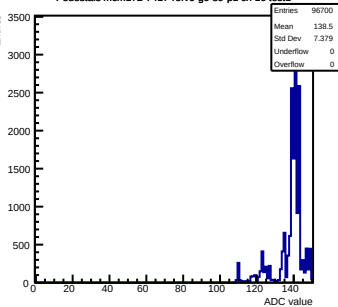
Pedestals mcm172-7417-relv6-g0-s0-p1 ch 16 test1
