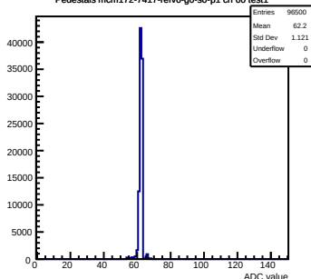
Pedestals mcm172-7417-relv6-g0-s0-p1 ch 60 test1
