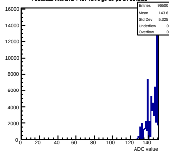
Pedestals mcm172-7417-relv6-g0-s0-p1 ch 53 test1
