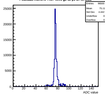
Pedestals mcm172-7417-relv6-g0-s0-p1 ch 49 test1
