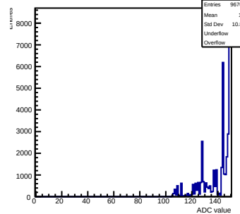
Pedestals mcm172-7417-relv6-g0-s0-p1 ch 23 test1
