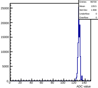
Pedestals mcm172-7417-relv6-g0-s0-p1 ch 20 test1
