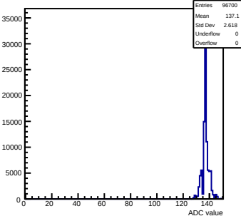
Pedestals mcm172-7417-relv6-g0-s0-p1 ch 28 test1
