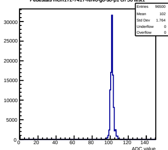
Pedestals mcm172-7417-relv6-g0-s0-p1 ch 56 test1
