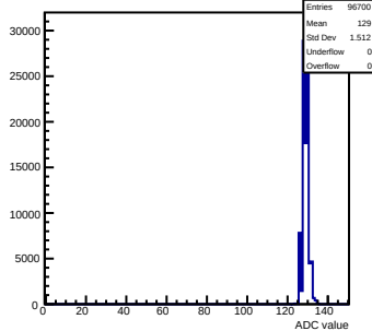
Pedestals mcm172-7417-relv6-g0-s0-p1 ch 21 test1
