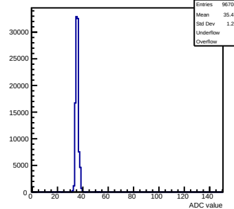
Pedestals mcm172-7417-relv6-g0-s0-p1 ch 22 test1
