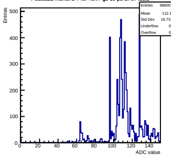
Pedestals mcm172-7417-relv7-g0-s0-p1 ch 97 test1
