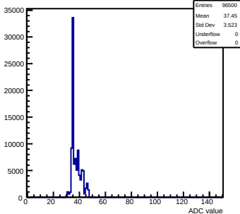
Pedestals mcm172-7417- \text{rev7-g0-s0-p1} ch 120 test1
