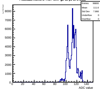
Pedestals mcm172-7417-refv7-g0-s0-p1 ch 5 test1
