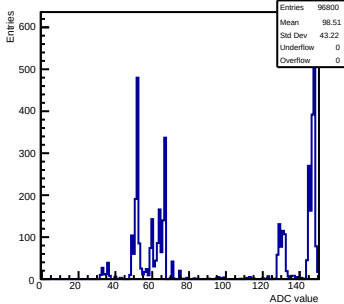
Pedestals mcm172-7417-relv7-g0-s0-p1 ch 78 test1
