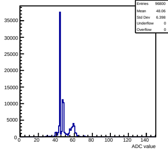
Pedestals mcm172-7417-relv7-g0-s0-p1 ch 77 test1
