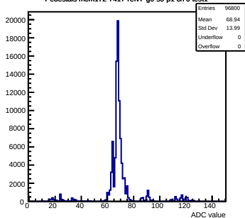
Pedestals mcm172-7417-refv7-g0-s0-p1 ch 0 test1
