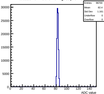
Pedestals mcm173-6E0F-refv1-g0-s0-p1 ch 20 test1
