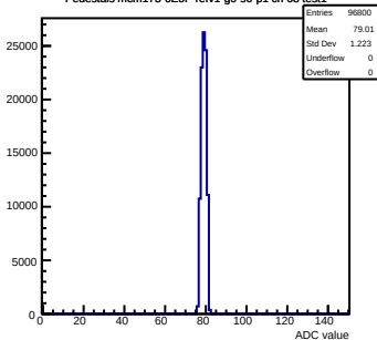
Pedestals mcm173-GEOf-refV1-g0-s0-p1 ch 68 test1
