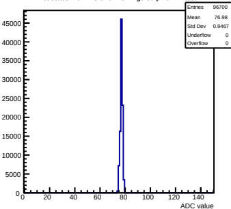
Pedestals mcm173-6E0F-refv1-g0-s0-p1 ch 24 test1
