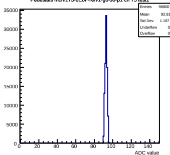
Pedestals mcm173-GEOf-refV1-g0-s0-p1 ch 75 test1
