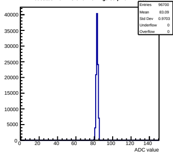
Pedestals mcm173-6E0F-refv1-g0-s0-p1 ch 21 test1
