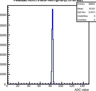
Pedestals mcm173-GEOf-refV1-g0-s0-p1 ch 65 test1
