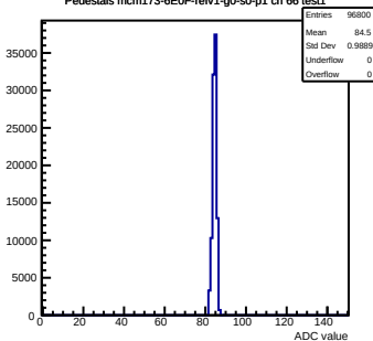
Pedestals mcm173-GEOf-refV1-g0-s0-p1 ch 66 test1
