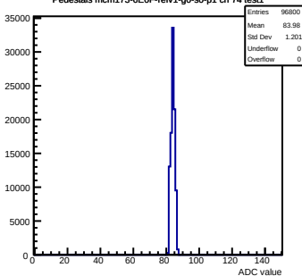
Pedestals mcm173-GEOf-refV1-g0-s0-p1 ch 74 test1
