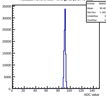
Pedestals mcm173-GEOf-refV1-g0-s0-p1 ch 79 test1
