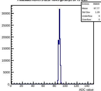
Pedestals mcm173-GEOf-refV1-g0-s0-p1 ch 72 test1
