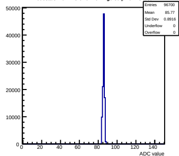
Pedestals mcm173-6E0F-refv1-g0-s0-p1 ch 23 test1
