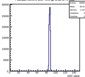
Pedestals mcm173-GEOf-refV1-g0-s0-p1 ch 71 test1
