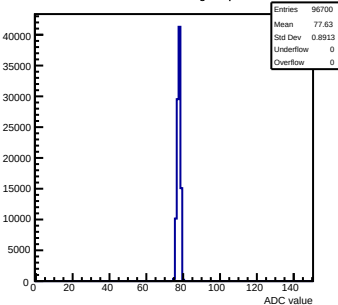
Pedestals mcm173-6E0F-refv1-g0-s0-p1 ch 28 test1
