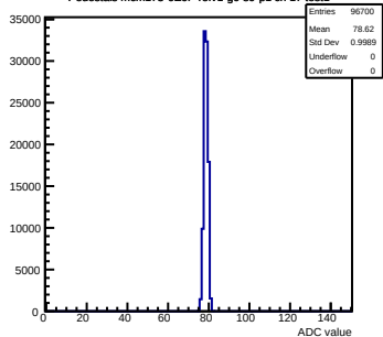
Pedestals mcm173-6E0F-refv1-g0-s0-p1 ch 17 test1
