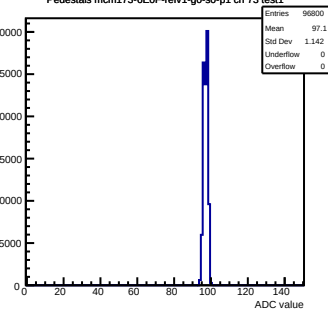
Pedestals mcm173-GEOf-refV1-g0-s0-p1 ch 73 test1
