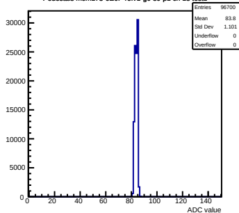
Pedestals mcm173-6E0F-refv1-g0-s0-p1 ch 18 test1
