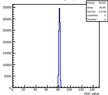
Pedestals mcm173-6E0F-refv1-g0-s0-p1 ch 29 test1
