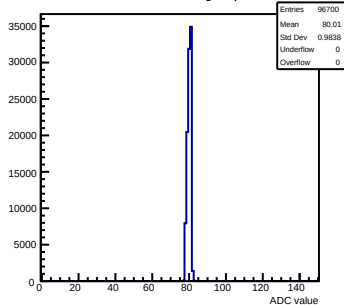
Pedestals mcm173-6E0F-refv1-g0-s0-p1 ch 30 test1
