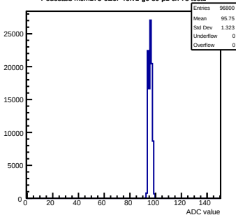
Pedestals mcm173-GEOf-refV1-g0-s0-p1 ch 78 test1
