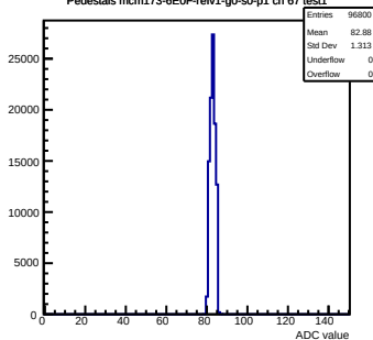
Pedestals mcm173-GEOf-refV1-g0-s0-p1 ch 67 test1
