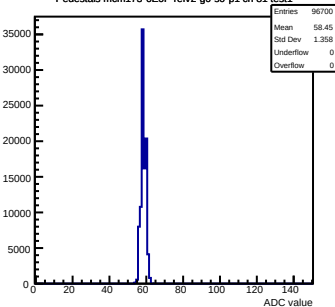
Pedestals mcm173-6E0F-refV2-g0-s0-p1 ch 81 test1
