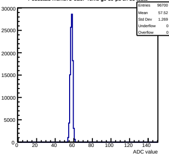
Pedestals mcm173-6E0F-refV2-g0-s0-p1 ch 85 test1
