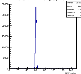
Pedestals mcm173-6E0F-refV2-g0-s0-p1 ch 95 test1
