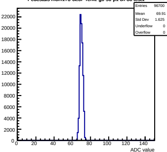
Pedestals mcm173-6E0F-refV2-g0-s0-p1 ch 80 test1
