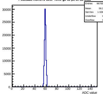
Pedestals mcm173-6E0F-refV2-g0-s0-p1 ch 83 test1
