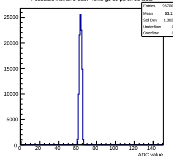
Pedestals mcm173-6E0F-refV2-g0-s0-p1 ch 91 test1
