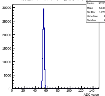
Pedestals mcm173-6E0F-refV2-g0-s0-p1 ch 87 test1
