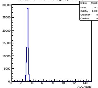
Pedestals mcm173-6E0F-refV3-g0-s0-p1 ch 50 test1
