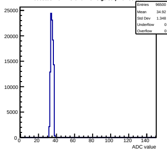
Pedestals mcm173-6E0F-refV3-g0-s0-p1 ch 53 test1
