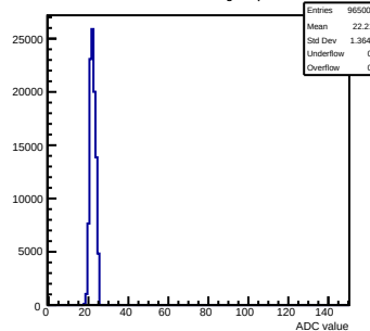
Pedestals mcm173-6E0F-refV3-g0-s0-p1 ch 63 test1
