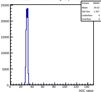
Pedestals mcm173-6E0F-refV3-g0-s0-p1 ch 56 test1
