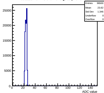
Pedestals mcm173-6E0F-refV3-g0-s0-p1 ch 57 test1
