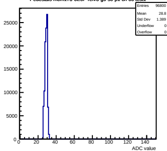
Pedestals mcm173-6E0F-refV3-g0-s0-p1 ch 66 test1
