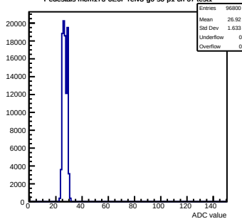
Pedestals mcm173-6E0F-refV3-g0-s0-p1 ch 67 test1
