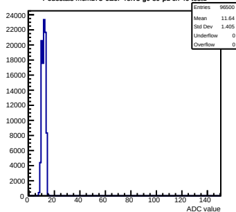
Pedestals mcm173-6E0F-refV3-g0-s0-p1 ch 49 test1
