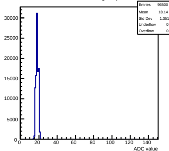
Pedestals mcm173-6E0F-refV3-g0-s0-p1 ch 62 test1
