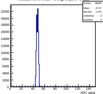
Pedestals mcm173-6E0F-refV3-g0-s0-p1 ch 48 test1
