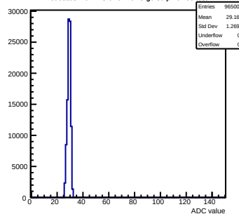
Pedestals mcm173-6E0F-refV3-g0-s0-p1 ch 55 test1
