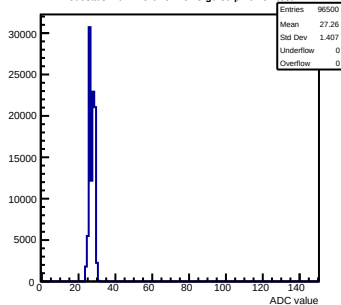
Pedestals mcm173-6E0F-refV3-g0-s0-p1 ch 54 test1
