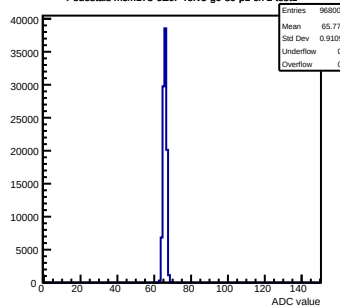
Pedestals mcm173-6E0F-relV5-g0-s0-p1 ch 2 test1
