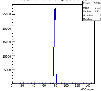
Pedestals mcm173-GEOf-refV5-g0-s0-p1 ch 67 test1
