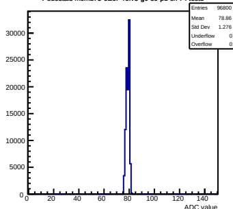
Pedestals mcm173-GEOf-refV5-g0-s0-p1 ch 74 test1
