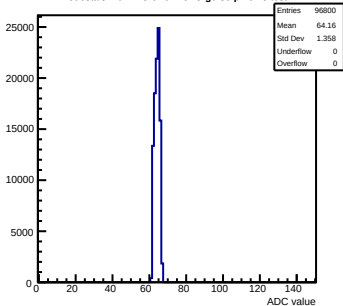
Pedestals mcm173-6E0F-relV5-g0-s0-p1 ch 8 test1
