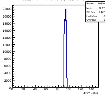
Pedestals mcm173-GEOf-refV5-g0-s0-p1 ch 73 test1
