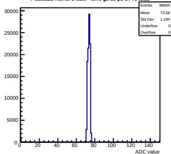
Pedestals mcm173-GEOf-refV5-g0-s0-p1 ch 70 test1
