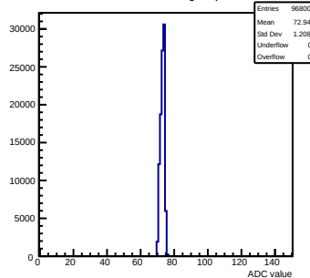
Pedestals mcm173-6E0F-relV5-g0-s0-p1 ch 14 test1
