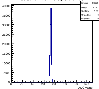
Pedestals mcm173-6E0F-relV5-g0-s0-p1 ch 1 test1
