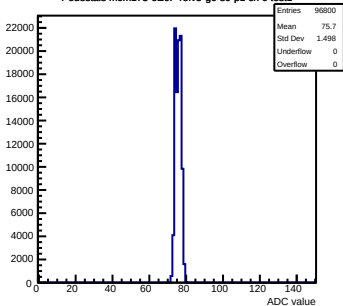
Pedestals mcm173-6E0F-relV5-g0-s0-p1 ch 0 test1
