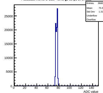
Pedestals mcm173-6E0F-relV5-g0-s0-p1 ch 3 test1
