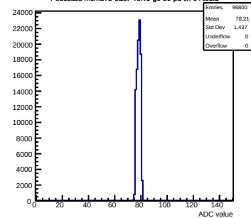
Pedestals mcm173-GEOf-refV5-g0-s0-p1 ch 64 test1
