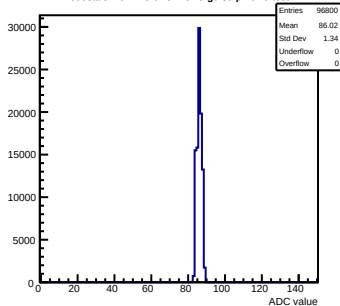
Pedestals mcm173-6E0F-relV5-g0-s0-p1 ch 9 test1
