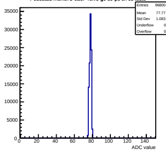
Pedestals mcm173-GEOf-refV5-g0-s0-p1 ch 65 test1
