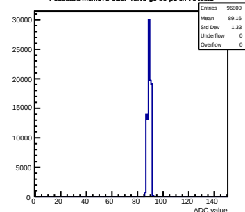
Pedestals mcm173-GEOf-refV5-g0-s0-p1 ch 76 test1
