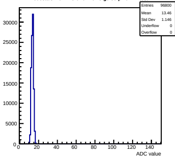
Pedestals mcm173-6E0F-reV3-g0-s0-p1 ch 12 test1
