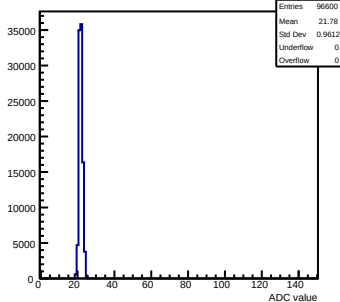
Pedestals mcm173-6E0F-refV3-g0-s0-p1 ch 102 test1
