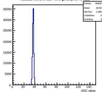
Pedestals mcm173-6E0F-refV3-g0-s0-p1 ch 79 test1
