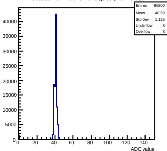
Pedestals mcm173-6E0F-refV3-g0-s0-p1 ch 76 test1
