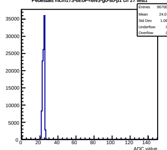
Pedestals mcm173-6E0F-refV3-g0-s0-p1 ch 27 test1
