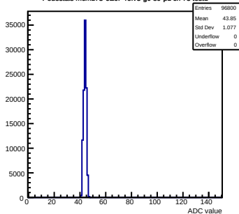
Pedestals mcm173-6E0F-refV3-g0-s0-p1 ch 73 test1
