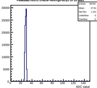
Pedestals mcm173-6E0F-refV3-g0-s0-p1 ch 20 test1
