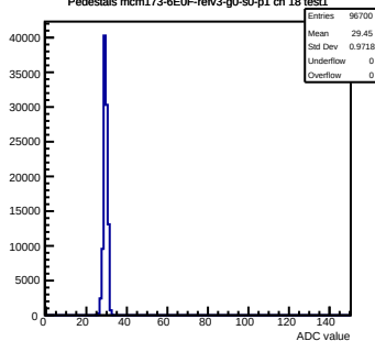
Pedestals mcm173-6E0F-refV3-g0-s0-p1 ch 18 test1
