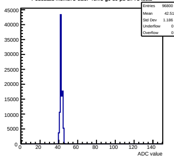
Pedestals mcm173-6E0F-refV3-g0-s0-p1 ch 78 test1
