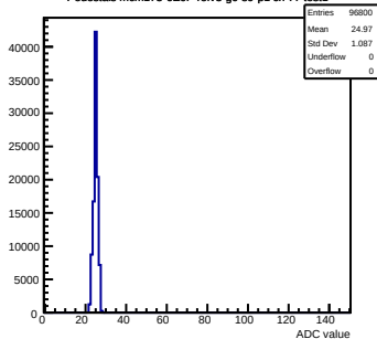
Pedestals mcm173-6E0F-refV3-g0-s0-p1 ch 77 test1
