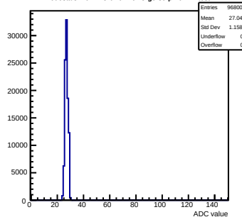
Pedestals mcm173-6E0F-reV3-g0-s0-p1 ch 11 test1
