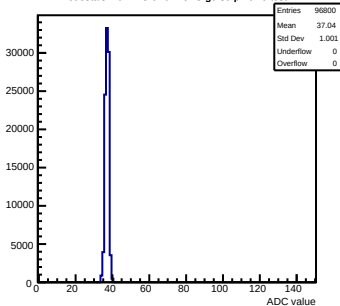
Pedestals mcm173-6E0F-reV3-g0-s0-p1 ch 9 test1
