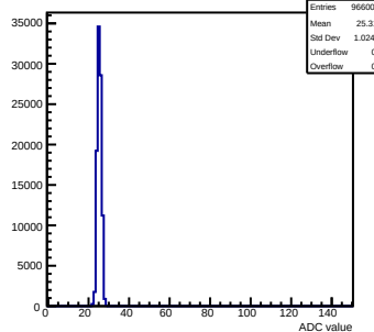
Pedestals mcm173-6E0F-refV3-g0-s0-p1 ch 103 test1
