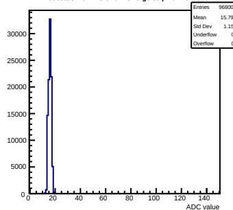
Pedestals mcm173-6E0F-reV3-g0-s0-p1 ch 15 test1
