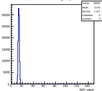
Pedestals mcm173-6E0F-reV3-g0-s0-p1 ch 8 test1
