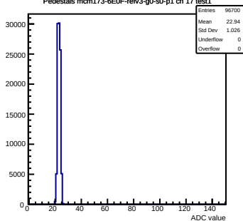
Pedestals mcm173-6E0F-refV3-g0-s0-p1 ch 17 test1
