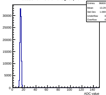
Pedestals mcm173-6E0F-reV3-g0-s0-p1 ch 10 test1
