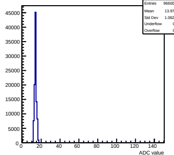
Pedestals mcm173-6E0F-refV3-g0-s0-p1 ch 111 test1
