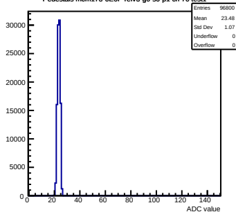
Pedestals mcm173-6E0F-refV3-g0-s0-p1 ch 70 test1
