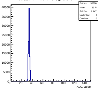
Pedestals mcm173-6E0F-refV3-g0-s0-p1 ch 72 test1
