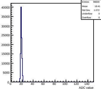
Pedestals mcm173-6E0F-refV3-g0-s0-p1 ch 109 test1
