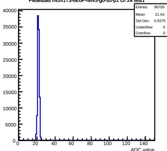
Pedestals mcm173-6E0F-refV3-g0-s0-p1 ch 24 test1
