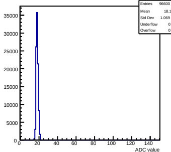
Pedestals mcm173-6E0F-refV3-g0-s0-p1 ch 106 test1
