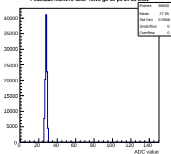
Pedestals mcm173-6E0F-refV3-g0-s0-p1 ch 65 test1
