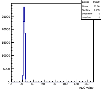
Pedestals mcm173-6E0F-refV3-g0-s0-p1 ch 108 test1
