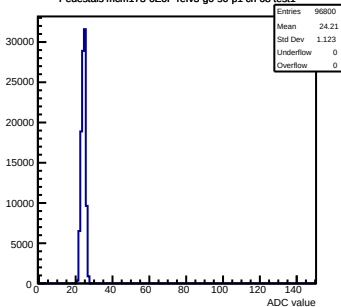
Pedestals mcm173-6E0F-refV3-g0-s0-p1 ch 68 test1
