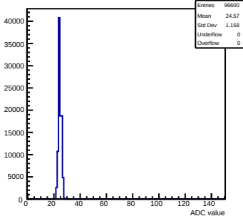
Pedestals mcm173-6E0F-refV3-g0-s0-p1 ch 104 test1
