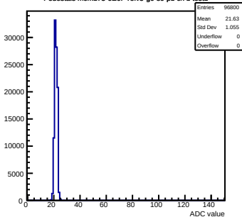
Pedestals mcm173-6E0F-reV3-g0-s0-p1 ch 1 test1
