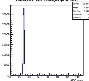
Pedestals mcm173-6E0F-refV3-g0-s0-p1 ch 26 test1
