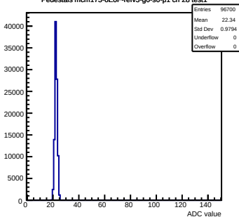
Pedestals mcm173-6E0F-refV3-g0-s0-p1 ch 28 test1
