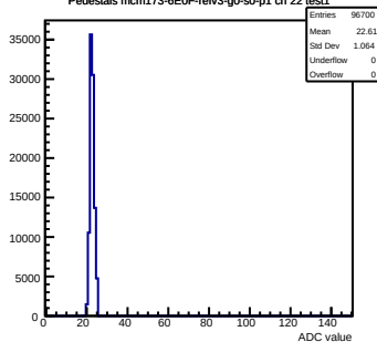
Pedestals mcm173-6E0F-refV3-g0-s0-p1 ch 22 test1
