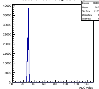
Pedestals mcm173-6E0F-reV3-g0-s0-p1 ch 7 test1
