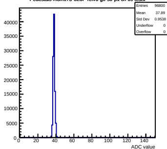
Pedestals mcm173-6E0F-refV3-g0-s0-p1 ch 69 test1
