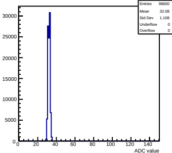
Pedestals mcm173-6E0F-refV3-g0-s0-p1 ch 105 test1
