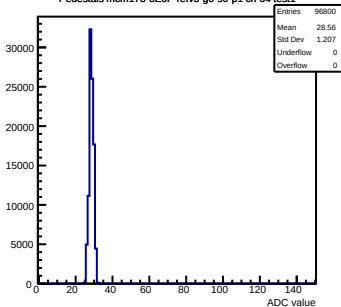
Pedestals mcm173-6E0F-refV3-g0-s0-p1 ch 64 test1
