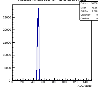
Pedestals mcm173-GE0F-refv4-g0-s0-p1 ch 34 test1
