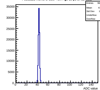
Pedestals mcm173-6E0F-refv4-g0-s0-p1 ch 83 test1
