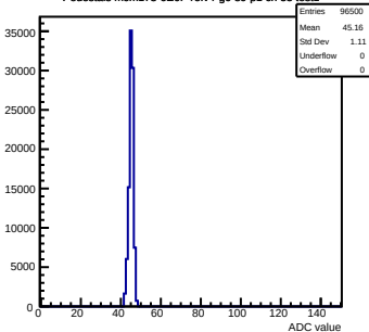
Pedestals mcm173-GE0F-refV4-g0-s0-p1 ch 55 test1
