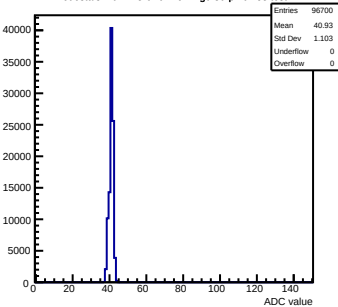
Pedestals mcm173-6E0F-refv4-g0-s0-p1 ch 88 test1
