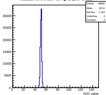
Pedestals mcm173-GE0F-refv4-g0-s0-p1 ch 41 test1
