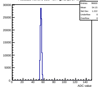
Pedestals mcm173-GE0F-refv4-g0-s0-p1 ch 46 test1
