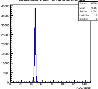
Pedestals mcm173-GE0F-refV4-g0-s0-p1 ch 50 test1
