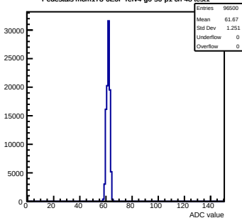
Pedestals mcm173-GE0F-refV4-g0-s0-p1 ch 48 test1
