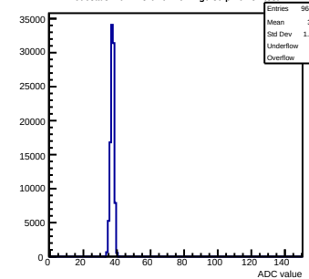
Pedestals mcm173-6E0F-refv4-g0-s0-p1 ch 87 test1
