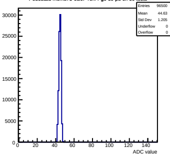
Pedestals mcm173-GE0F-refV4-g0-s0-p1 ch 59 test1
