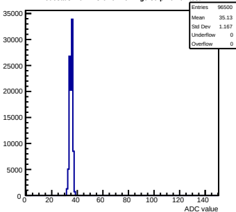
Pedestals mcm173-GE0F-refV4-g0-s0-p1 ch 62 test1
