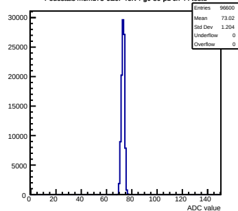
Pedestals mcm173-GE0F-refv4-g0-s0-p1 ch 44 test1
