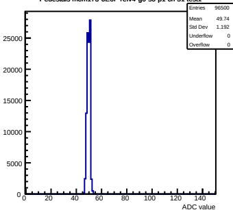
Pedestals mcm173-GE0F-refV4-g0-s0-p1 ch 51 test1
