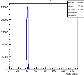
Pedestals mcm173-GE0F-refV4-g0-s0-p1 ch 63 test1
