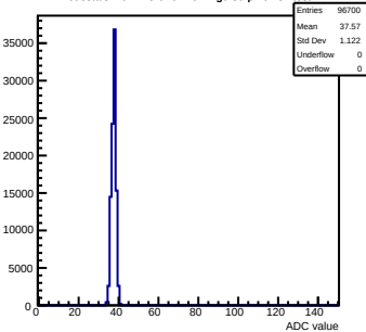
Pedestals mcm173-6E0F-refv4-g0-s0-p1 ch 84 test1
