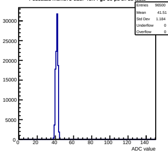
Pedestals mcm173-GE0F-refV4-g0-s0-p1 ch 52 test1
