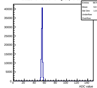
Pedestals mcm173-6E0F-refv4-g0-s0-p1 ch 86 test1
