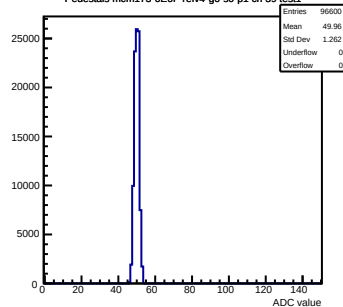
Pedestals mcm173-GE0F-refv4-g0-s0-p1 ch 39 test1
