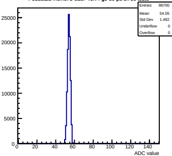
Pedestals mcm173-6E0F-refv4-g0-s0-p1 ch 80 test1
