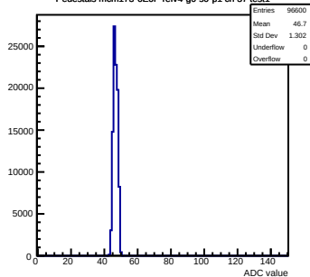
Pedestals mcm173-GE0F-refv4-g0-s0-p1 ch 37 test1
