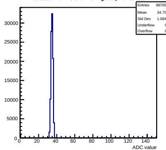
Pedestals mcm173-6E0F-refv4-g0-s0-p1 ch 89 test1
