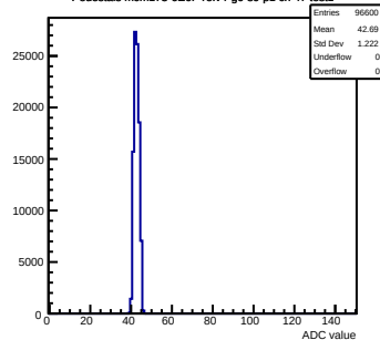
Pedestals mcm173-GE0F-refv4-g0-s0-p1 ch 47 test1
