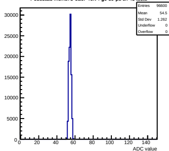
Pedestals mcm173-GE0F-refv4-g0-s0-p1 ch 45 test1
