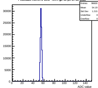
Pedestals mcm173-GE0F-refv4-g0-s0-p1 ch 38 test1
