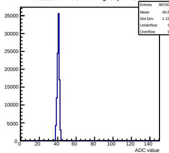
Pedestals mcm173-6E0F-refv4-g0-s0-p1 ch 85 test1
