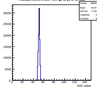
Pedestals mcm173-GE0F-refv4-g0-s0-p1 ch 35 test1
