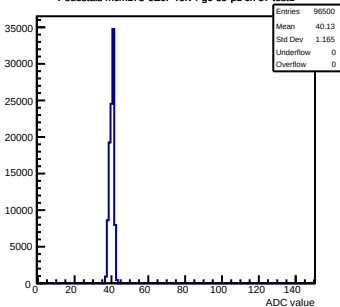
Pedestals mcm173-GE0F-refV4-g0-s0-p1 ch 57 test1
