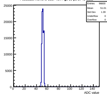
Pedestals mcm173-GE0F-refv4-g0-s0-p1 ch 40 test1
