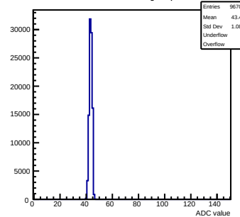
Pedestals mcm173-6E0F-refv4-g0-s0-p1 ch 94 test1
