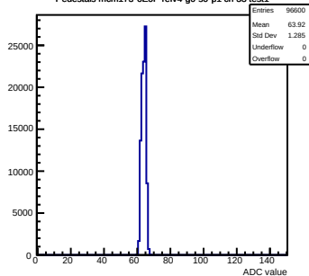
Pedestals mcm173-GE0F-refv4-g0-s0-p1 ch 33 test1
