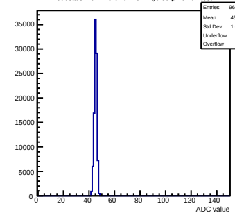
Pedestals mcm173-6E0F-refv4-g0-s0-p1 ch 91 test1
