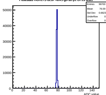
Pedestals mcm173-GEOf-refV5-g0-s0-p1 ch 29 test1
