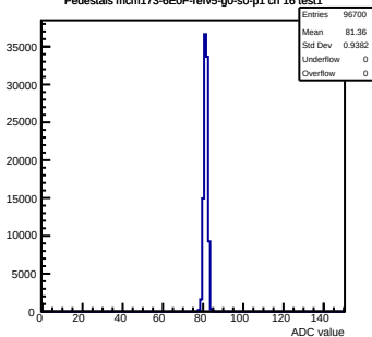
Pedestals mcm173-GEOf-refV5-g0-s0-p1 ch 16 test1
