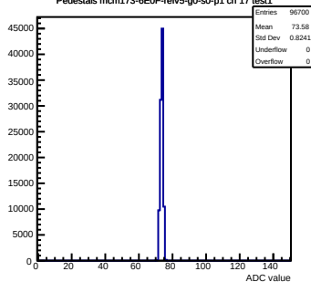
Pedestals mcm173-GEOf-refV5-g0-s0-p1 ch 17 test1
