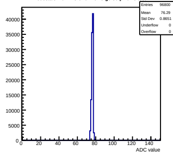
Pedestals mcm173-6E0F-reV5-g0-s0-p1 ch 3 test1
