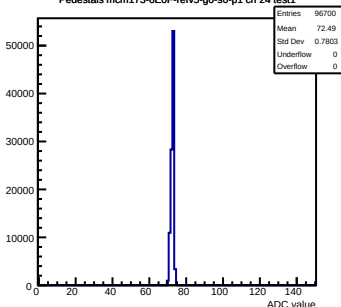
Pedestals mcm173-GEOf-refV5-g0-s0-p1 ch 24 test1
