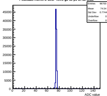
Pedestals mcm173-6E0F-refV5-g0-s0-p1 ch 82 test1
