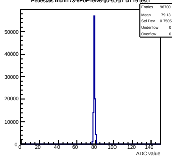
Pedestals mcm173-GEOf-refV5-g0-s0-p1 ch 19 test1
