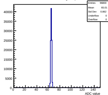
Pedestals mcm173-6E0F-reV5-g0-s0-p1 ch 8 test1
