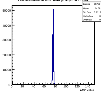
Pedestals mcm173-GEOf-refV5-g0-s0-p1 ch 27 test1
