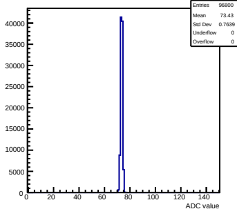
Pedestals mcm173-6E0F-reV5-g0-s0-p1 ch 14 test1
