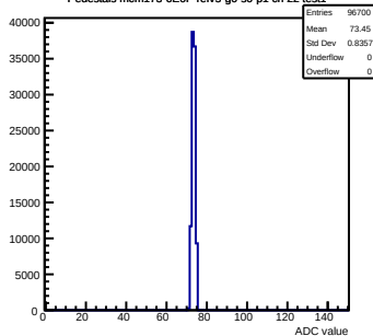
Pedestals mcm173-GEOf-refV5-g0-s0-p1 ch 22 test1
