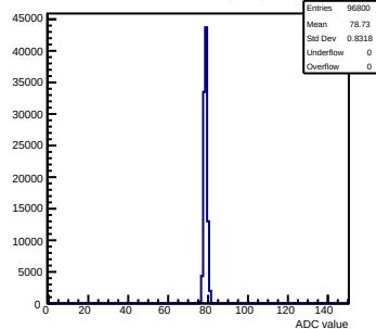
Pedestals mcm173-6E0F-reV5-g0-s0-p1 ch 7 test1
