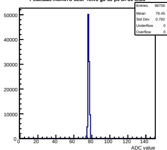
Pedestals mcm173-6E0F-refV5-g0-s0-p1 ch 81 test1
