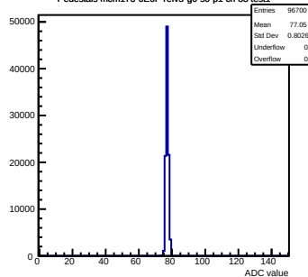
Pedestals mcm173-6E0F-refV5-g0-s0-p1 ch 83 test1
