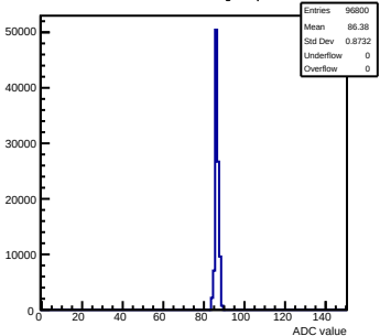
Pedestals mcm173-6E0F-reV5-g0-s0-p1 ch 9 test1
