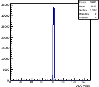
Pedestals mcm173-6E0F-reV5-g0-s0-p1 ch 5 test1
