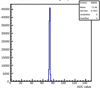
Pedestals mcm173-6E0F-reV5-g0-s0-p1 ch 1 test1
