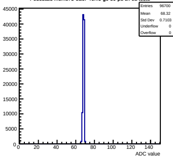
Pedestals mcm173-6E0F-refV5-g0-s0-p1 ch 92 test1
