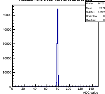
Pedestals mcm173-GEOf-refV5-g0-s0-p1 ch 21 test1
