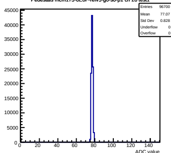
Pedestals mcm173-GEOf-refV5-g0-s0-p1 ch 26 test1
