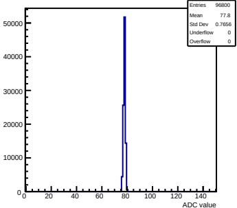
Pedestals mcm173-6E0F-reV5-g0-s0-p1 ch 13 test1
