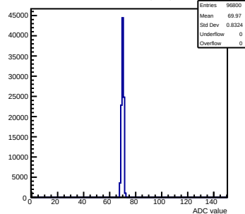
Pedestals mcm173-6E0F-reV5-g0-s0-p1 ch 4 test1
